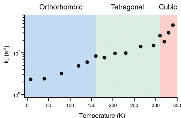
Figure 2. The temperature dependence of the monomolecular recombination rate, k_1 . Values are provided in Table S1 (Supporting Information).
