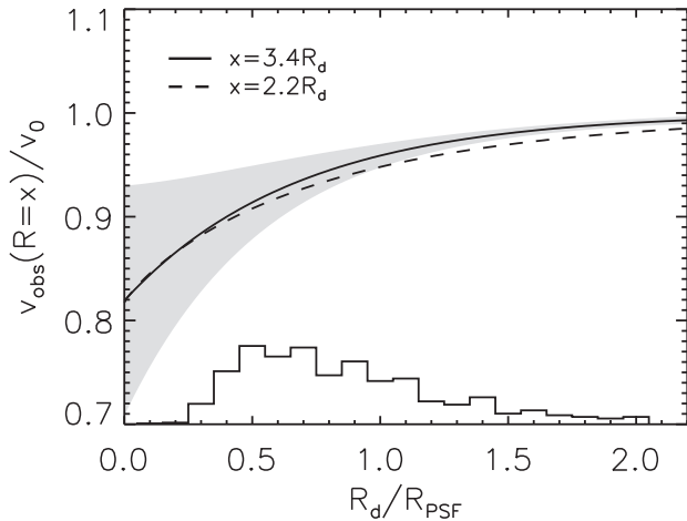
Figure 3. Beam smearing correction applied to measurements of the rotation velocity at radii of 3.4R_d and 2.2R_d ( v_C and v_{2.2} , respectively), as a function of R_d/R_{\text{PSF}} . The shaded region represents the 1\sigma scatter of outcomes for \sim 10^5 mock galaxies. Tracks show the median of these outcomes and are defined by equation (B6) and the parameters listed in Table B1. The histogram represents the R_d/R_{\text{PSF}} distribution of the KROSS sample. Applying these beam smearing corrections to our data, we find a modest median velocity correction of \xi_v = 1.07 \pm 0.03 and range of \xi_v = 1.0 – 1.17 .
