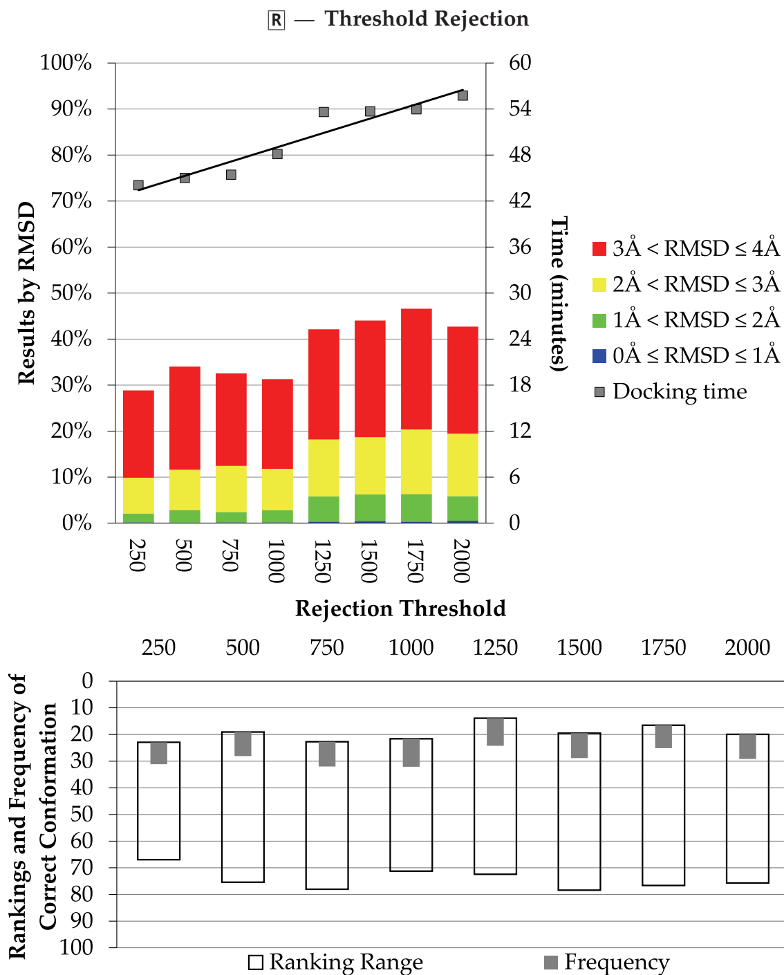
Figure 6.7: Effect of early rejection using scoring thresholds on docking time and results, showing improved accuracy and longer time at larger thresholds
