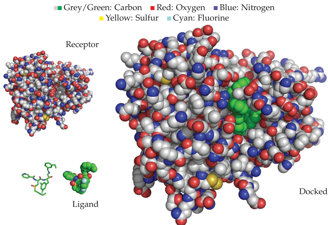
Figure 1.1: The human recombinant beta-secretase protein with a ligand proposed as a treatment for Alzheimer's disease (PDB code 2HM1)
