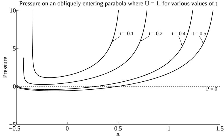
Figure 4. The pressure on a parabolic impactor for various times with U = 1 . The critical time at which the trailing turnover point stops advancing is given by t = 1/2 . It is clear that the pressure vanishes at d_- = -1/2 when t reaches this critical value.
