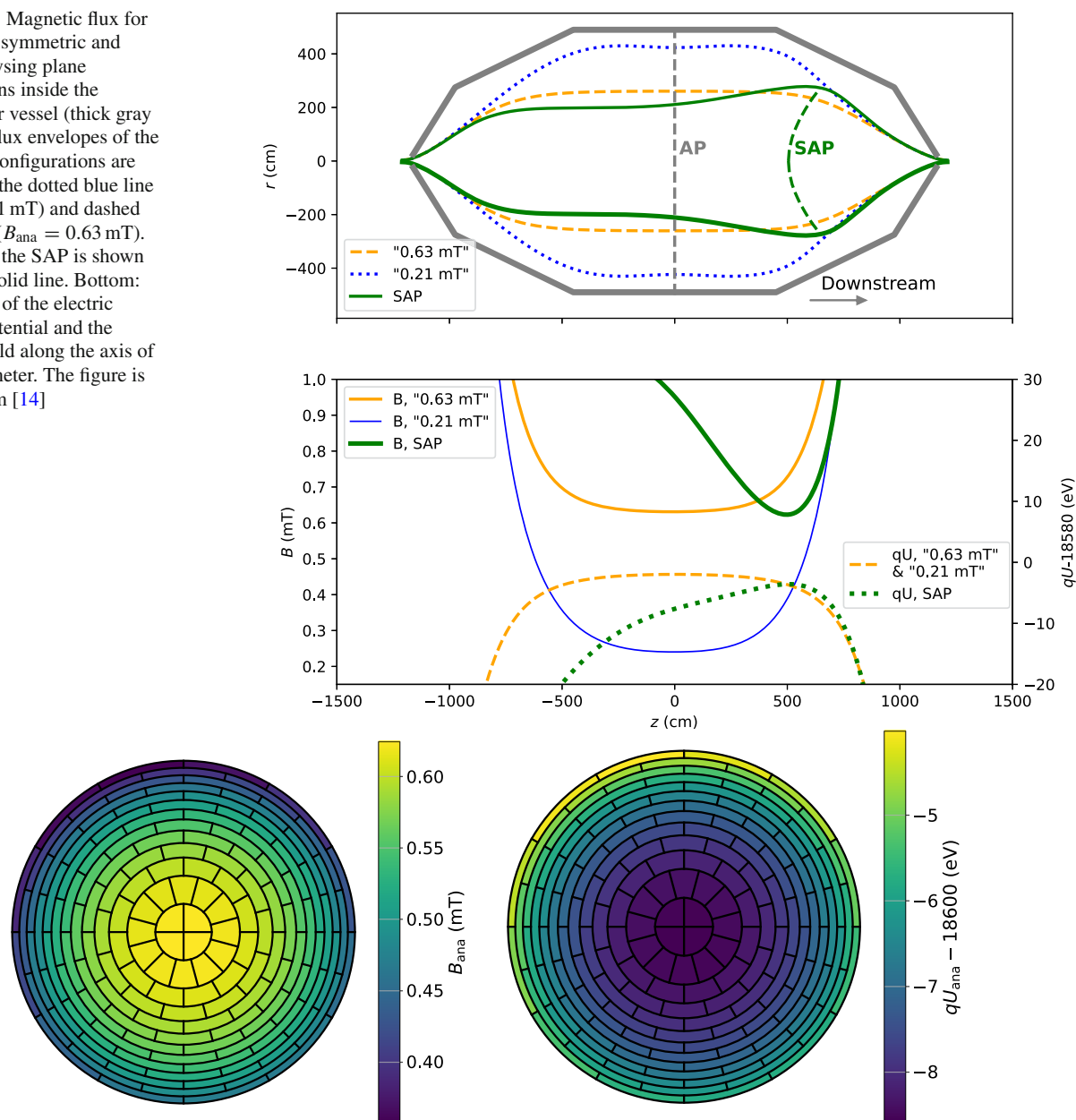
Fig. 4 An image of the magnetic field (left) and the electric retarding potential (right) of the SAP configuration on the detector pixels. The magnetic field in the analysing plane is estimated for the electrons arriving at the center of each pixel via a full simulation of electromagnetic fields in the main spectrometer. A typical variation of 0.2 mT for the SAP mode is significantly larger than the magnetic-field variation
