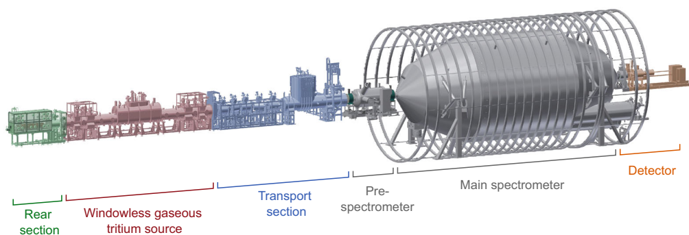
Fig. 1 Overview of the KATRIN experimental setup. The rear section contains the monitoring and calibration instruments, including the photoelectron source. Windowless gaseous tritium source provides up to 100 GBq of activity. The emitted electrons follow the magnetic field
