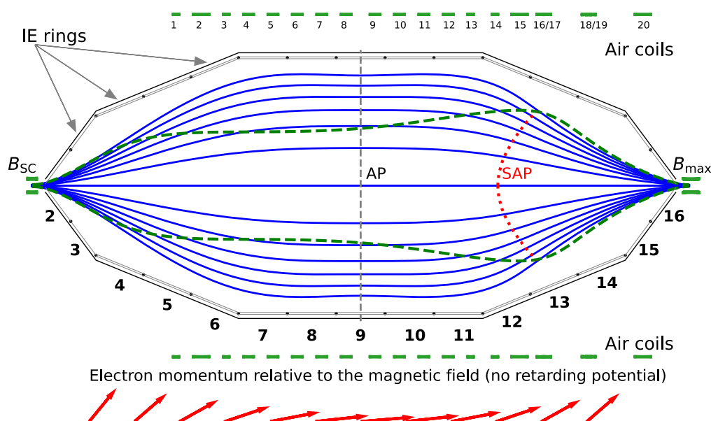
Fig. 2 The MAC-E-filter principle of the KATRIN main spectrometer. Electrons, emitted in the tritium source in the field B_S , enter the spectrometer from the left. The solid blue lines indicate the magnetic field lines inside the spectrometer. The magnetic field is produced by the superconducting (SC) solenoids ( B_{SC} and B_{max} ) and 20 air coils. The electric retarding potential is generated by the voltage applied to the spectrometer vessel (solid dark gray line) and the inner electrode
