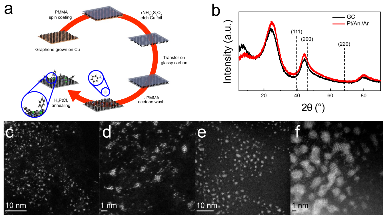
Figure 1. (a) Schematic illustration of the synthesis process (5 steps) for Pt SSC (gray, Pt; green, Cl; blue, N; black, carbon; white, H). Step 1: graphene nanosheets are grown by chemical vapor deposition (CVD) on copper. Step 2: copper foil is etched after spin coating with poly(methyl methacrylate) (PMMA) on top. Step 3: Thin-layer graphene coated with PMMA is then transferred onto a polished glassy carbon (GC) electrode. Step 4: after washing the PMMA with acetone and heating to 250^\circ\text{C} to remove trace organic contaminants, aniline is drop cast onto the graphene-coated GC electrode and dried. Step 5: chloroplatinic acid in ethanol is then drop cast and annealed under an argon atmosphere. This sample is referred to as the (Pt/Ani/Ar) sample. Control sample (Pt/Ar) is prepared by the same method but without aniline. (b) X-ray diffraction patterns for pristine GC and a (Pt/Ani/Ar) sample on GC; low-magnification to high-magnification atomic resolution HAADF-STEM images of (Pt/Ani/Ar) (c, d) and (Pt/Ar) (e, f).
