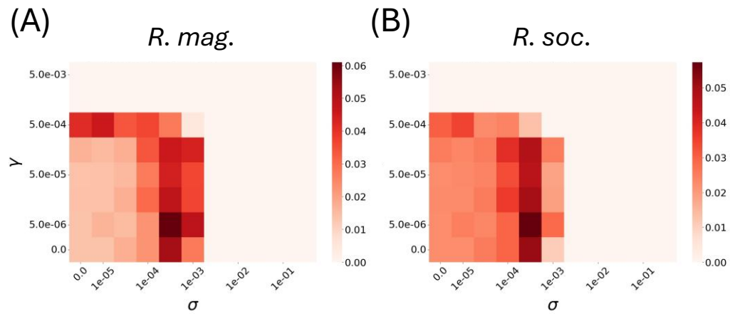
Fig. S4. Euclidean distance of observed tree composition ( p(CL) , p(AR) and p(SX) ) from that across the simulated (Pieszko et al., 2025) space of the sex rate \sigma and the LOH rate \gamma (optimised mutation rates; \beta = 0.05 ). Distances < 0.8 were truncated, and the remaining distances were normalised. (A) R. magnacalcarata . (B) R. socialis .
