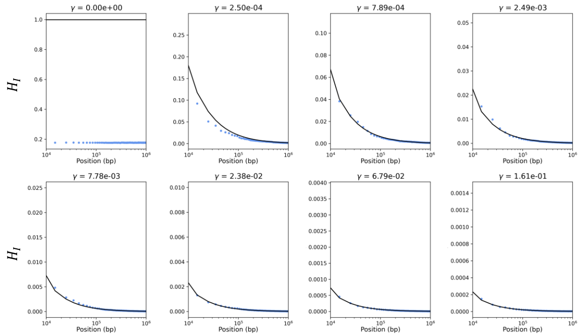
Fig. S16. H_I after 200,000 simulated generations of obligate central fusion (CF) (blue dots) compared to the analytical predictions of Engelstädter (2017) (black lines; section A, Eq. 5) under a range of LOH rates \gamma . Chromosome positions 0- 10^4 (i.e., with very high H_I values) are not shown for clarity.
