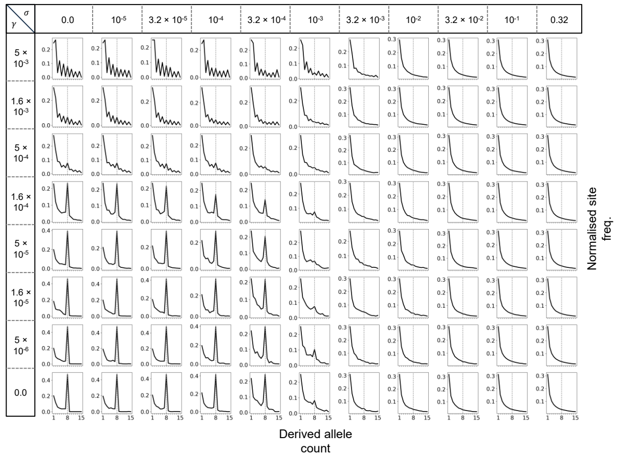
Fig. S2. Normalised site frequency spectrum (SFS; n = 8 individuals) across the simulated (Pieszko et al., 2025) space of the sex rate \sigma and the LOH rate \gamma . For each parameter combination, the SFS was obtained by summing site counts across 100 replicates and then normalising by the total number of sites; fixed derived sites are not shown. Dashed vertical lines indicate the 50% frequency class.
