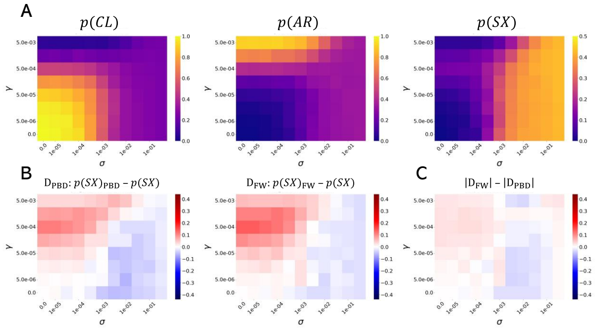
Fig. S2. Tree composition estimated through the PBD approach; comparison with FW inference through clustering ( k = 100 SNPs) given fragmented input sequence (5-kb segments). (A) p(CL) , p(AR) and p(SX) across the simulated space of sex rates \sigma and LOH rates \gamma (note the color scale is capped at 0.5 in the p(SX) heatmap). (B) Deviations D from true p(SX) associated with the PBD and FW approaches. (C) Absolute difference in deviations from true p(SX) between the two approaches: red indicates PBD is closer to truth, blue indicates FW is closer to truth.
