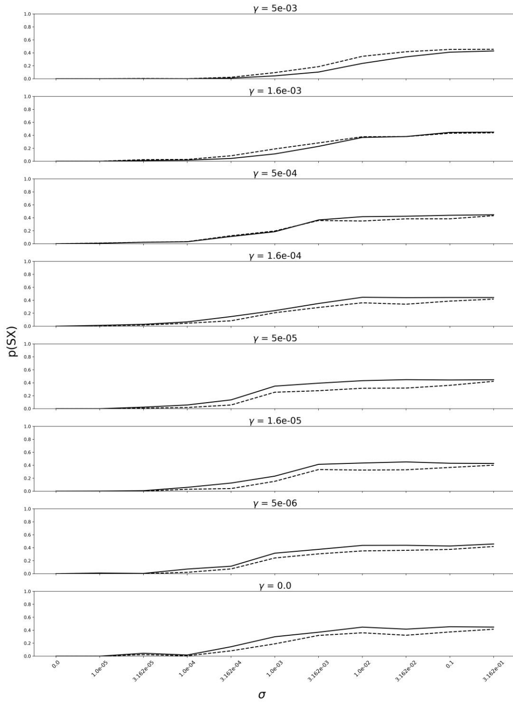
Fig. S8. True p(SX) (solid lines) and p(SX) in heterozygous genome regions ( \beta = 0.1 ; dashed lines) as a function of \sigma under different scenarios of \gamma ; MP model.
