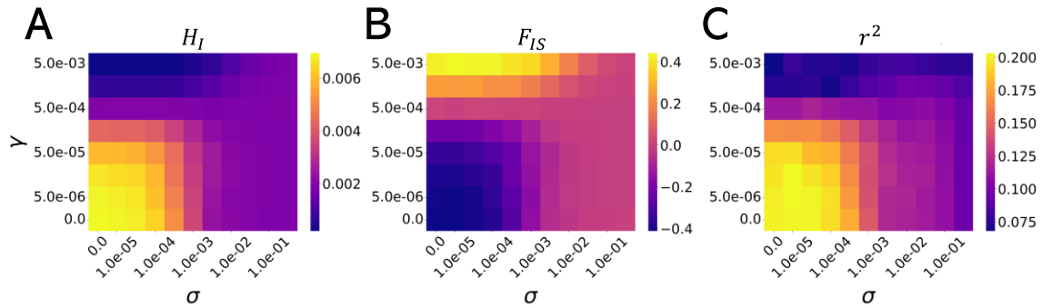
Fig. 3. Simulation results for population genetic statistics. Average H_I , F_{IS} and r^2 for SNP pairs < 1,000 bp apart across the space of the sex rate \sigma , increasing from the left to the right of each heatmap, and the LOH rate \gamma , increasing from the bottom to the top; MP model. For each scenario, mean statistic values were obtained for samples of 100 random individuals and averaged across 100 replicates.
