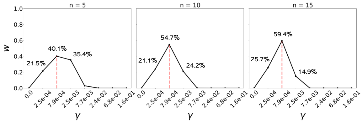
Fig. S3. Akaike weights of evidence ( w ) for different LOH rates \gamma given an observed F_{IS} = 0 and distributions of values obtained via sampling n = 5, 10 or 15 individuals from obligate CF populations replicated 100 times. Dashed vertical lines indicate \gamma closest to \frac{1}{2N} .
