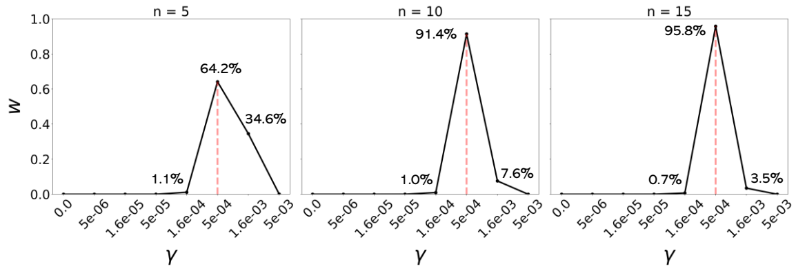
Fig. S2. Akaike weights of evidence ( w ) for different LOH rates \gamma given an observed F_{IS} = 0 and distributions of values obtained via sampling n = 5, 10 or 15 individuals from obligate MP populations replicated 100 times. Dashed vertical lines indicate \gamma = \frac{1}{2N} .
