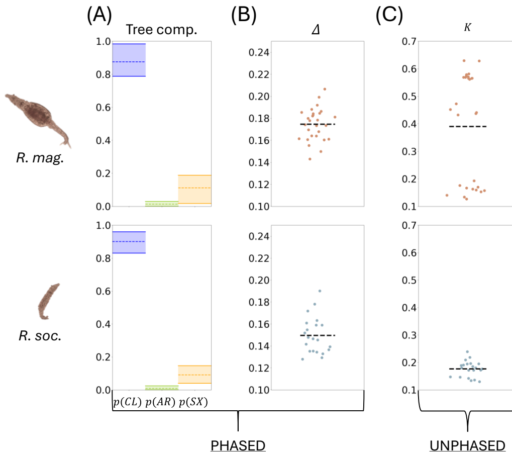
Fig. 4. Results of genealogical analysis in Rotaria : metrics calculated for phased segments (A - tree composition, B - \Delta ) and unphased, genome-wide SNPs (C - K ). Each plot is based on values obtained for the 28 pairs of individuals from the Silwood populations. Dashed horizontal lines denote means; the tree composition plots additionally show the spread (minimum-maximum) within each tree category.
