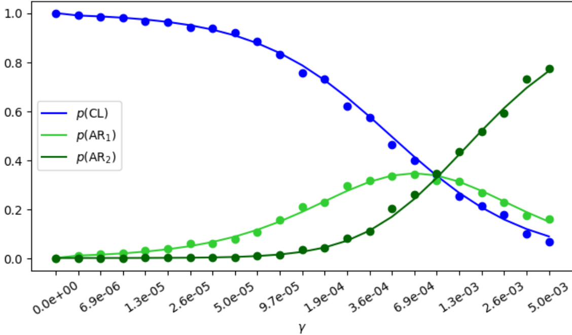
Fig. B. Tree proportions p(CL) , p(AR_1) and p(AR_2) under obligate asexuality and a range of per-locus, per-generation LOH rates \gamma ( N = 1000 ): comparison of expressions obtained here (lines) and the values obtained using the MP model (points; each scenario in 100 replicates).
