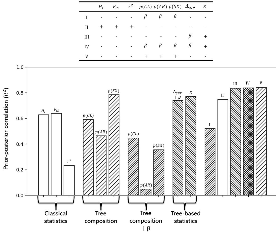
Fig. 6. Predictability of the sex rate \sigma from different summary statistics: the coefficient of determination ( R^2 ) between the prior (simulated; MP model) and posterior values obtained through rejection-based approximate Bayesian computation (ABC) (Csilléry et al., 2012). The predictive power of statistics was tested individually and in combinations I-V (see the legend at the top; '+' – included, '-' – excluded, ' \beta ' – calculated under heterozygosity bias). The per-simulation vectors of summaries were obtained using samples of 8 individuals.
