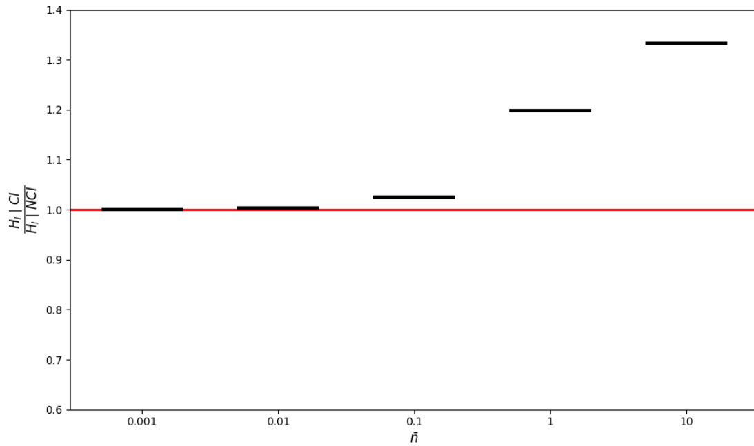
Fig. S17. Comparison of the CI and NCI models of crossover recombination during central fusion. A ratio of the equilibrium individual-level heterozygosity \hat{H}_I under the CI model to that expected under the NCI model as a function of the expected number of crossovers between the centromere and the focal locus \bar{n} .
