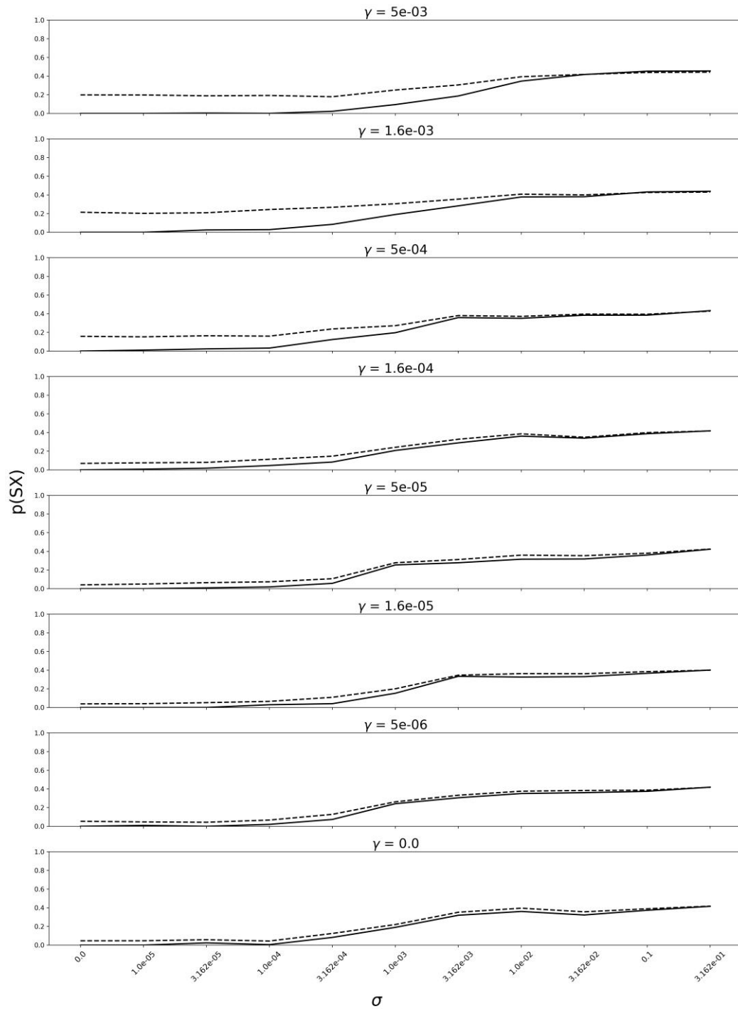
Fig. S10. p(SX) in heterozygous genome regions ( \beta = 0.1 ; solid lines) and p(SX) after additional genealogical inference with SINGER (dashed lines) as a function of \sigma under different scenarios of \gamma ; MP model.
