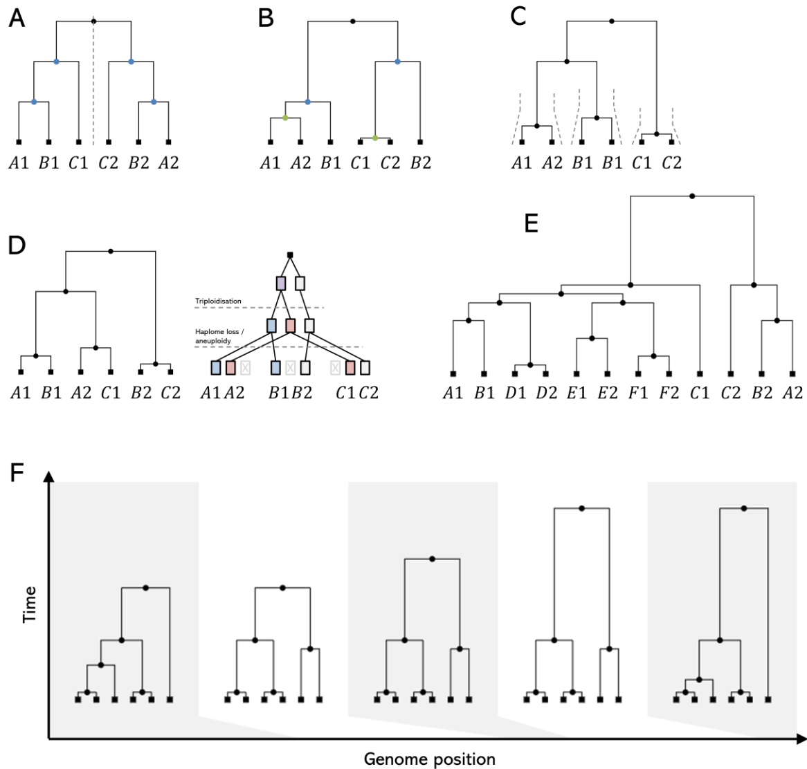
Fig. 2. Genealogical relationships and reproductive mode. The trees are shown for individuals A-F, each with haplotypes 1 and 2. (A) Topological Meselson effect under clonality; blue nodes correspond to splits between asexual lineages. (B) Asygamous LOH at terminal branches (green nodes) brings haplotypes together within individuals. (C) Clustering of haplotypes by population of origin: sex (Brandt et al., 2021) or asygamous recombination? (D) The 'allele sharing' pattern: sex (Vakhrusheva et al., 2020) or triploidisation followed by loss of homologous copies (right)? (E) Half of haplotypes cluster with a different population: hybridisation (see Fig. 2B in Rogers et al., 2014; Fig. 7 in Vakhrusheva et al., 2020) or asexuality with lineage-heterogenous LOH? (F) An ARG represented as a sequence of local trees: a sexual example simulated with msprime v1.3.2 (Baumdicker et al., 2022). Each tree describes a local non-recombining genealogy.
