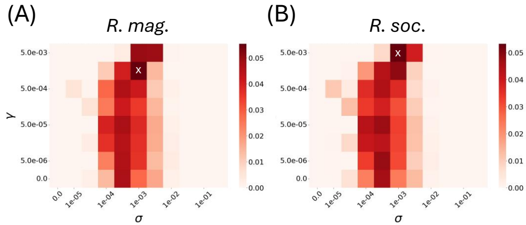
Fig. S7. Likelihood of mean \Delta for Silwood populations across the simulated (Pieszko et al., 2025) space of the sex rate \sigma and the LOH rate \gamma (optimised mutation rates; \beta = 0.05 ). Likelihoods were computed assuming normal distribution of simulated values per scenario (mean for 8 individuals per simulation; 100 replicates), then normalising across scenarios. White 'x' symbols mark the scenarios with highest likelihoods. (A) R. magnacalcarata . (B) R. socialis .
