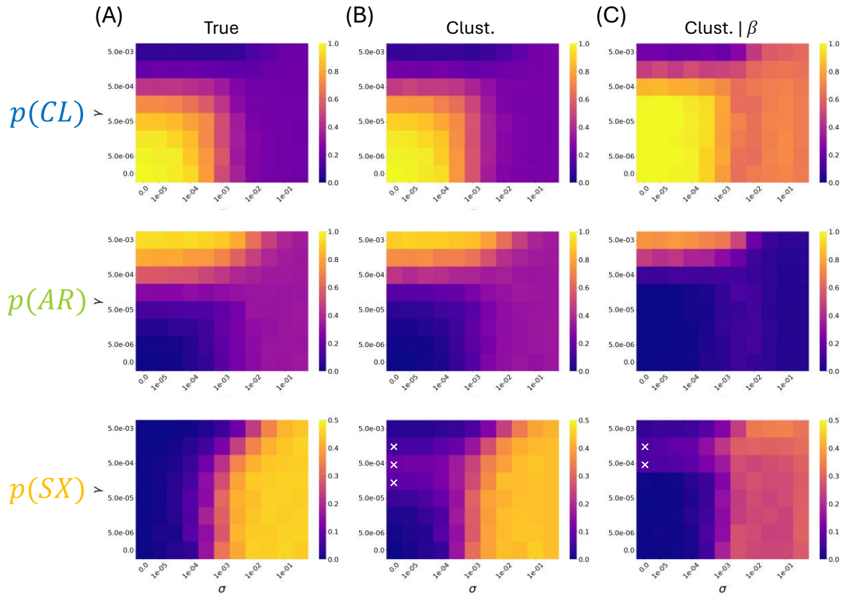
Fig S3. Proportions p of CL, AR and SX trees across the simulated (Pieszko et al., 2025) space of the sex rate \sigma and the LOH rate \gamma . Per simulation, mean values were computed for samples of 8 individuals; each scenario was replicated 100 times. White 'x' mark obligate asexual scenarios where p(SX) > 0.05 . (A) True proportions. (B) Proportions reconstructed using the clustering approach ( k = 100 ). (C) Proportions reconstructed using the clustering approach ( k = 100 ), given Rotaria -optimised mutation rates and when \beta = 0.05 .
