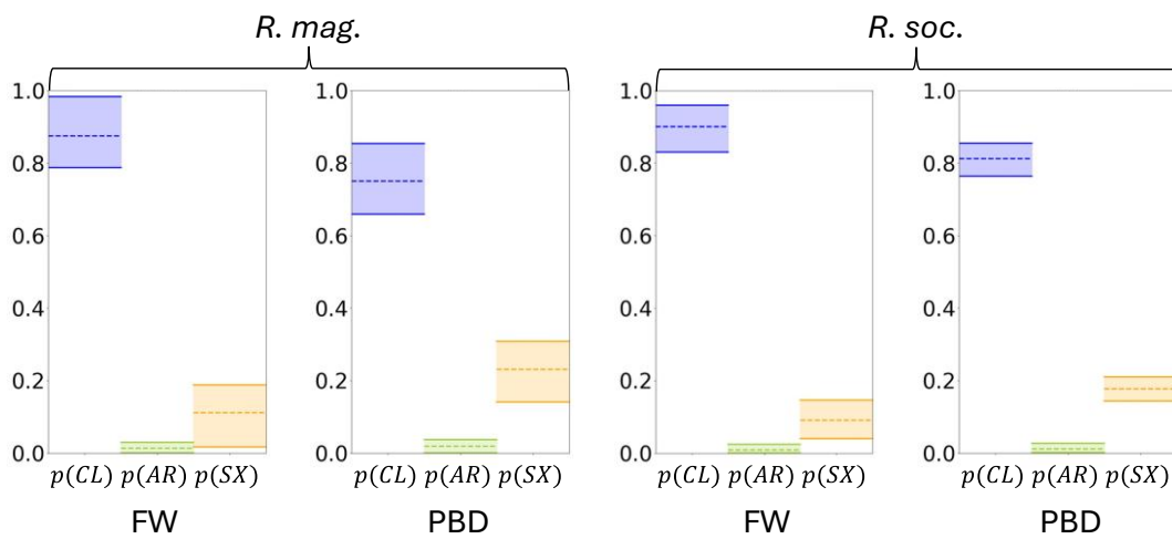
Fig. 5. PBD-based estimates of tree composition compared with those obtained using standard genealogical inference in fixed-length windows (the 'FW' approach; k = 100 SNPs). The FW estimates are reproduced from Fig. 4A. For both species, only individuals from the Silwood populations were included.
