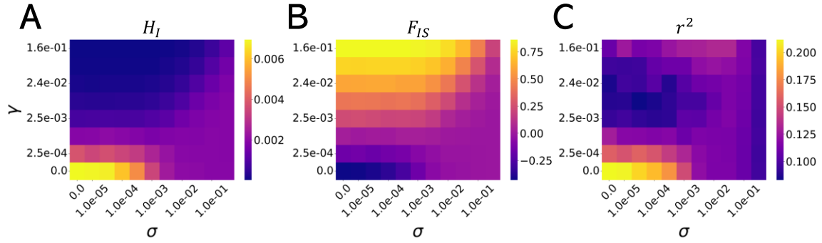
Fig. S1. H_I , F_{IS} and r^2 for SNPs < 1,000 bp apart across the space of the sex rate \sigma , increasing from the left to the right of each heatmap, and the LOH rate \gamma , increasing from the bottom to the top; CF model. For each scenario, mean statistic values were obtained for samples of 100 random individuals and averaged across 100 replicates.
