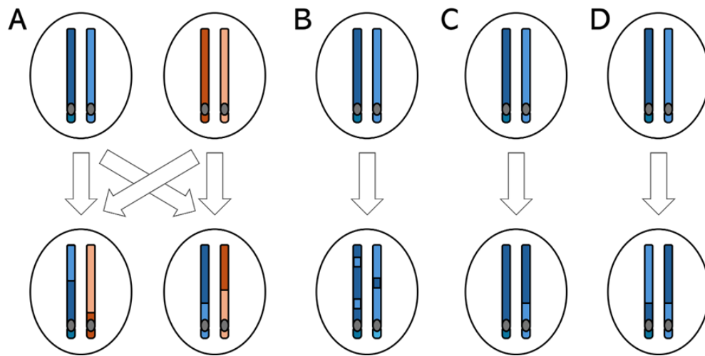
Fig. 1. Immediate effects of sexual and asexual reproduction on sequence diversity across a diploid chromosome arm. (A) Sexual reproduction with crossover recombination. (B) Mitotic parthenogenesis with gene conversion. Gene conversion during mitotic parthenogenesis results in localised loss of heterozygosity (LOH). (C) Meiotic parthenogenesis (central fusion automixis) with crossover recombination. Crossovers during central fusion automixis may result in long-range LOH or reciprocal recombination with a change of linkage (D).
