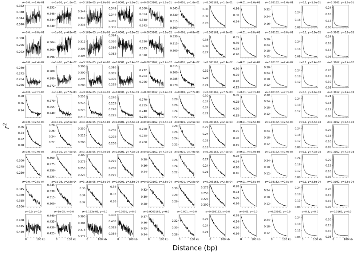
Fig. S5. r^2 as a function of inter-site distance across the space of sex rates \sigma and LOH rates \gamma ; CF model. r^2 was calculated using samples of 10 individuals and a maximum of 500 SNPs. Variability in some curves is due to a limiting number of SNPs.
