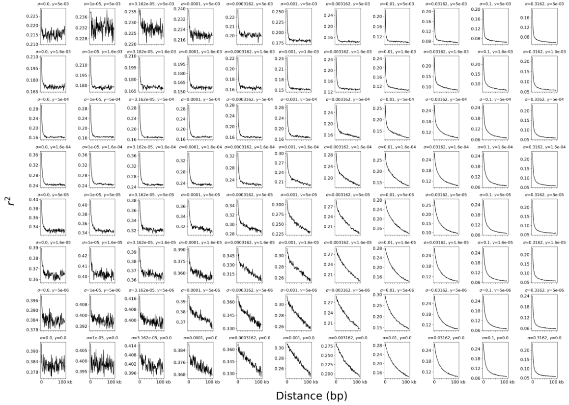
Fig. S4. r^2 as a function of inter-site distance across the space of sex rates \sigma and LOH rates \gamma ; MP model. r^2 was calculated using samples of 10 individuals and a maximum of 500 SNPs. Variability in some curves is due to a limiting number of SNPs.
