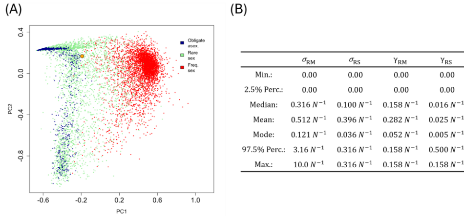
Fig. 5. The multidimensional space of simulated p(CL) , p(AR) , p(SX) , \Delta and K values (phased-segment statistics computed under \beta = 0.05 ). (A) The positioning of R. magnacalcarata (orange) and R. socialis (blue) from Silwood populations against the first two principal components. Scenarios of frequent sex are defined by sex rates > \frac{1}{N} , where N = 1,000 is the simulated population size. (B) Summaries of the posterior distributions of the rate of sex \sigma and rate of LOH \gamma obtained through rejection-based approximate Bayesian computation (ABC) (Csilléry et al., 2012). Values are expressed in terms of N (= 1,000) for general comparisons.
