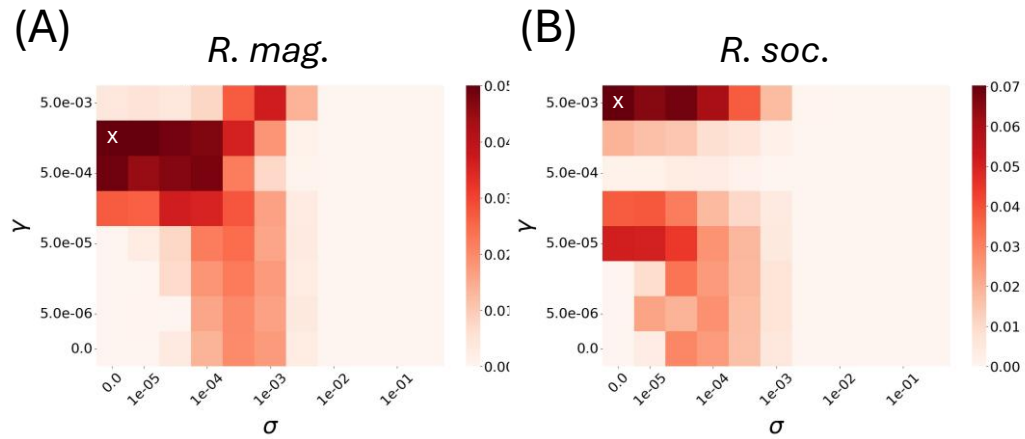
Fig. S6. Likelihood of mean K for Silwood populations across the simulated (Pieszko et al., 2025) space of the sex rate \sigma and the LOH rate \gamma (optimised mutation rates). Likelihoods were computed assuming normal distribution of simulated values per scenario (mean for 8 individuals per simulation; 100 replicates), then normalising across scenarios. White 'x' symbols mark the scenarios with highest likelihoods. (A) R. magnacalcarata . (B) R. socialis .
