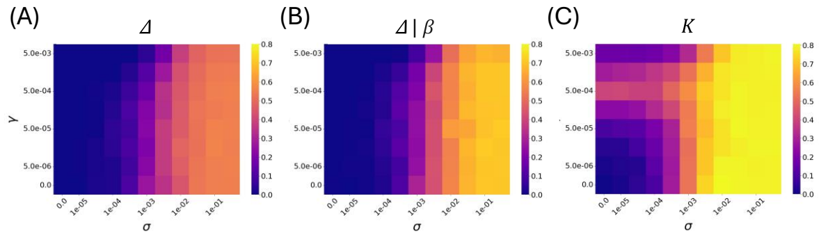
Fig. S5. \Delta and K across the simulated (Pieszko et al., 2025) space of the sex rate \sigma and the LOH rate \gamma . Per simulation, mean values were computed for samples of 8 individuals; each scenario was replicated 100 times. (A) \Delta computed using the SNP-based procedure (optimised mutation rates). (B) \Delta (optimised mutation rates; \beta = 0.05 ). (C) K (optimised mutation rates).
