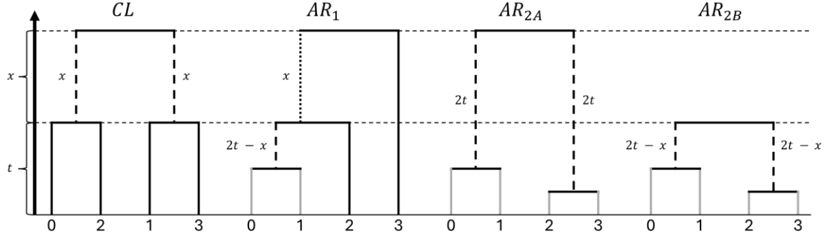
Fig. A. Two-individual, four-tip local trees under obligate asexuality with asynonymous recombination. Epoch t precedes the divergence of asexual lineages; epoch x precedes coalescence due to LOH. Branches that terminate in LOH within epoch t (with expected length x - t ) are marked in grey. The expected lengths of branches on which doubletons (dashed) and tripletons (dotted) arise are displayed alongside them.
