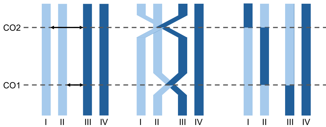
Fig. S14. Resolution of crossovers. Two crossovers occur: between chromatids II and III (CO1) and between chromatids I and III (CO2). Although chromatid II was not involved in CO2, the reconnecting of broken DNA molecules results in a double crossover on this chromatid.
