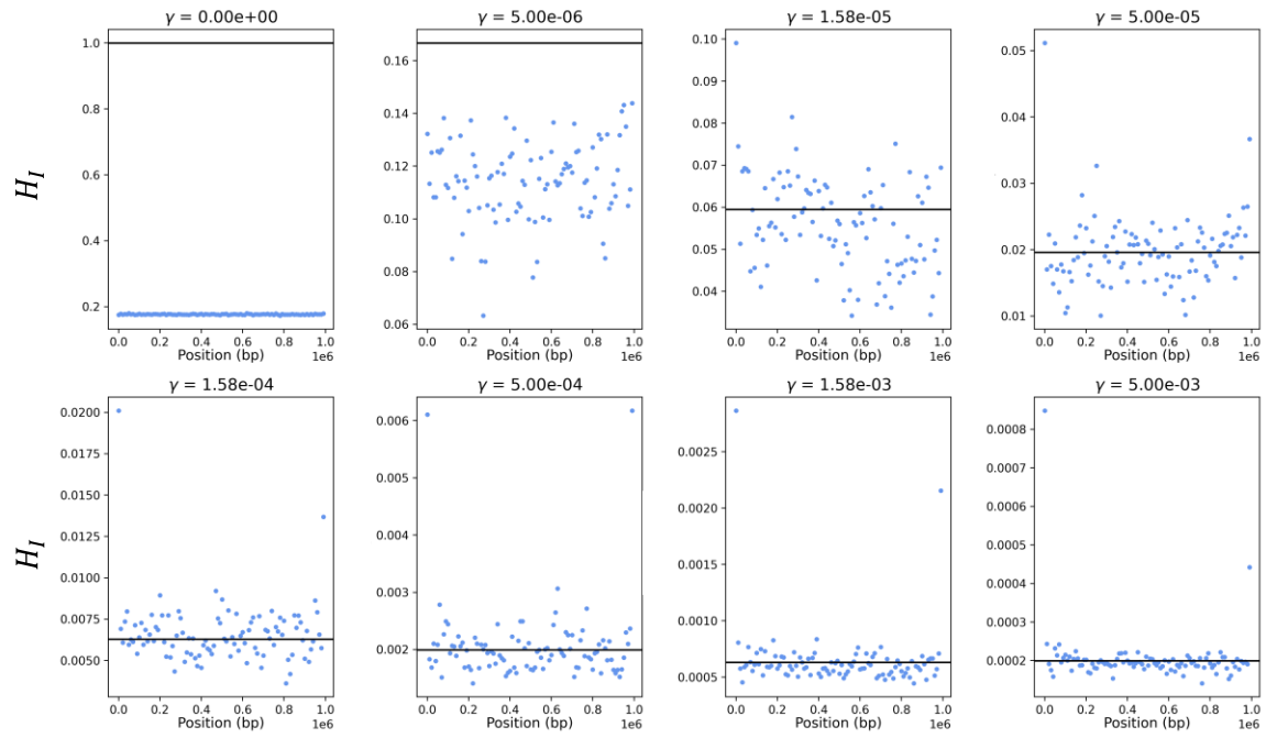
Fig. S15. H_I after 200,000 simulated generations of obligate mitotic parthenogenesis (MP) (blue dots) compared to the analytical predictions (black lines; section A, Eq. 7) under a range of LOH rates \gamma .
