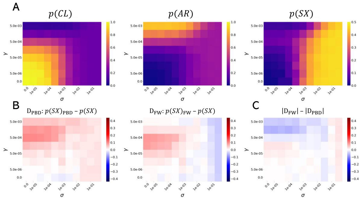
Fig. 1. Tree composition estimated through the PBD approach; comparison with FW inference through clustering ( k = 100 SNPs). (A) PBD-based p(CL) , p(AR) and p(SX) estimates across the simulated space of sex rates \sigma and LOH rates \gamma (note the color scale is capped at 0.5 in the p(SX) heatmap). (B) Deviations D from true p(SX) associated with the PBD and FW approaches. (C) Absolute difference in deviations from true p(SX) between the two approaches: red indicates PBD is closer to truth, blue indicates FW is closer to truth.
