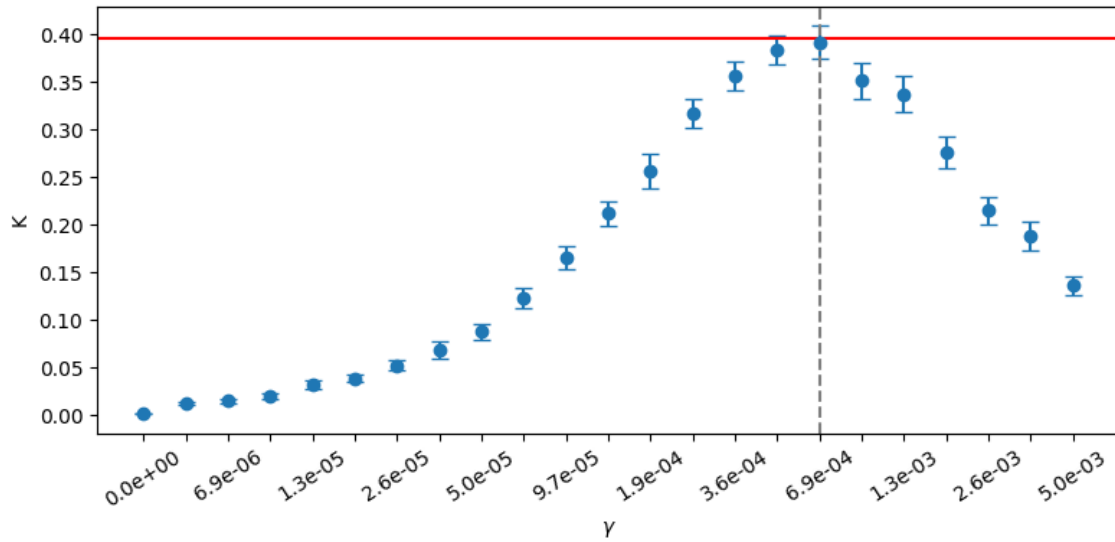
Fig. C. K under obligate asexuality and a range of per-locus, per-generation LOH rates \gamma ( N = 1000 ): comparison of the maximum value obtained here (red line) and the values obtained using the MP model (points; bars show standard error among 100 replicates).
