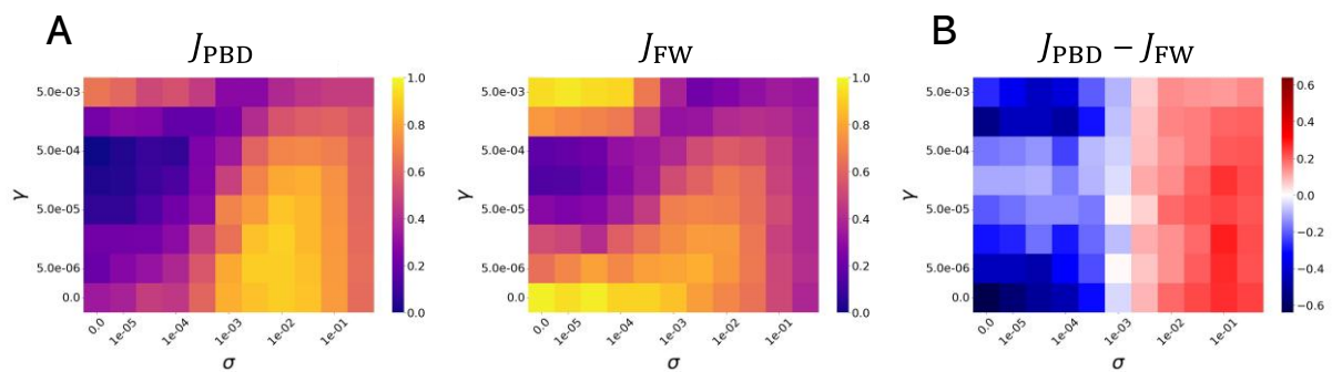
Fig. 3. Accuracy of SX block delimitation through the PBD and FW ( k = 100 SNPs) approaches. (A) Comparisons against the simulated ground truth as measured with the Jaccard similarity index J . (B) Difference in J between the two approaches. Blue regions correspond to higher accuracy of FW; red regions correspond to higher accuracy of PBD.
