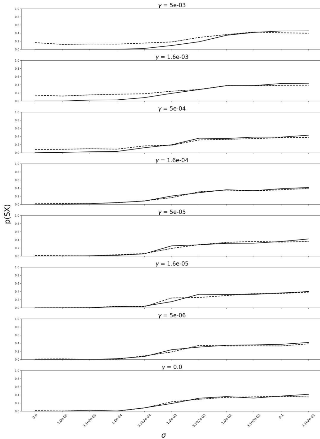
Fig. S9. p(SX) in heterozygous genome regions ( \beta = 0.1 ; solid lines) and p(SX) after additional genealogical inference with IQ-TREE (dashed lines) as a function of \sigma under different scenarios of \gamma ; MP model.
