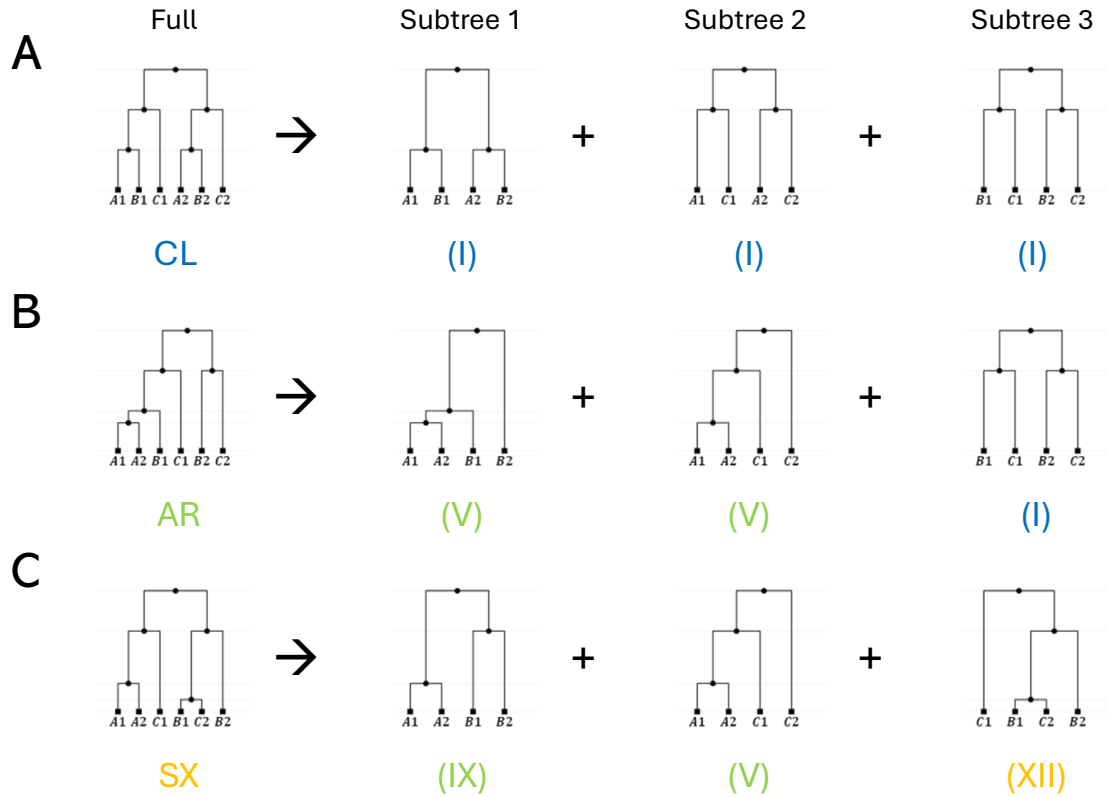
Fig. S6. Exhaustive tree classification: example of 3 individuals. To disentangle the reproductive history, trees for individuals A , B and C (each with alleles 1 and 2) can be decomposed into subtrees for the \binom{3}{2} possible pairs of individuals. Roman numerals and colours correspond to Fig. 4A. (A) A clonal tree is decomposed into CL subtrees (note the equal timing of internal nodes that is not recovered by many inference algorithms and hence ignored in Fig. 4A). (B) The signature of asynonymous recombination is reflected in subtrees 1 and 2. (C) The signature of sex is reflected in subtree 3.
