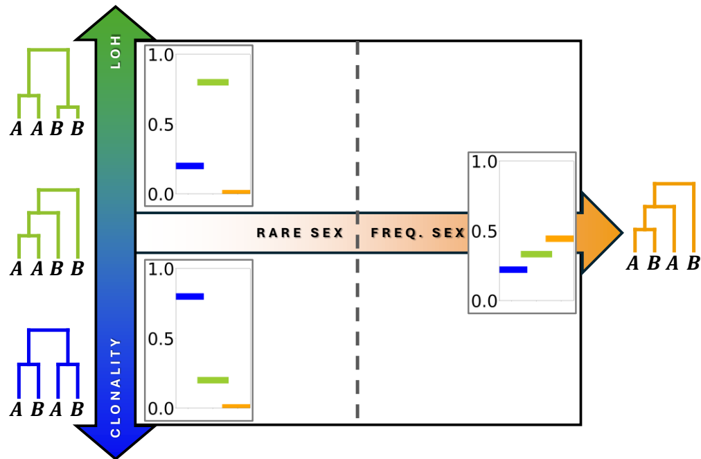
Fig. 3. Genealogical signatures of reproductive mode. Relative proportions p of CL (blue), AR (green) and SX (orange) classes of four-tip trees ('tree composition'; bar plots) distinguish asexual and sexual scenarios (axes). Trees are shown for diploid individuals A and B . Total p(AR) , and the proportion of balanced AR trees (top left), increase with the rate of asynonymous recombination; p(SX) increases with the rate of sex. See Pieszko et al. (2025) for more details.
