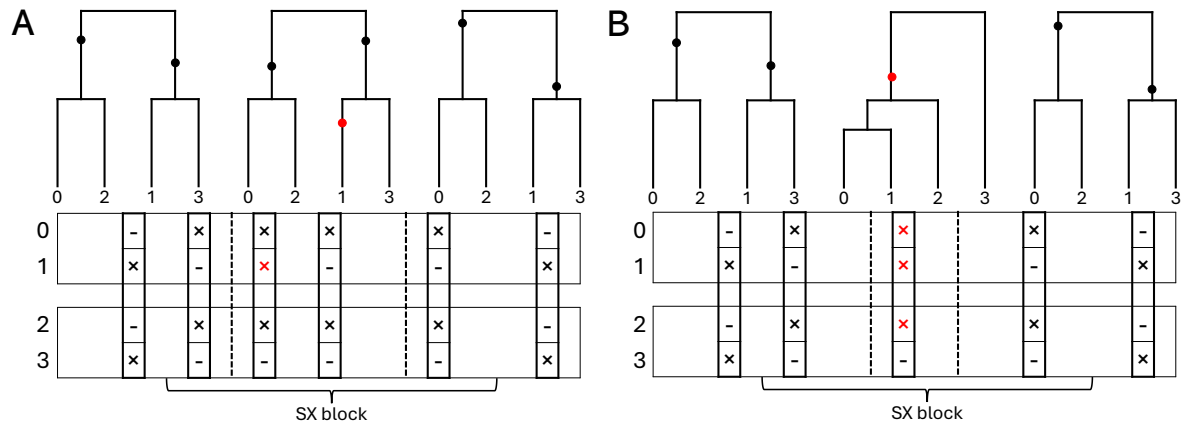
Fig. 4. Spurious sex signals identified by the PBD approach. (A) An SX block anchored at a triplet that arose through recurrent mutation (homoplasy). (B) An SX block anchored at a triplet that arose on an unbalanced AR tree.
