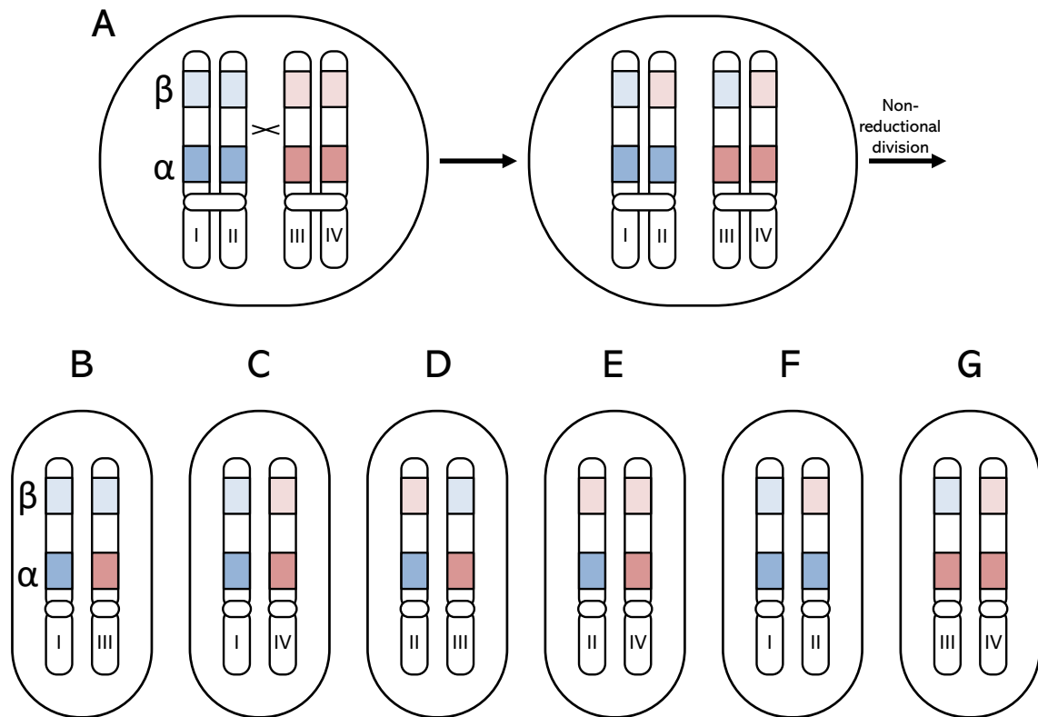
Fig. 1. Asexual chromatinid segregation modulates the consequences of recombination: a two-locus example with a single crossover (CO). (A) A CO between loci \alpha and \beta leads to a recombinant configuration at the CO-distal locus \beta , followed by a non-reductional (mitotic or meiotic) cell division. (B-G) The six theoretically possible combinations of chromatids in a non-reduced gamete. Random pairing with equiprobable outcomes B-G results in a \frac{1}{3} chance of LOH (non-simultaneously) at either locus. If only non-sister chromatids co-segregate (B-E), as in mitotic and certain forms of meiotic asexuality ('central fusion automixis'; Suomalainen et al., 1987), a \frac{1}{2} chance of LOH at locus \beta is expected, with no LOH at locus \alpha . If only sister chromatids co-segregate (F and G), as in certain forms of meiotic asexuality ('terminal fusion automixis'; Suomalainen et al., 1987), LOH is avoided at locus \beta but occurs at locus \alpha . See Stenberg and Saura (2009) for cytological diagrams of how ploidy is restored in different forms of non-reductional meiosis.
