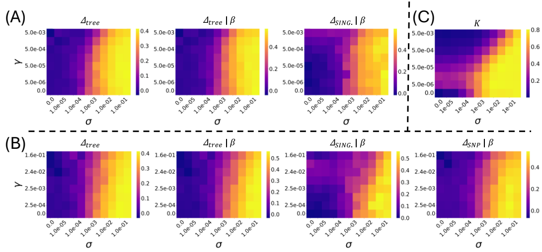
Fig. S13. Tree-based statistics across the space of the sex rate \sigma , increasing from the left to the right of each heatmap, and the LOH rate \gamma , increasing from the bottom to the top; supplementary results. (A) \Delta calculated based on true trees ( \Delta_{tree} ) or reconstructed trees ( \Delta_{SING.} ); MP model. \beta = 0.1 . (B) \Delta calculated based on true ( \Delta_{tree} ), reconstructed trees ( \Delta_{SING.} ) or SNP-based intervals ( \Delta_{SNP.} ); CF model. \beta = 0.1 . (C) K under the CF model.
