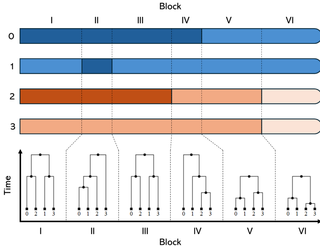
Fig. 2. Changes in sequence diversity along a heterogeneous genealogy. In this example, the genealogy of two diploid individuals (blue and orange, with chromosomes 0, 1 and 2, 3, respectively) changes due to asynonymous recombination. The resulting patterns of diversity, with loss of heterozygosity (LOH) in one (blocks II and IV) or both (blocks V and VI) individuals, occurring more anciently (e.g., block II) or recently (e.g., block VI), are best represented as the underlying ancestral recombination graph (ARG) with local trees that describe non-recombining histories.
