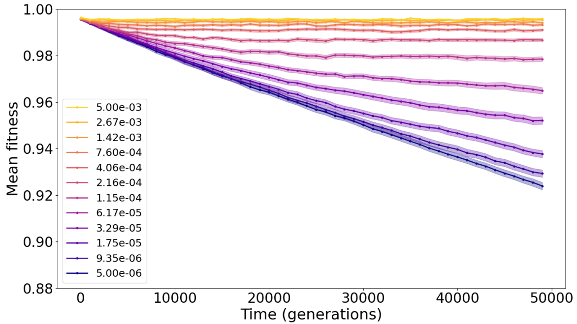
Fig. 1. Asygamous recombination-associated LOH rescues fitness of asexual populations: a time-series. MP scenarios (chromosome length L = 1 Mb; population size N = 1,000 ; mean gene conversion tract length \lambda = 5,000 bp) were simulated with \gamma varying between 5 \times 10^{-6} and 5 \times 10^{-3} , and the per-site per-generation mutation rate \mu of 5 \times 10^{-9} . Each scenario was replicated 100 times. In a simple model of background selection, selection coefficients s of new mutations were drawn from a gamma distribution s \sim \text{Gamma}(\bar{s} = -0.01, \alpha = 0.2) , where \bar{s} is the mean and \alpha is the shape parameter. Dominance coefficients were fixed at 0.2. Shaded areas represent 95% confidence intervals.
