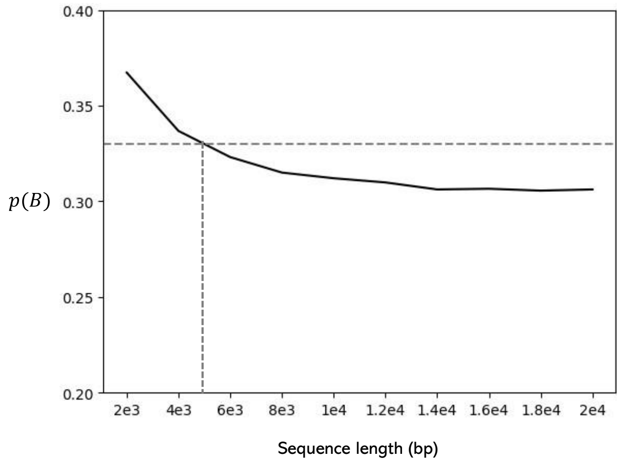
Fig. S1. Proportion of balanced trees p(B) obtained through the PBD approach as a function of sequence length: obligate sexual scenarios simulated using msprime v1.3.2 ( r = \mu = 10^{-6} , N = 1,000 ) (Baumdicker et al., 2022). Dashed horizontal line represents the expected value of p(B) under obligate sex.
