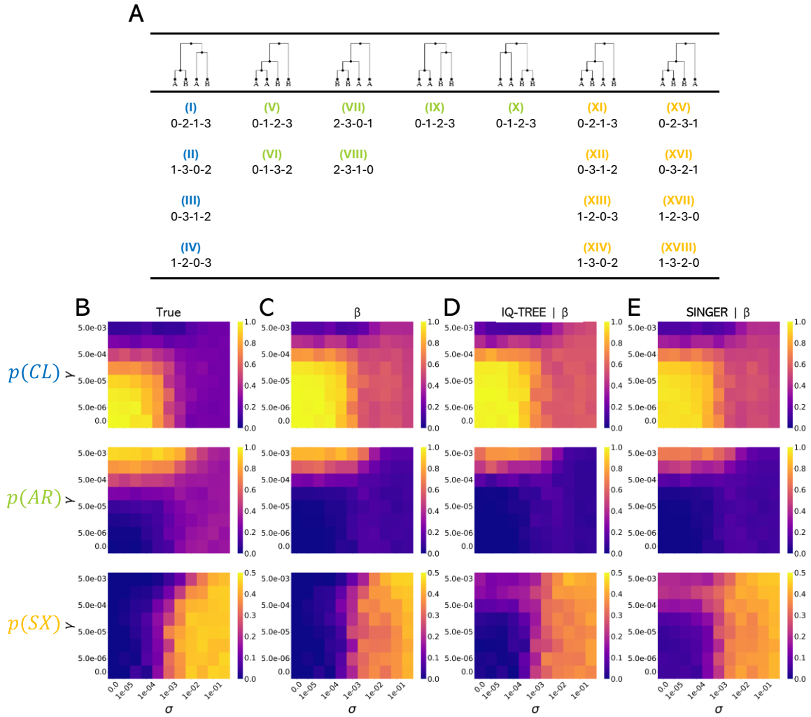
Fig. 4. Systematic analysis of tree composition. (A) The 18 two-individual, four-tip coalescent trees can be classified into three categories: clonality-compatible (CL; blue), asygamous recombination-compatible (AR; green) and sex-specific (SX; orange). Here, the trees are drawn for individuals A (homologs 0 and 1) and B (homologs 2 and 3), with the possible tip labelling displayed below. (B)-(E) Tree proportions p falling into the CL, AR and SX categories across the space of the sex rate \sigma , increasing from the left to the right of each heatmap, and the LOH rate \gamma , increasing from the bottom to the top; MP model. p(CL) , p(AR) and p(SX) reflect the rates of sex and asygamous recombination (B), a relationship that is biased towards CL trees through sampling heterozygous genome regions (C), and broken down when SX trees are generated through inference error (D – IQ-TREE, E – SINGER). Note that the colour scale is capped at 1.0 in the p(CL) and p(AR) heatmaps and at 0.5 in the p(SX) heatmaps.
