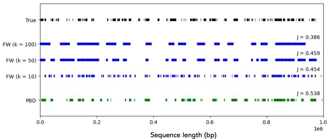
Fig. 2. Breakpoint delimitation through the PBD (green) and FW (blue) approaches: SX blocks in an example ARG ( \sigma = 0.001 , \gamma = 5 \times 10^{-4} ). The accuracy of SX blocks recovered by the FW approach depends on window size k . For the given example ARG, the PBD approach performs best (Jaccard similarity index values J on the right).
