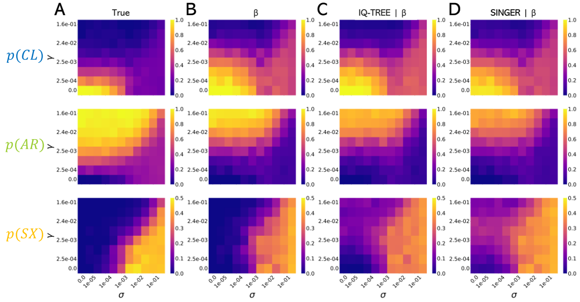
Fig. S7. Tree proportions p falling into the CL, AR and SX categories across the space of the sex rate \sigma , increasing from the left to the right of each heatmap, and the LOH rate \gamma , increasing from the bottom to the top; CF model. Note that the colour scale is capped at 1 in the p(CL) and p(AR) heatmaps, and at 0.5 in the p(SX) heatmaps. (A) True values. (B) Heterozygosity bias of \beta = 0.1 . (C) IQ-TREE inference, (D) SINGER inference.
