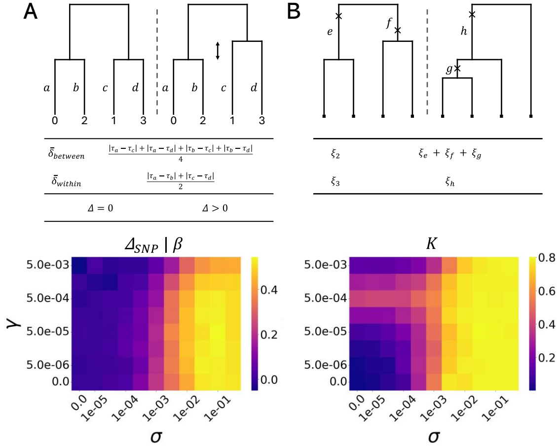
Fig. 5. Tree-based statistics to distinguish between asexual and sexual scenarios. (A) \Delta : a statistic calculable for haplotype-resolved segments. Top: example CL trees with equal (left) and unequal (right) timing of internal nodes. The lengths \tau of branches a, b, c and d are used to calculate \bar{\delta}_{between} and \bar{\delta}_{within} ; see Results. The values of \Delta reflect the asymmetry in the timing of internal nodes in CL and SX trees. Bottom: variation in \Delta is driven by the rate of sex \sigma . (B) K : a statistic calculable for genome-wide SNPs. Top: Mutations ('x') arising on different branches of balanced (left; CL or AR) and unbalanced (right; AR or SX) trees contribute to the pool of doubletons ( \xi_2 ) and tripletons ( \xi_3 ). \xi_2 and \xi_3 can be used to summarise the genome-wide signal of reproductive mode; see Results. Bottom: K values vary with the rate of LOH \gamma but are predominantly driven by the rate of sex \sigma .
