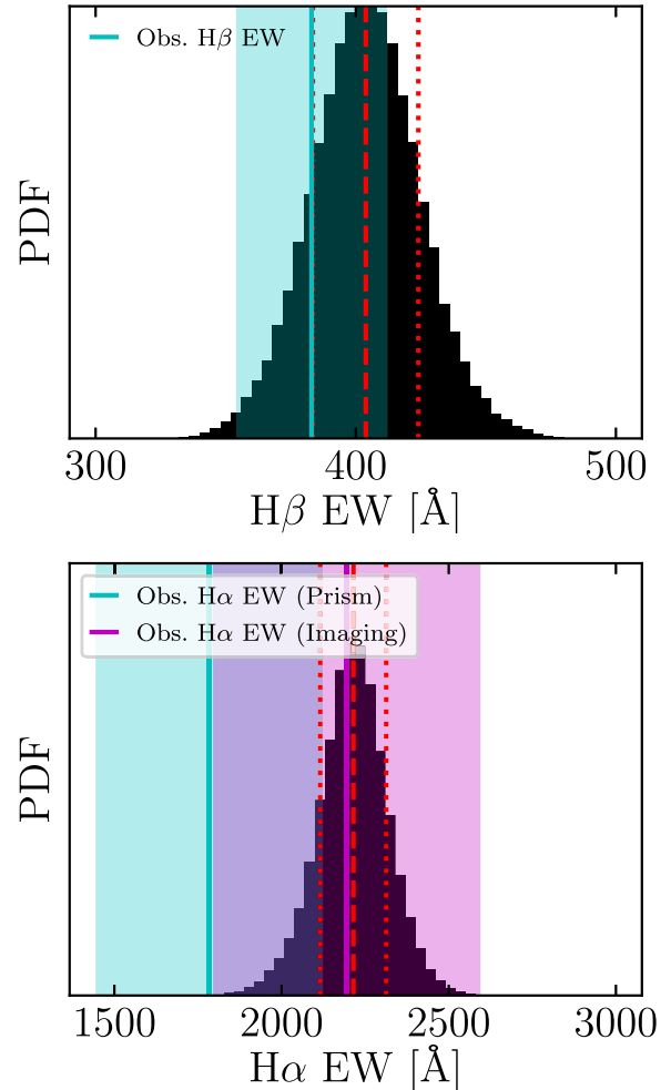
Figure 8. Top: Posterior distribution on H \beta equivalent width predicted by the continuum fitting. The median and 1\sigma values (red lines) are consistent with that measured from the Prism spectrum (blue). Bottom: Same as top panel, but for H \alpha . Here, the median and 1\sigma values (red lines) are somewhat higher than that measured from the Prism spectrum (blue), but in good agreement with the equivalent width implied by the medium-band imaging.
