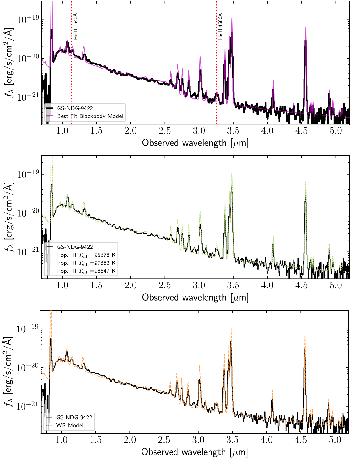
Figure 10. Top: Spectrum of GS-NDG-9422 (black) compared with the best-fitting blackbody model (magenta) with T_{\text{BB}} = 10^{5.05} K and a He II leakage fraction of 0.22 (Table 4; Section 5.2). Middle: Spectrum of GS-NDG-9422 (black) compared with photoionization models powered by various individual massive Pop. III stars with different effective temperatures. Bottom: Spectrum of GS-NDG-9422 (black) compared with the photoionisation model powered by a model Wolf-Rayet SED with the most similar spectrum to the best-fitting blackbody SED. All models can also reproduce the observed spectrum well (dotted lines). See Section 5.2 for details.
