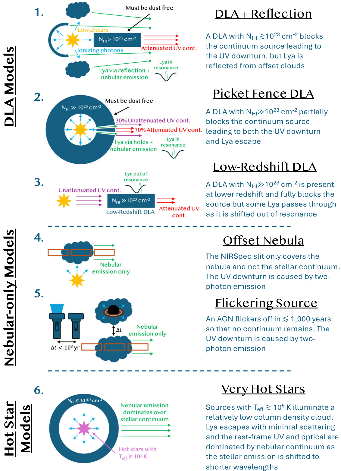
Figure 15. Summary of the three classes of scenarios that can explain the spectrum on GS-NDG-9422. For each scenario, we show various cartoons for how the physics may manifest and give rise to a steep UV slope, a high- \text{Ly}\alpha escape fraction, and the UV turnover redward of \text{Ly}\alpha .
