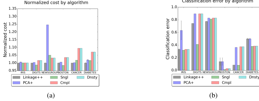
Figure 1: A comparison of the algorithms on real-world data. (a) The figure shows the cost \text{cost}(\cdot) of the algorithm normalized by the cost of LINKAGE++. (b) The figure shows the percentage of misclassified nodes. By looking more closely at the output of the algorithm, one can see that a large fraction of the misclassifications happen in subgroups of the same group.
