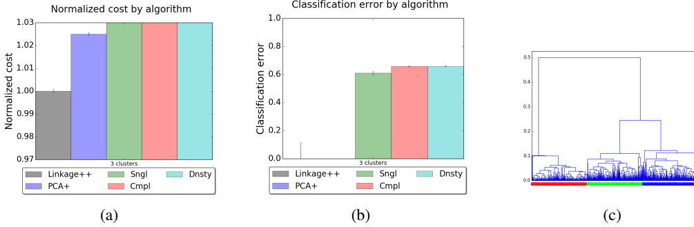
Figure 3: The clustering obtained by PCA+ on a ground truth tree on three nodes induced by the adjacency matrix \begin{bmatrix} 1. & 0.49 & 0.39 \\ 0.49 & 1. & 0.39 \\ 0.39 & 0.39 & 1. \end{bmatrix} and n = 999 nodes split equally. Here only LINKAGE++ and PCA+ classify the bottom clusters of the subtrees correctly. However, the projection to the euclidian space (PCA) does not preserve the underlying ultrametric causing PCA+ to merge incorrectly. (a) LINKAGE++ recovers the ground truth. All other algorithm merge incorrectly. (b) LINKAGE++ and PCA+ classify the bottom clusters correctly causing the classification to be perfect even though PCA+ failed to correctly reconstruct the ground-truth. This suggests that the classification error is less suitable measure for hierarchical data. (c) PCA+ in contrast to LINKAGE++ merges incorrectly two bottom clusters of different branches in the ground-truth tree (green and blue as opposed to green and red).
