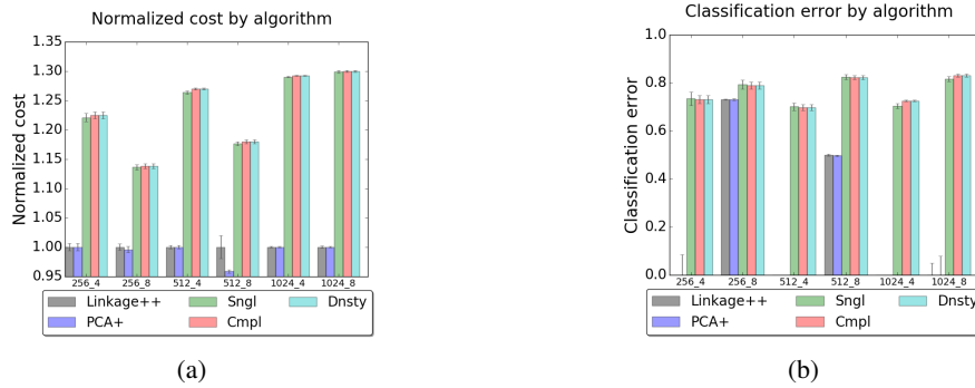
Figure 2: A comparison of the algorithms on synthetic data for highly structured ground-truth for different n, k . PCA+ performs well on these inputs and we conjecture that this is due to the highly structured nature of the ground-truth. (a) The cost of LINKAGE++ and PCA+ are well-below the costs of the standard linkage algorithms. (b) We see a threshold phenomena for k = 8 from n = 512 to n = 1024 . Here the classification error drops from 0.5 to 0, which is explained by concentration of the eigenvalues allowing the PCA to separate the bottom clusters correctly.
