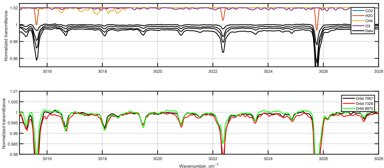
Fig. 2. Top panel: Consecutive ACS MIR transmission spectra measured in diffraction order 180 at tangent altitudes 8–18 km (orbit 7067, black curves), against synthetic models indicating potential contributions of different atmospheric components at 10 km with MIR resolution (coloured curves): 15 ppmv of water vapour, 1 ppbv of methane, and 200 ppbv of ozone. Three H 2 O lines and a series of periodic unidentified features are apparent. Bottom panel: Similar spectra measured in three selected orbits (6975, 7067, and 7326) at tangent altitudes of 10 km.
