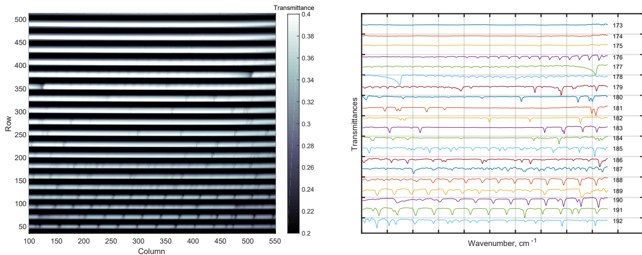
Fig. 1. Left panel: Example of a single detector frame measured by ACS MIR in secondary grating position 12 after processing (orbit 6975, L_s = 40.3^\circ , tangent altitude 13 km). Right panel: Associated series of transmission spectra (right panel), covering the wavenumber range from 2894 \text{ cm}^{-1} (diffraction order 173) to 3239 \text{ cm}^{-1} (order 192). The left and right edges of the frame in the spectral dimension, where the signal decreases, are cropped.
