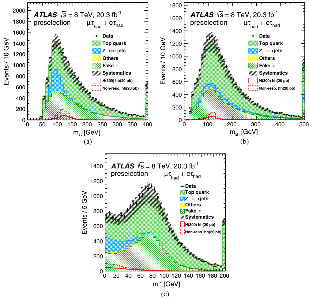
FIG. 2 (color online). Kinematic distributions of the hh \rightarrow b\bar{b}\tau\tau analysis after the preselection (see text) comparing data with the expected background contributions: (a) dilepton mass m_{\tau\tau} reconstructed using the MMC method, (b) dijet mass m_{bb} , and (c) the transverse mass m_T^{E_T^{\text{miss}}} of the lepton and the E_T^{\text{miss}} system. The top quark background includes contributions from both t\bar{t} and the single top-quark production. The background category labeled “Others” comprises diboson and Z \rightarrow ee/\mu\mu contributions. Contributions from single SM Higgs boson production are included in the background estimates, but are too small to be visible on these distributions. As illustrations, expected signal distributions for a Higgs boson pair production cross section of 20 pb are overlaid for both nonresonant and resonant Higgs boson pair production. A mass of m_H = 300 GeV is assumed for the resonant production. The last bin in all distributions represents overflows. The gray hatched bands represent the uncertainties on the total background contributions. These uncertainties are largely correlated from bin to bin.
