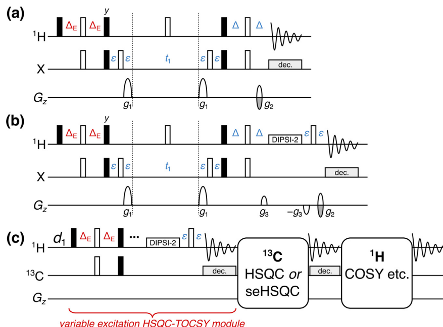
Fig. 4. (a) NOAH HSQC module with modified INEPT delay \Delta_E = (\arcsin f)/(4 \cdot J_{\text{CH}}) , where f is the fraction of ^1\text{H}^{\text{C}} magnetisation excited. (b) NOAH HSQC-TOCSY module (“ \text{S}^{\text{T}} ”), modified from the ASAP-HSQC-TOCSY [10]. The gradients g_3 are 1 ms long and have an amplitude of 10.1 G/cm. (c) Overview of a NOAH-3 \text{S}'\text{X} or \text{S}^{\text{T}}\text{X} supersequence. The ^1\text{H}^{\text{C}} magnetisation is partly used by the initial HSQC-TOCSY module, with a subsequent HSQC or seHSQC using the remaining ^1\text{H}^{\text{C}} magnetisation. The bulk ^1\text{H}^{\text{C}} magnetisation is retained for one or more homonuclear modules at the end. All other symbols have the same meanings as in Fig. 1.
