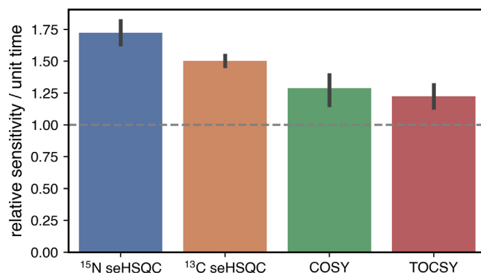
Fig. 6. Relative sensitivities per unit time ( \rho_t ) for the four modules in the S_N S_C CT supersequence (using a TOCSY mixing time of 35 ms). Error bars indicate 95% confidence intervals. The four NOAH modules, individually acquired, were used as the reference spectra ( \rho_t = 3.36 ). Spectra were obtained on a 700 MHz Bruker AV III equipped with a TCI H/C/N cryoprobe; the sample used was 50 mM zolmitriptan in DMSO- d_6 .
