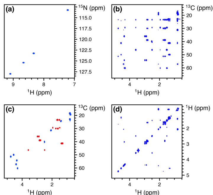
Fig. 5. Spectra obtained from the NOAH-4 \text{S}_\text{N}^+\text{S}_2^+\text{S}_2^+\text{C}^{\text{C}} supersequence. 256 t_1 increments were used, with 2 scans per increment. The total experiment time was 17 min and 35 s. (a) ^{15}\text{N} seHSQC. (b) ^{13}\text{C} HSQC-TOCSY (30 ms mixing, f = 0.9 ). (c) Multiplicity-edited ^{13}\text{C} ZIP-seHSQC. Notice that having the edited seHSQC removes the need for the less desirable HSQC-TOCSY editing. (d) CLIP-COSY. Spectra were obtained on a 700 MHz Bruker AV III equipped with a TCI H/C/N cryoprobe; the sample used was 40 mM gramicidin in \text{DMSO}-d_6 .
