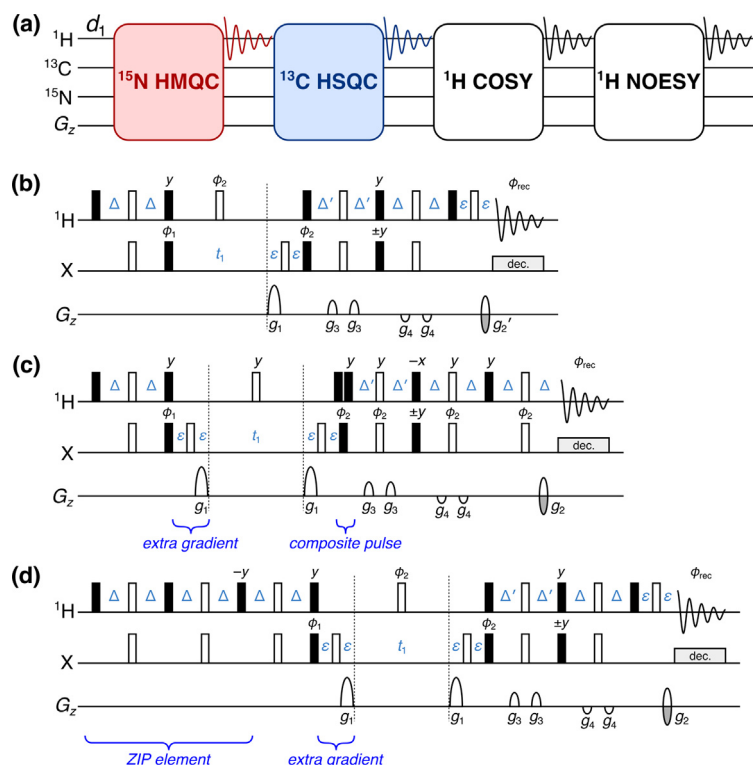
Fig. 1. (a) Overview of a typical NOAH supersequence (MSCN, using the single-letter abbreviations previously defined [44]). The {}^1\text{H} - {}^{15}\text{N} HMQC and {}^1\text{H} - {}^{13}\text{C} HSQC modules are coloured; these may be replaced with the new seHSQC module proposed in this work. (b) Cavanagh-Rance-Kay (CRK) seHSQC [58,59]. (c) Version 1 of the NOAH seHSQC module, abbreviated as “S 1 + ”. (d) Version 2 of the NOAH seHSQC module (“ZIP-seHSQC”), abbreviated as “S 2 + ”. Filled and unfilled bars represent 90° and 180° pulses respectively; all 180° pulses on {}^{13}\text{C} are adiabatic (frequency-swept) pulses. All pulses are applied along +x unless otherwise noted. Phase cycling is performed with \phi_1 = (x, -x) , \phi_2 = (x, x, -x, -x) , and \phi_{\text{rec}} = (x, -x, -x, x) . The delays are chosen as follows: \Delta = 1/(4 \cdot {}^1J_{\text{XH}}) , \Delta' = 1/(8 \cdot {}^1J_{\text{CH}}) or 1/(4 \cdot {}^1J_{\text{NH}}) , and \varepsilon is the minimum time needed for a gradient pulse and subsequent recovery. All gradient pulses are 1 ms long, except for g_1 and g_2 in {}^{15}\text{N} experiments which are 2.5 ms long. Gradient amplitudes, as percentages of maximum gradient strength (53 G/cm), are as follows: g_1 = 80\% ; g_2 = \pm 40.2\% ( {}^{13}\text{C} ) or \pm 16.2\% ( {}^{15}\text{N} ); g_2' = g_2/2 ; g_3 = 11\% ; g_4 = -5\% . The signs of g_2 and g_2' , as well as the phase of the 90° X pulse marked \pm y , are alternated within each t_1 increment to provide echo-antiecho selection. Refer to Figure S1 for product operator analysis.
