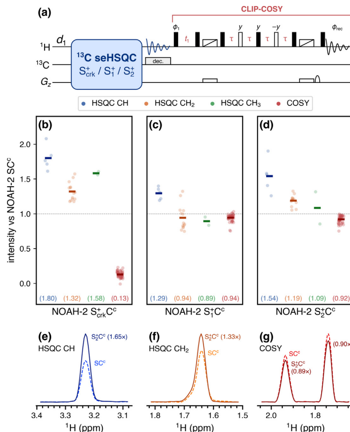
Fig. 2. Sensitivity comparisons for NOAH-2 S^+ \text{C}^{\text{C}} (seHSQC + CLIP-COSY) supersequences, using the CRK and NOAH seHSQC implementations. The delay \Delta' was set to 1/(8 \cdot ^1J_{\text{CH}}) . All intensities are normalised against the NOAH-2 \text{SC}^{\text{C}} (HSQC + CLIP-COSY) supersequence, without HSQC sensitivity enhancement. HSQC intensities are further grouped by multiplicity. Circles represent the relative intensities of individual peaks; solid bars, as well as the numbers in parentheses, indicate averages over all peaks of a given type. (a) Pulse sequence of the NOAH-2 S^+ \text{C}^{\text{C}} (seHSQC + CLIP-COSY) experiment; any of the variants shown in Fig. 1 (CRK, version 1, or version 2/“ZIP”) can be used as the seHSQC module. The CLIP-COSY [62] is performed with \phi_1 = \phi_{\text{rec}} = (x, -x) and States quadrature detection in the indirect dimension; the perfect echo mixing delay \tau is set to 8.33 ms. The unfilled rectangles with diagonal lines, applied simultaneously with z-gradients, represent frequency-swept pulses used for suppression of zero-quantum coherence [65]. (b) Using the original CRK seHSQC (Fig. 1b), which leads to severely reduced COSY intensities. (c) Using the S_1^+ module (Fig. 1c). (d) Using the S_2^+ module (Fig. 1d). (e)–(f) Slices of the NOAH HSQC (dashed line) and NOAH ZIP-seHSQC ( S_1^+ or S_2^+ ) spectra (solid line) through f_1 = 78.9 ppm (a CH peak, (e)) and f_1 = 28.5 ppm (a CH 2 peak, (f)). (g) Slices of the CLIP-COSY module from the NOAH-2 \text{SC}^{\text{C}} (dashed line) and S_2^+ \text{C}^{\text{C}} (solid line) supersequences, through f_1 = 1.36 ppm. Spectra were obtained on a 700 MHz Bruker AV III equipped with a TCI H/C/N cryoprobe; the sample used was 40 mM andrographolide in DMSO- d_6 .
