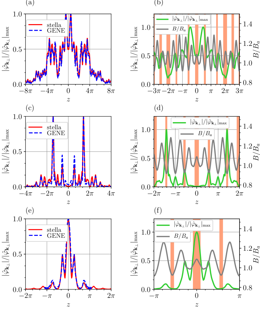
Figure 10: Normalized modulus of the electrostatic potential computed with stella (solid red line) and GENE (dashed blue line) as a function of z over the entire length of the flux tube for some modes simulated in test 3; specifically, we are representing the modes (k_x \rho_i, k_y \rho_i) = (0, 0.7) (a), (0, 1.2) (c) and (0, 4.7) (e). The structures calculated with stella are shown as solid green lines in narrower z ranges in figures (b), (d) and (f), respectively, together with the normalized magnetic field strength (grey line) and the bad curvature regions (shaded in red).
