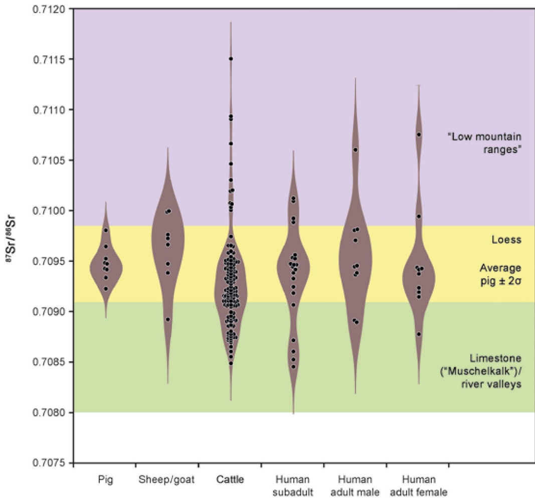
Fig. 25. Distribution of ^{87}\text{Sr}/^{86}\text{Sr} ratios of humans and domestic animals from the Bandkeramik settlement of Vaihingen an der Enz, on the basis of individual measurements and kernel density curves of value distributions. The dataset of cattle includes samples from 57 teeth and 44 individuals, while for all other groups each data point represents one tooth / individual (data: BENTLEY ET AL. 2003; 2004; KNIPPER 2011).
