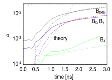
Figure 5. Magnetization level derived from the 3D PIC simulation. The magnetization is achieved up to 1% level.
