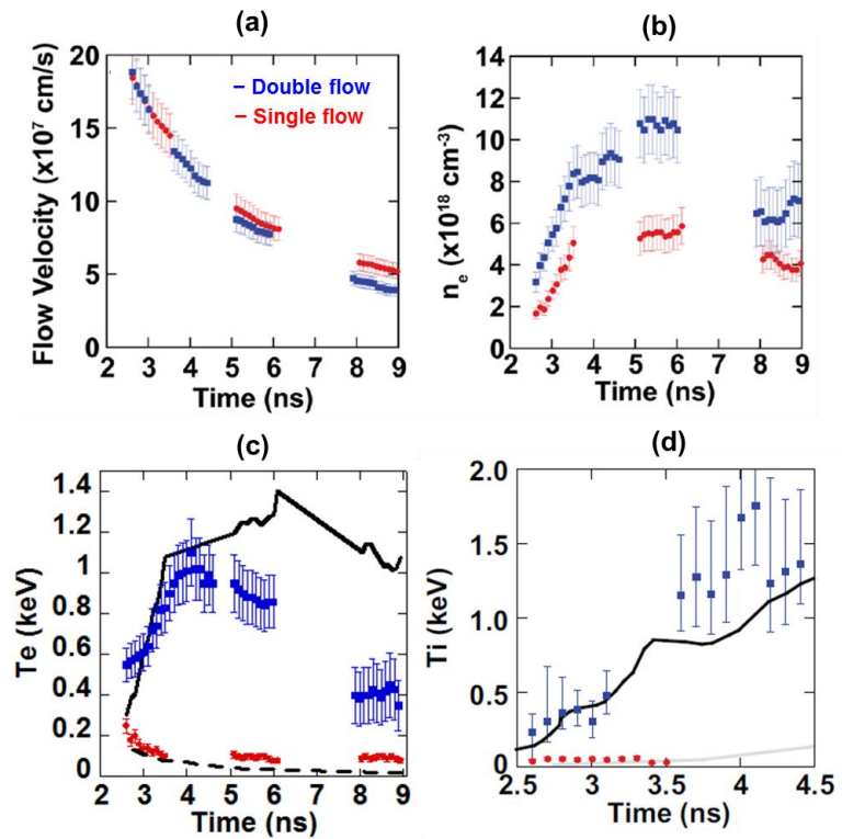
Figure 2. Omega Thomson scattering results for both single and double flows. The high increase in T_e and T_i are due to electron drag force and the electrostatic instabilities.
