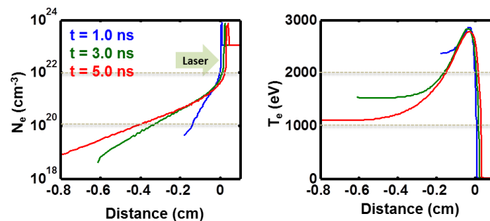
Figure 6. HYDRA simulation results for the NIF experimental condition with 100 kJ per target condition. The different color represents the pulse duration. At 5 ns setting, the N_e is \sim 10^{20} cm ^{-3} and the T_e is \sim 1 keV at 4 mm from the target surface.
