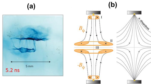
Figure 3. Omega EP short pulse generated proton image of counter-streaming plasmas at 5.2 ns after the laser. Highly stable self-organizing planar magnetic field structures are observed. This is from the Biermann battery magnetic field that is generated near the target surface; advects along the electron flows; then recompresses in the mid-plane.
