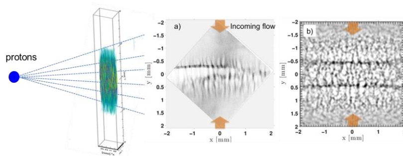
Figure 4. Schematic of proton image of D3He3 imploding capsule. (a) is the experimental data where the Weibel filamentary structures are clearly observed; (b) is the 3D Particle-in-cell simulation and the proton ray trajectory from experimental angle. The simulation also added Biermann battery field that shows as the band structure in the middle.
