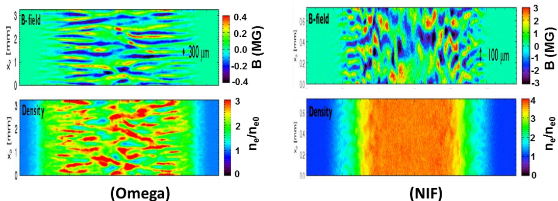
Figure 7. 3D PIC simulation results of B-field (top row) and electron density (bottom row) for Omega and NIF cases. The NIF experiments will be able to produce fully formed collisionless shocks ( n_e/n_{e0} \sim 4 ) and B field near 3 MG.
