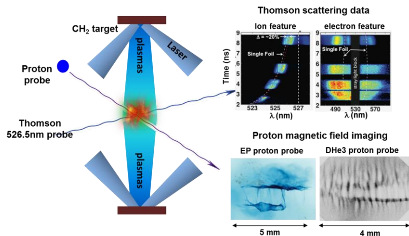
Figure 1. Schematic of Omega experiment. We use Thomson scattering to probe the plasma state and proton probe to image the magnetic field structures.
