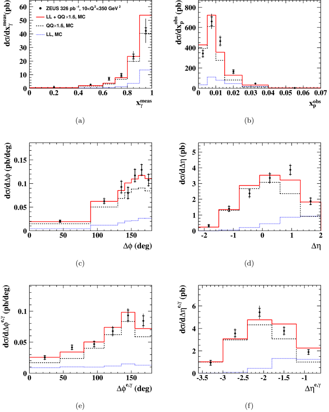
Figure 3. Differential cross sections in (a) x_\gamma^{\text{meas}} , (b) x_p^{\text{obs}} , (c) \Delta\phi , (d) \Delta\eta , (e) \Delta\phi^{e,\gamma} , and (f) \Delta\eta^{e,\gamma} , for the full range 10 < Q^2 < 350 \text{ GeV}^2 . The inner and outer error bars show, respectively, the statistical uncertainty and the statistical and systematic uncertainties added in quadrature. The solid histograms are the Monte Carlo predictions from the sum of QQ photons from PYTHIA normalised by a factor 1.6 plus DJANGOHERACLES LL photons. The dashed (dotted) lines show the QQ (LL) contributions.
