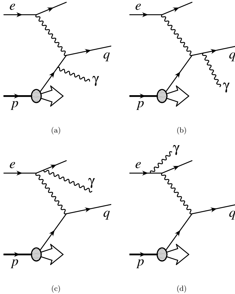
Figure 1. Lowest-order diagrams for photon production in ep scattering. (a), (b): quark radiative diagrams (QQ); (c), (d): lepton radiative diagrams (LL).
