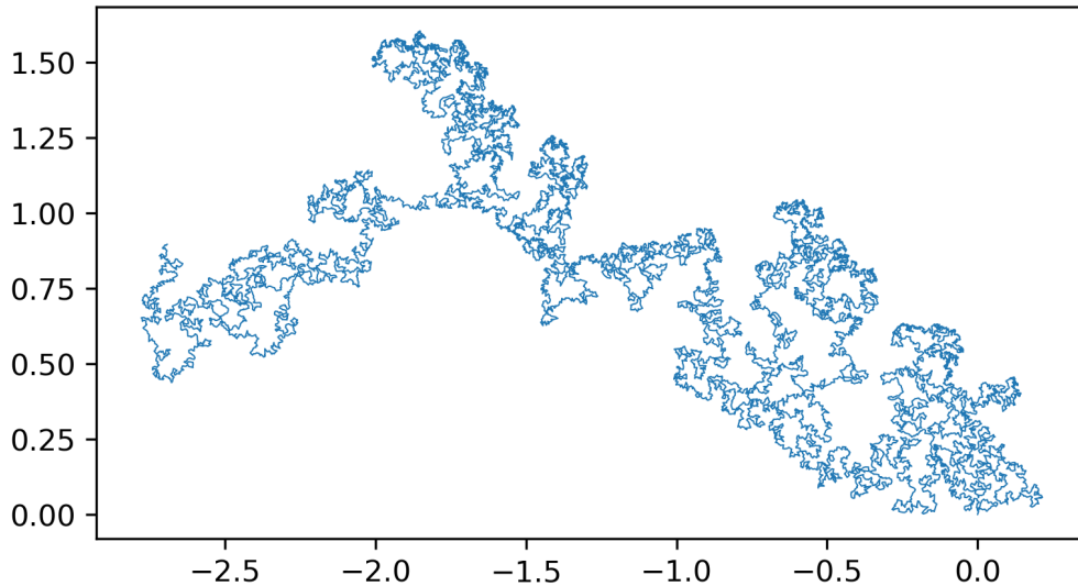
FIGURE 6.1. A sample of SLE_\kappa trace for \kappa = 6 with our method using 17884 points.
