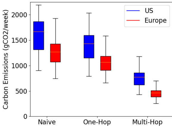
Figure 3: Carbon emissions for content delivery in the US and Europe, comparing the naive case (sending 2AM) with carbon-aware (one-hop) and carbon-intelligent (multi-hop) scheduling
