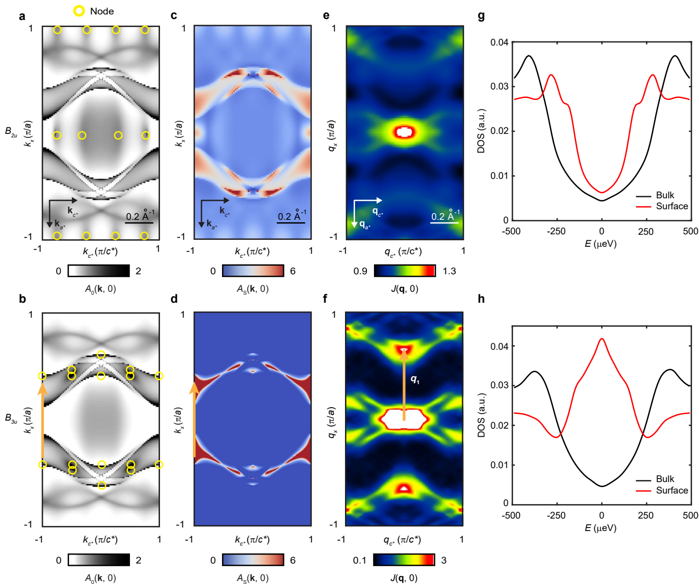
Extended Data Fig. 5 | JDOS, QPI and DOS simulations for B_{2u} and B_{3u} gap symmetry. a-b. Bulk spectral function of \text{UTe}_2 projection at the (0-11) SBZ of \text{UTe}_2 for B_{2u} and B_{3u} gap structures. c-d. Surface spectral function A_S(\mathbf{k}, 0) at the (0-11) SBZ of \text{UTe}_2 . e-f. Simulated QPI using the J(\mathbf{q}, 0) at the (0-11) SBZ of \text{UTe}_2 . g-h. Bulk and surface band DOS
