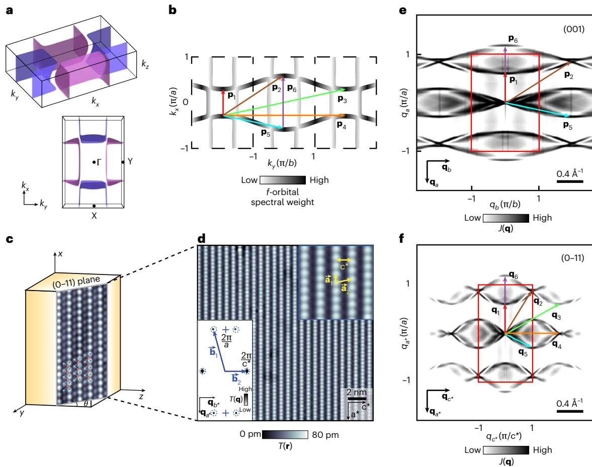
Fig. 1 | FS and QPI predictions for the (0-11) surface of UTe 2 . a , Bulk FS of UTe 2 based on recent band-structure models (Methods). b , Bulk UTe 2 FS intersecting the k_z = 0 plane. Highlighted with coloured arrows are a sextet of scattering interference wavevectors \mathbf{p}_i , i = 1-6 connecting spectral weight maxima in \mathbf{k} space derived heuristically from f -electron orbital contributions. c , Schematic of UTe 2 (0-11) cleave surface, whose normal is oriented to the crystal \mathbf{b} -axis at \theta \cong 24^\circ . Uranium (red) and two inequivalent tellurium atom sites (dark and light blue) overlaid on a T(\mathbf{r}) image, revealing the tellurium chains of the (0-11) cleave surface. d , Typical topographic image T(\mathbf{r}) of the (0-11) cleave surface of UTe 2 .
