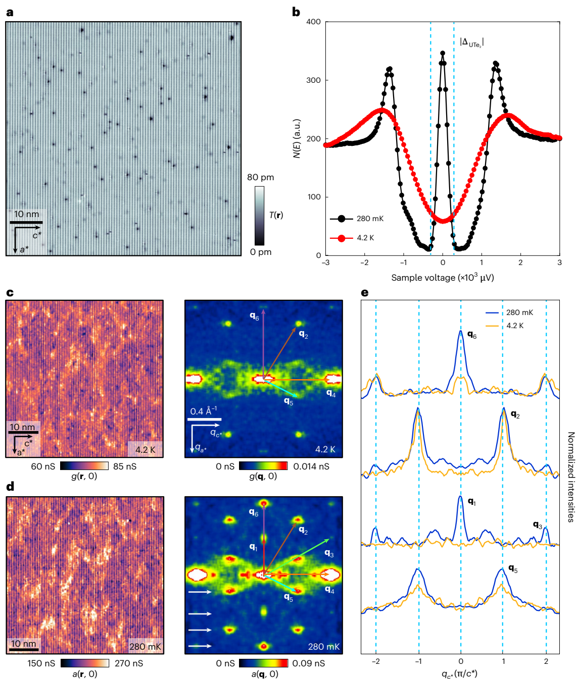
Fig. 3 | QPI visualization of UTe_2 superconductive QSB. a , Typical topographic image T(\mathbf{r}) of the (0-11) cleave surface of UTe_2 . b , Measured differential conductance in the UTe_2 normal-state g(V) at T = 4.2 K; and Andreev differential conductance in the superconducting state a(V) at T = 280 mK. Intense Andreev conductance is observed at V = 0 . c , Measured g(\mathbf{r}, 0) and g(\mathbf{q}, 0) at T = 4.2 K in the UTe_2 normal state in the identical FOV as in a . The setpoint is V_s = 3 mV and I = 200 pA. d , Measured a(\mathbf{r}, 0) and a(\mathbf{q}, 0) at T = 280 mK in the UTe_2 superconducting state in the identical FOV as in a and c . Here a sextet of scattering interference wavevectors \mathbf{q}_i , i = 1-6 from theoretical predictions are overlaid. The excellent correspondence between the predictions and the
