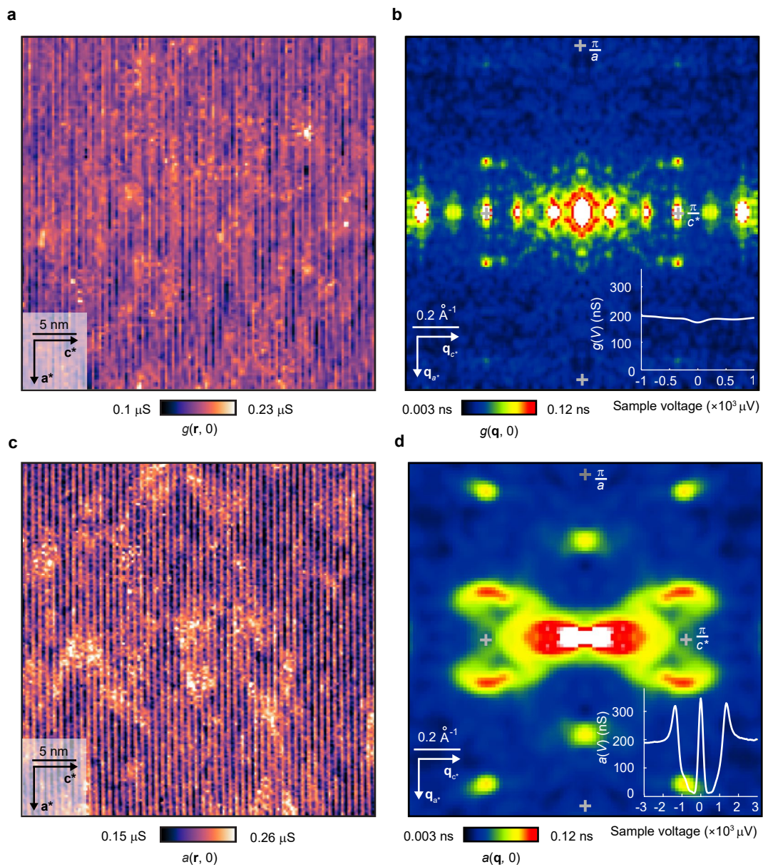
Extended Data Fig. 9 | Non-superconductive tip and superconducting tip QSB scattering interference detection. a. Measured normal-tip g(r, 0) at T = 280 mK. b. Measured normal tip g(q, 0) at T = 280 mK. Inset: Normal-tip single-electron
