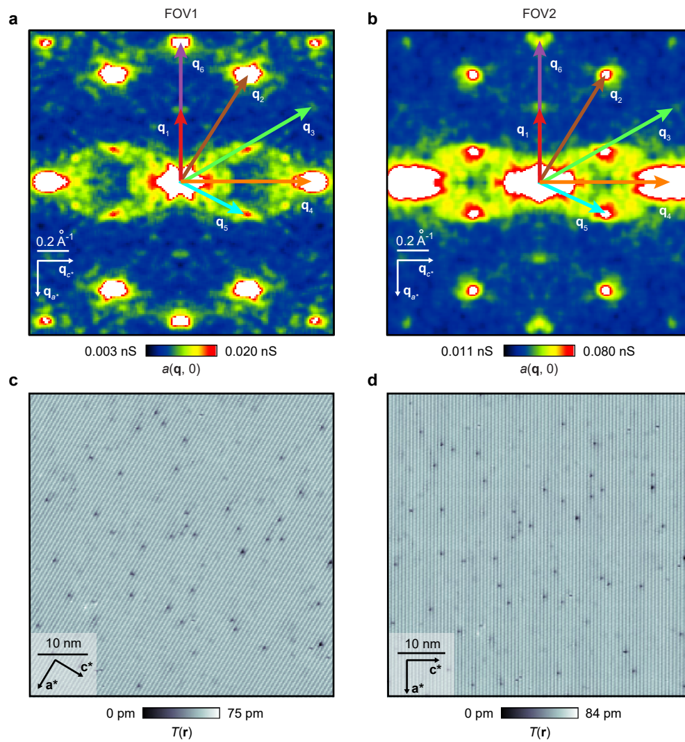
Extended Data Fig. 10 | Independent QSB QPI visualization experiments. a-b. Two independent measurements of a(\mathbf{q}, 0) at T = 280 mK confirm the repeatability of the sextet of scattering wavevectors for the B_{3d} -QSB. c-d. Topographs of areas studied in a and b , respectively.
