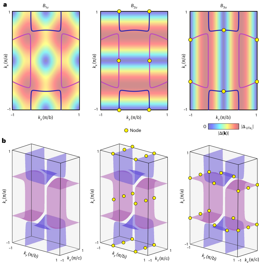
Fig. 2 | Simple models for UTe 2 Δ k . a , Magnitude of the UTe 2 superconductive energy gap |Δ k | at k z = 0 for the B 1u , B 2u and B 3u order parameters on the FS shown in Fig. 1a,b. The nodal locations occur within the dark blue regions where |Δ k | → 0. Note that B 1u does not exhibit gap nodes in this model because the FS is open along the k z axis. b , From a , the theoretically predicted nodal locations for the B 1u , B 2u and B 3u order parameters on the FS shown in Fig. 1a,b are indicated
