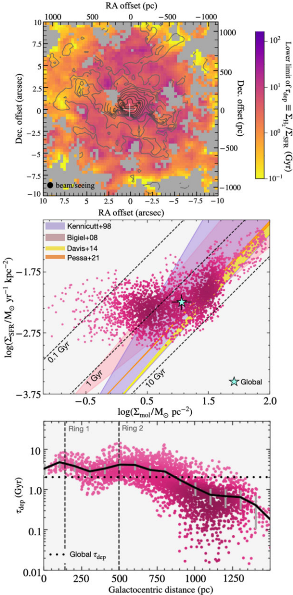
Figure 4. Top: Depletion time map of NGC 524, for all spaxels with CO and H \alpha surface brightnesses at least three times above the noise level. The extinction-corrected H \alpha surface brightness is overlaid as grey to black contours (from the 3\sigma level to the maximum). The centre of the galaxy is marked as a white cross. The synthesized beam/seeing is shown in the bottom-left corner as a solid black circle ( 1''.1 \times 1''.1 or \approx 125 \times 125 pc ^2 ). Middle: \Sigma_{\text{SFR}} - \Sigma_{\text{mol}} relation. Red data points, shaded by their density, satisfy the same criteria as the spaxels in the top panel. The cyan star shows the global \Sigma_{\text{SFR}} and \Sigma_{\text{mol}} . The purple, pink, yellow, and orange regions represent the power-law relations of Kennicutt Jr (1998), Bigiel et al. (2008), Davis et al. (2014), and Pessa et al. (2021), respectively. The black dashed diagonal lines are lines of equal depletion times (labelled). Bottom: Depletion time as a function of galactocentric distance. Red data points, shaded by their density, satisfy the same criteria as the spaxels in the top panel. The black curve shows the depletion times measured within annuli of 150 pc width, with the uncertainties shown as grey vertical bars. The black dashed vertical lines indicate the positions of the two molecular gas rings. The black dotted horizontal line indicates the global depletion time. The global molecular gas depletion time of NGC 524 is \approx 2 Gyr, but this increases to \approx 5.2 Gyr near the galaxy centre. We note that all depletion times are really lower limits, as the H \alpha emission may not arise purely from SF.
