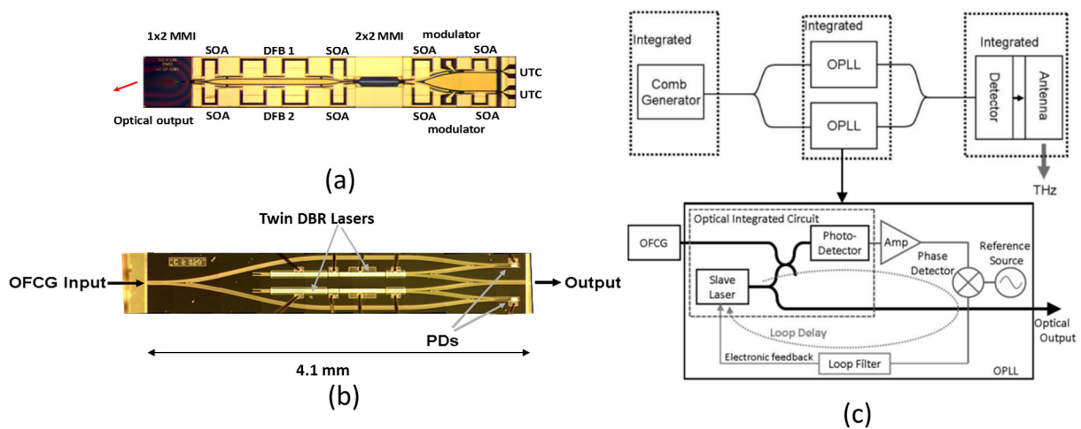
Figure 27. Microscope view of monolithic photonic integration of (a) dual DFB dual wavelength source [201] and (b) a dual OPLL [202], and (c) schematic diagram of tuneable coherent THz source. (SOA: semiconductor amplifier, DFB: distributed feedback laser, DBR: distributed Bragg reflector, OFCG: optical frequency comb, OPLL: optical phase lock loop). © 2011 IEEE. (a) © 2014 IEEE. Reprinted, with permission, from [201]. (b) and (c) reprinted with permission, from [202].
