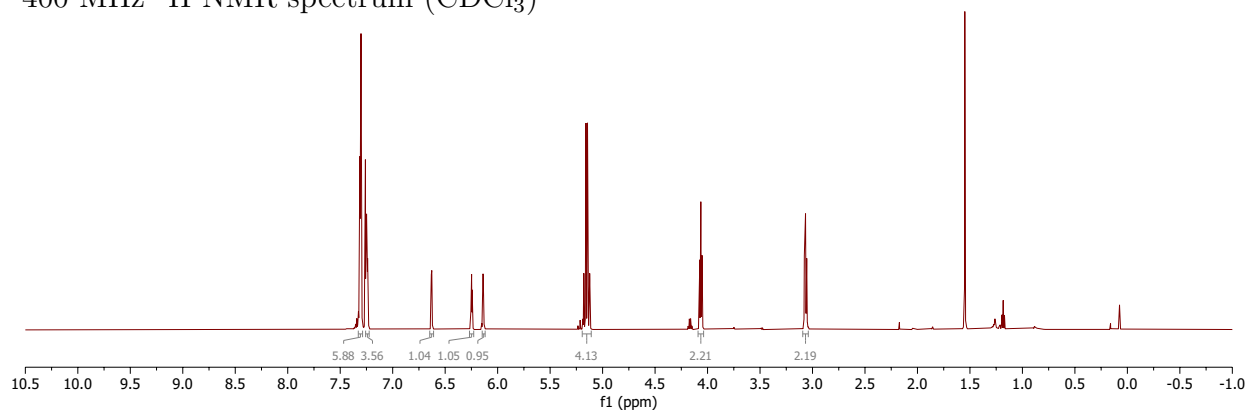
400 MHz ^1\text{H} NMR spectrum ( \text{CDCl}_3 )
