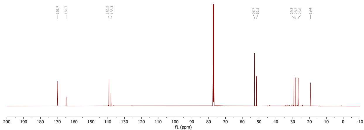
126 MHz 13 C NMR spectrum (CDCl 3 )
