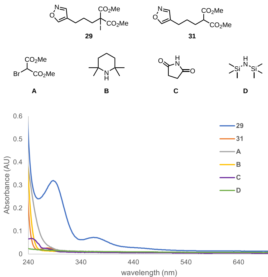
Figure 2.1. UV-VIS spectra of iodomalonnate 29 , malonnate 31 , bromomalonnate A , TMP ( B ), succinimide ( C ), and HMDS ( D ) (5 mM in THF).
