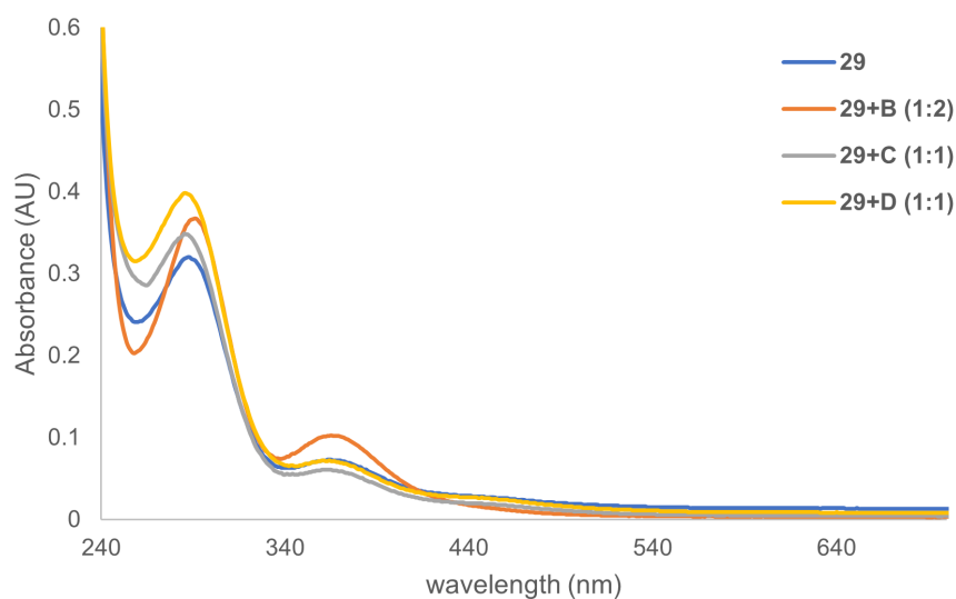
Figure 2.2. UV-VIS spectra of iodomalonnate 29 , and mixtures of iodomalonnate 29 with TMP ( B ), succinimide ( C ), and HMDS ( D ) (5 mM in THF).
