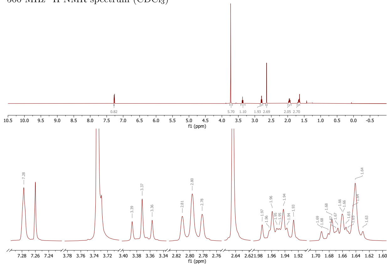
126 MHz 13 C NMR spectrum (CDCl 3 )
