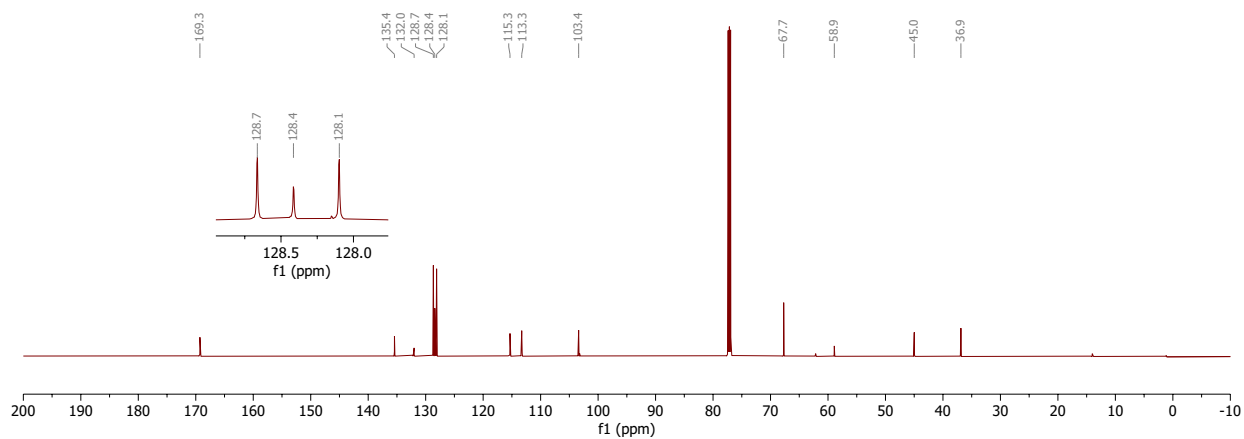
101 MHz ^{13}\text{C} NMR spectrum ( \text{CDCl}_3 )
