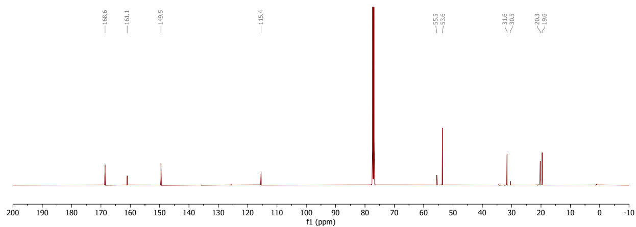
126 MHz ^{13}\text{C} NMR spectrum ( \text{CDCl}_3 )
