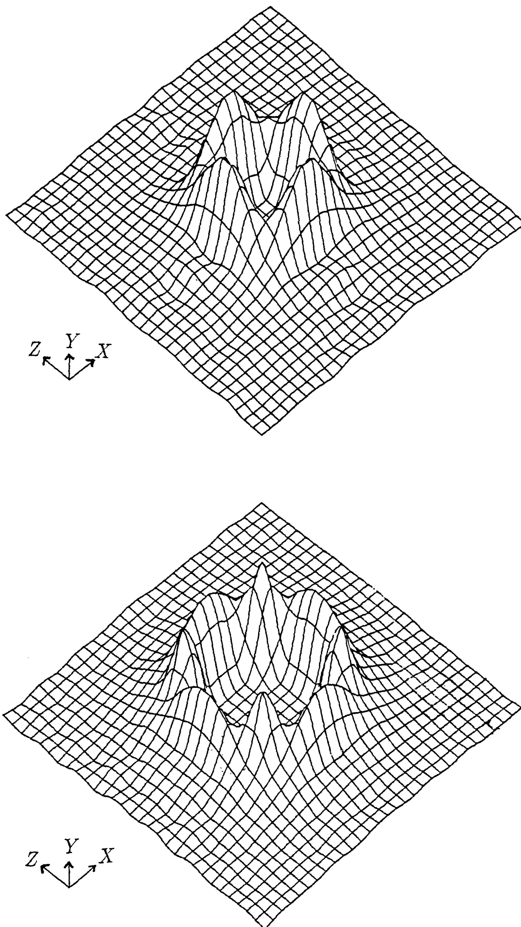
Figure 3.3: Computed free surface elevation for a three-dimensional cone Y = \epsilon R at t = 0.25 and t = 0.5 .
