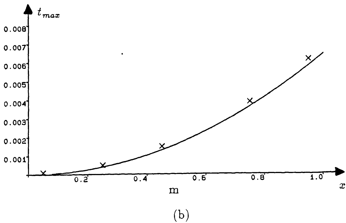
Figure 2.31: Comparison between experimental data and theory. (a) Maximum pressure in 10\text{kN/m}^2 and (b) Time to maximum pressure in seconds versus distance from the centerline in m.
