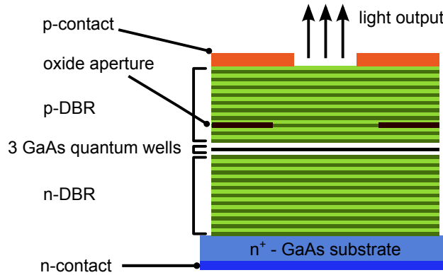
Figure 5.1: Schematic representation of the GaAs VCSEL driving the SCT opto-links.
