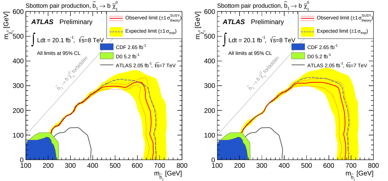
Figure 7.27: Left: Nominal exclusion in the sbottom plane using SRA signal regions only. Right: Exclusion limit obtained from a shape fit to the m_{\text{CT}} distribution.
