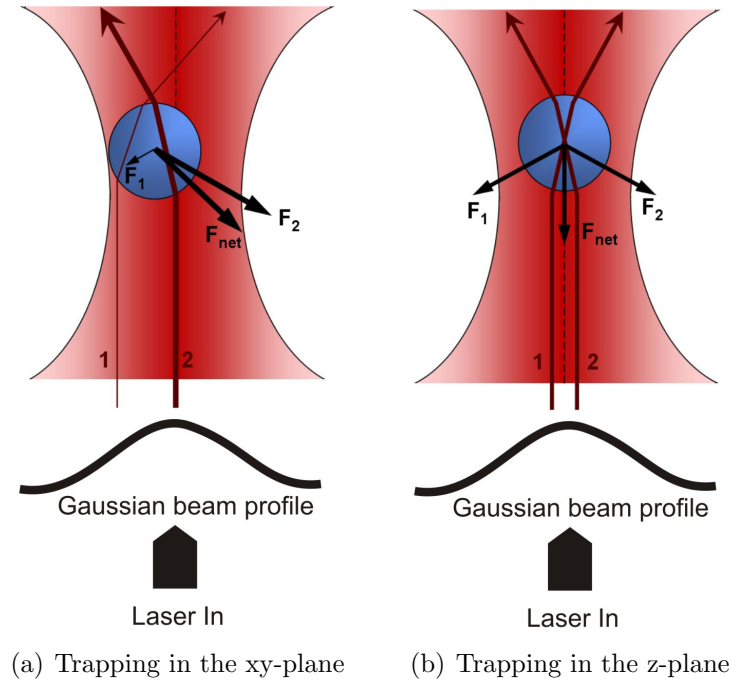
Figure 1.19: Schematics showing the principle of optical trapping using ray optics. A bead is illuminated by a Gaussian profiled laser beam. The representative laser paths are shown as red lines with arrows indicating the direction of beam propagation. The thickness of the red lines indicates the intensity of laser beam. (a) The gradient forces (black lines) are generated by the refraction of the beam when they interact with the particle, resulting in a change of photon momentum which is transferred on to the particle, thus generating the forces F_1 and F_2 . As more photons follow path 2 than 1 (because the beam intensity is higher along the former), force F_2 is stronger than F_1 . Consequently, the net gradient force ( F_{net} ) in the lateral direction directs the particle to centre of the beam, keeping it trapped in the same position in x and y . (b) To achieve a three-dimensional trap, the scattering force needs to be compensated as well. This is achieved by sharply focussing the laser thus generating an axial gradient force towards this region when the particle is in its vicinity. The scattering force (not shown) is in the direction of propagation of the laser beam (i.e. upward in this figure) and is proportional to the intensity of the beam. The bead is trapped slightly beyond the focused spot where the gradient force and scattering force are in equilibrium in the z -plane.
