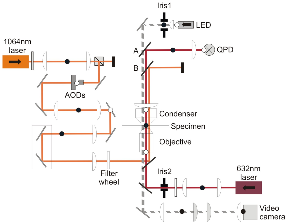
Figure 2.4: Layout of the optical trap used in these experiments (adapted from [94]).
