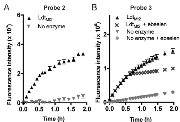
Figure 1. An increase in fluorescence intensity is observed on addition of fluorogenic probes 2 and 3 to Ldt Mt2 . A) Probe 2 ( \lambda_{\text{ex}} = 480 nm, \lambda_{\text{em}} = 555 nm) could be used at a concentration of 25 \mu\text{M} with 1 \mu\text{M} Ldt Mt2 to provide a sufficient level of fluorescent signal. B) Probe 3 (25 \mu\text{M} ; \lambda_{\text{ex}} = 480 nm, \lambda_{\text{em}} = 520 nm) showed better sensitivity than 2 , and provided a sufficient fluorescent signal with 100 nM Ldt Mt2 . The reaction between Ldt Mt2 and 3 was quenched after 30 min by the addition of ebselen to allow for high-throughput screening. Experiments with probe 2 were carried out in 50 mM sodium phosphate, pH 8.0, 0.01 % Triton X-100, and those with probe 3 were in 50 mM HEPES, pH 7.2, 0.01 % Triton X-100. Data points represent the mean, and error bars represent the standard deviation ( n = 96 ).
