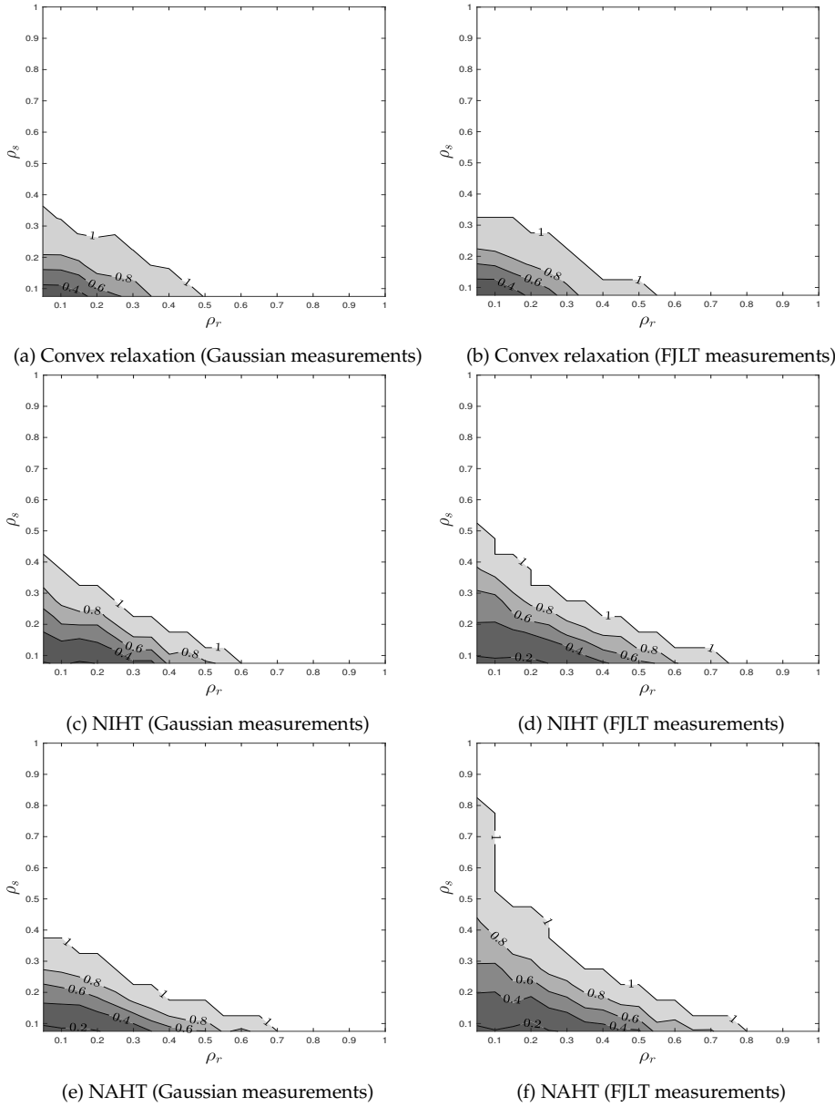
Figure 4.4: Phase transition level curves denoting the value of \delta^* for which values of \rho_r and \rho_s below which are recovered for at least 5 out of 10 experiments for \delta , \rho_r , and \rho_s as given by (4.110). The convex optimization problem is solved by SDPT3 (Toh et al., 1999). NIHT and NAHT are observed to recover matrices of higher ranks and sparsities compared to solving the convex relaxation.
