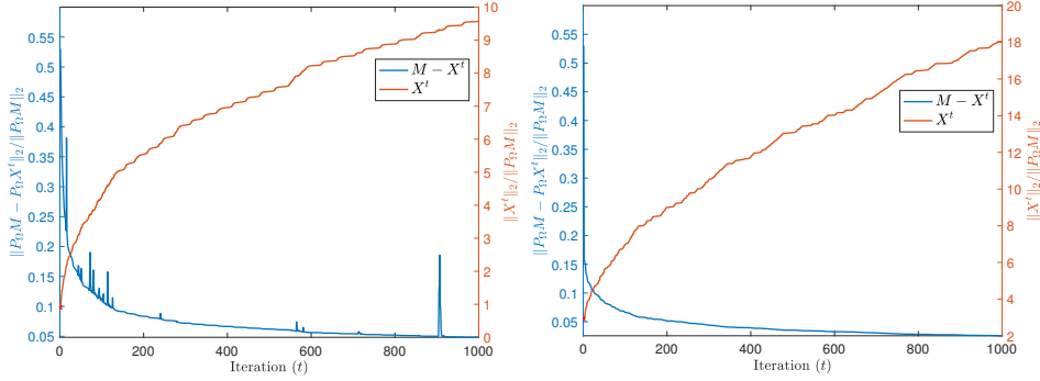
(c) CGIHT with restarts (Blanchard et al., 2015) applied to M^{(1)} . (d) ASD (Tanner and Wei, 2016) applied to M^{(1)} .
