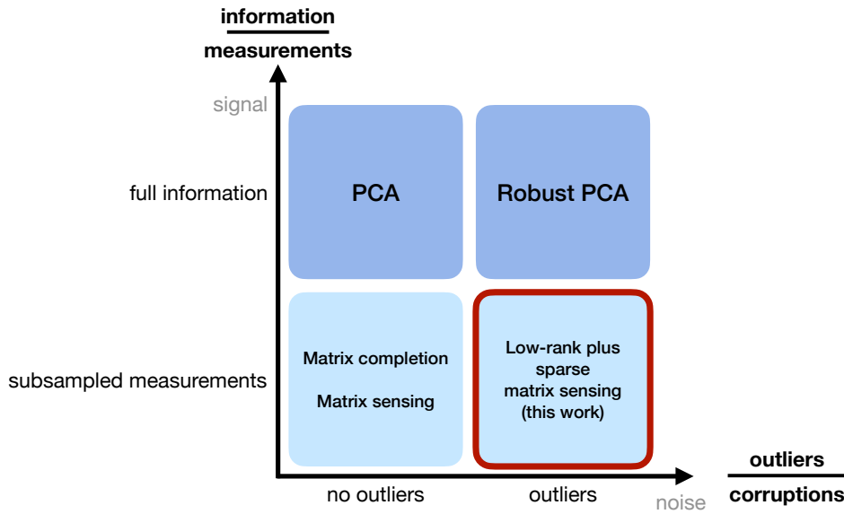
Figure 1.1: Schematic diagram that outlines the different problems based on low-rank matrix approximation. The main problem which is considered in this work is annotated in red.
