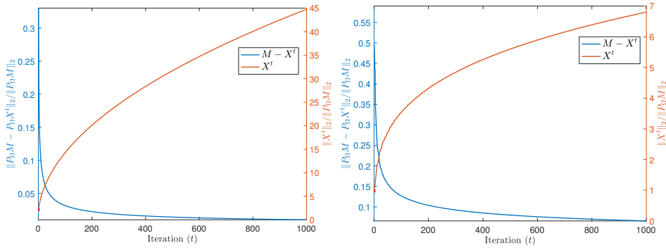
(a) PF (Haldar and Hernando, 2009) applied to M^{(1)} . (b) LMaFit (Wen et al., 2012) applied to M^{(1)} .
