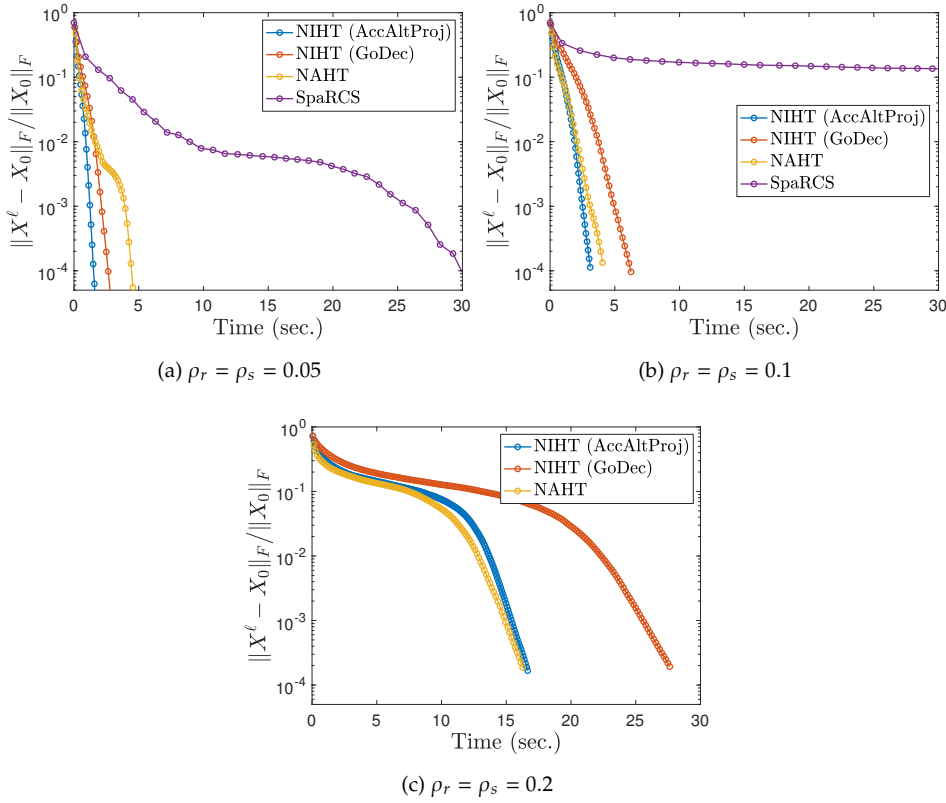
Figure 4.2: Relative error in the approximate X^\ell as a function of time for synthetic problems with m = n = 100 and p = (1/2)100^2 , \delta = 1/2 , for Gaussian linear measurements \mathcal{A} . In (b), SpaRCS converged in 171 sec. (45 iterations), and in (c), SpaRCS did not converge.
