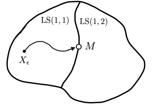
Sequence X_\varepsilon converges outside of the feasible set \text{LS}_{3,3}(1, 1) .
