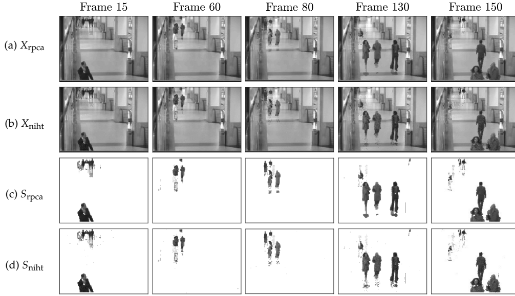
Figure 4.5: NIHT recovery results of a 190 \times 140 \times 150 video sequence compared to the approximation of the complete video sequence by Robust PCA (AccAltProj (Cai et al., 2019)). The video sequence is reshaped into a 26\,600 \times 150 matrix and either recovered from FJLT measurements with \delta = 0.33 using rank r = 1 and sparsity s = 197\,505 or approximated from the full video sequence by computing RPCA by AccAltProj with the same rank and sparsity parameters. Recovery by NIHT from subsampled information achieves PSNR of 34.5 dB whereas the Robust PCA approximation from the full video sequence achieves PSNR of 35.5 dB.
