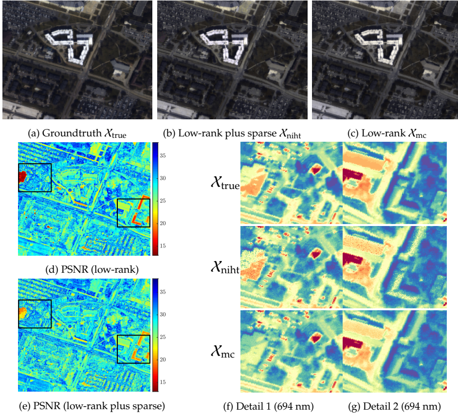
Figure 4.6: Recovery by NIHT from FJLT measurements with \delta = 0.33 using low-rank model ( \rho_r = 0.25, \rho_s = 0 ) compared to the low-rank plus sparse model ( \rho_r = 0.25, \rho_s = 0.05 ). Figure 4.6a - 4.6b show the color renderings of the original multispectral image and the two recovered images. Figure 4.6d and Figure 4.6e show the spatial PSNR of the recovery from the low-rank only model (overall PSNR of 38.9 dB) and the low-rank plus sparse model (overall PSNR of 39.1 dB) respectively. Figure 4.6f and Figure 4.6g show two details of size 128 \times 128 in the 694 nm band.
