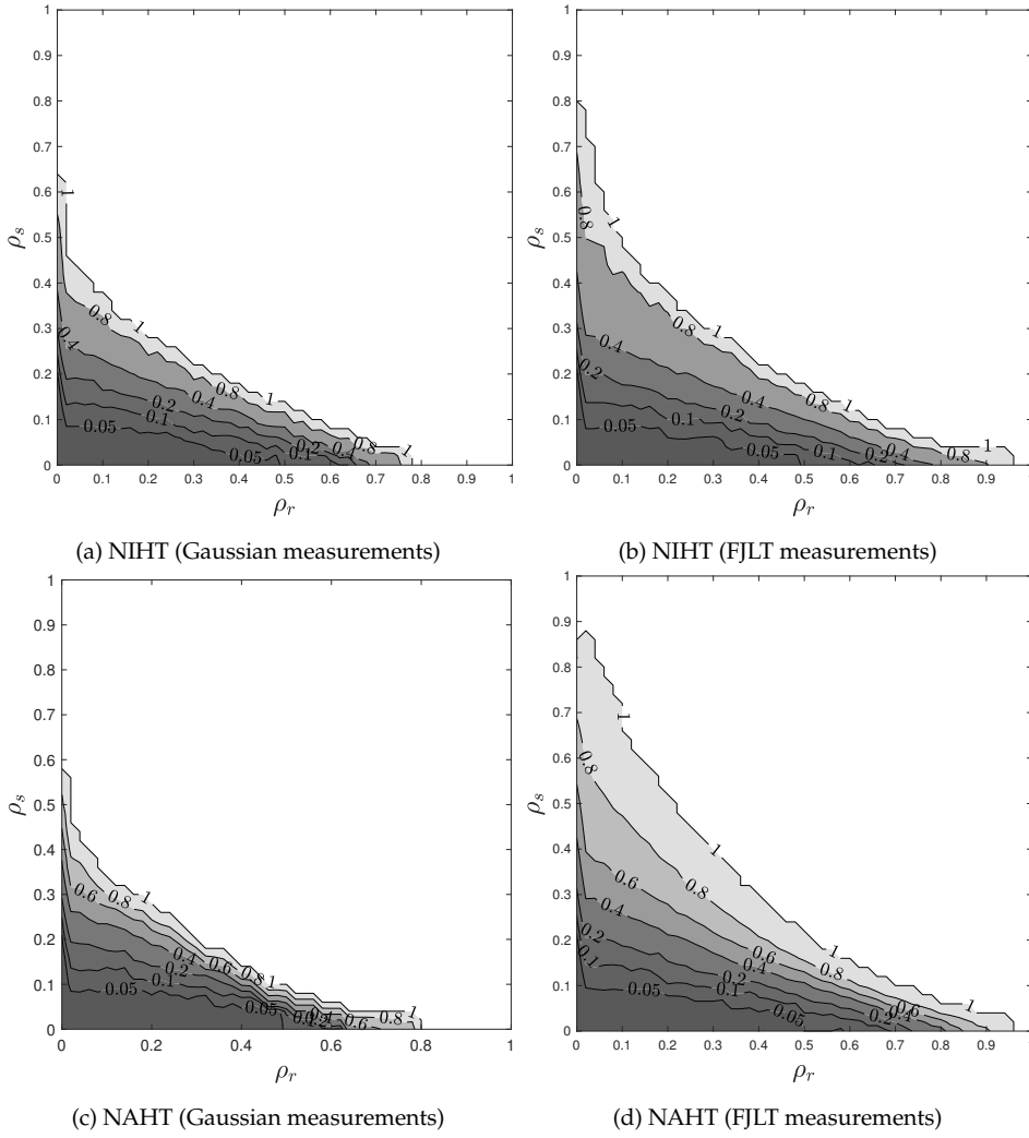
Figure 4.1: Phase transition level curves denoting the value of \delta^* for which values of \rho_r and \rho_s below which are recovered for at least half of the experiments for \delta , \rho_r , and \rho_s as given by (4.110). NIHT is observed to recover matrices of higher ranks and sparsities from FJLT than from Gaussian measurements, while the phase transitions for NIHT and NAHT are comparable. The RPCA projection in NIHT, step 5 in Alg. 1, is performed by AccAlt-Proj (Cai et al., 2019).
