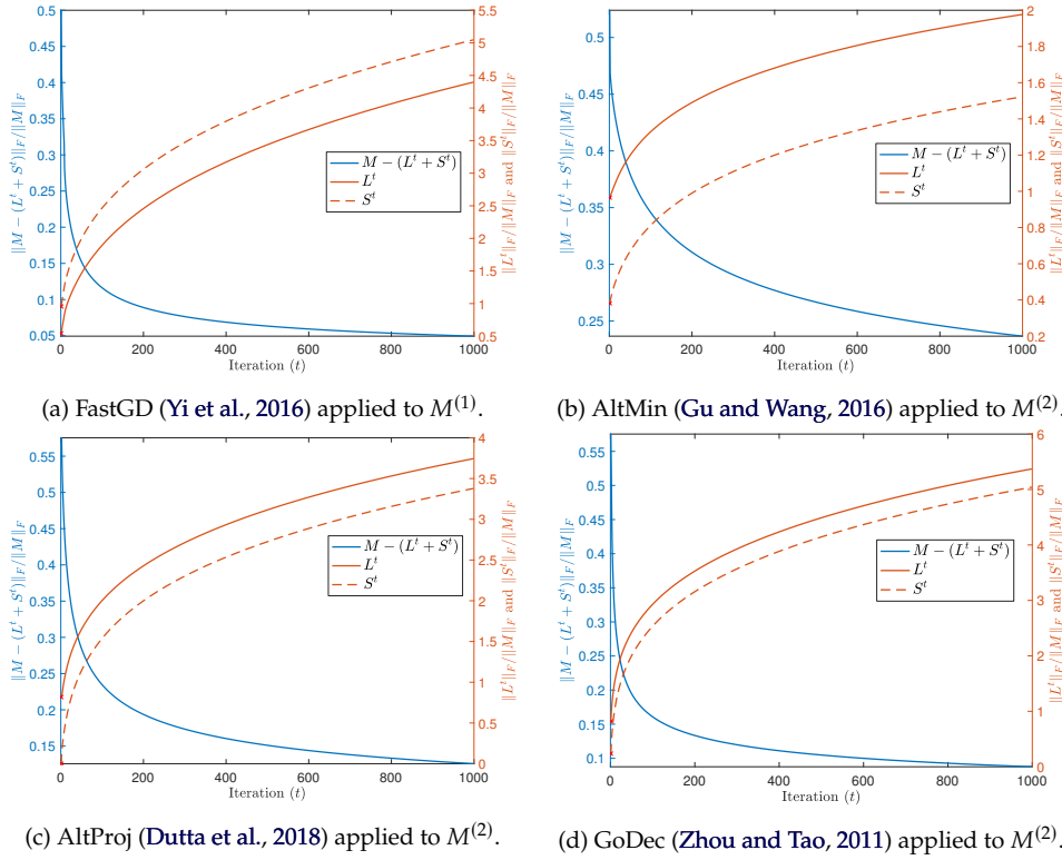
Figure 2.1: Solving for an \text{LS}_{3,3}(1,1) approximation to M^{(1)} and M^{(2)} using four non-convex Robust PCA algorithms. Despite the norm of the residual \|M - (L^t + S^t)\|_F converging to zero, norms of the constituents L^t, S^t diverge. We set algorithms parameters r = 1, s = 1 where possible. For FastGD we set \lambda = 3.23 and stepsize \eta = 1/6 which corresponds to choosing s = 1 . For GoDec we set the low-rank projection precision parameter to be 10.
