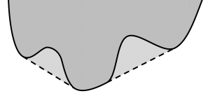
The convex envelope of a non-convex function.
