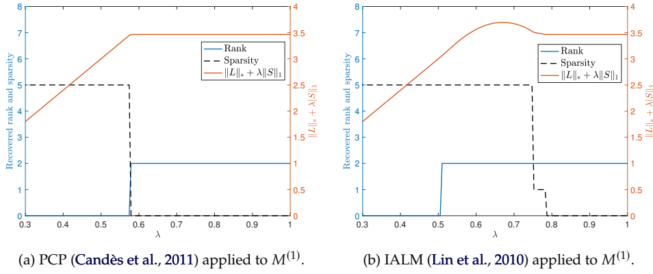
Figure 2.2: Recovered ranks and sparsities using two convex Robust PCA algorithms applied to M^{(1)} with varying choice of \lambda . Both PCP and IALM do not recover the r = 1, s = 1 solution for any \lambda . IALM recovers solutions with overspecified degrees of freedom r = 2, s = 5 for \lambda roughly 1/2 .
