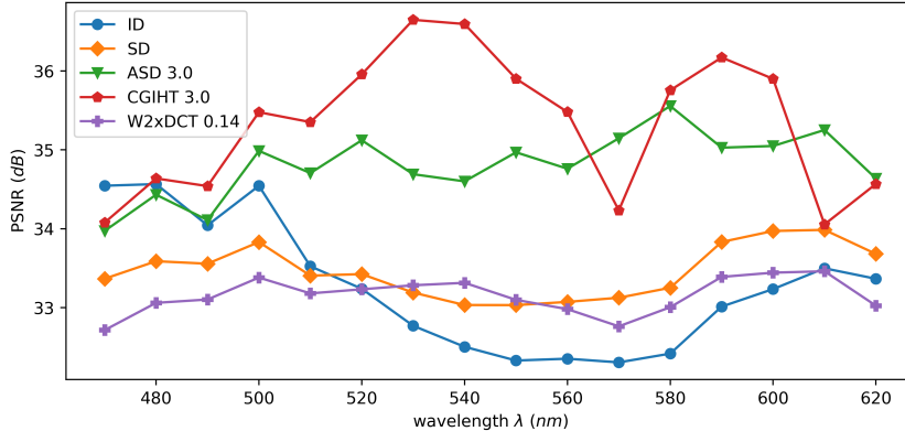
(a) PSNR throughout spectral bands.
