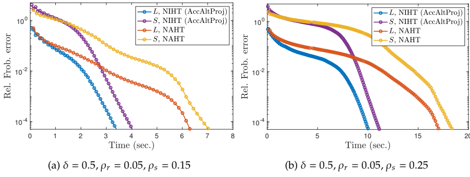
Figure 4.3: Error between the approximate recovered low-rank and sparse components L^\ell and S^\ell and the true low-rank and sparse components L_0 and S_0 . Error is plotted as a function of recovery time for synthetic problems with m = n = 100 and p = (1/2)100^2 , \delta = 1/2 , for Gaussian linear measurements \mathcal{A} .
