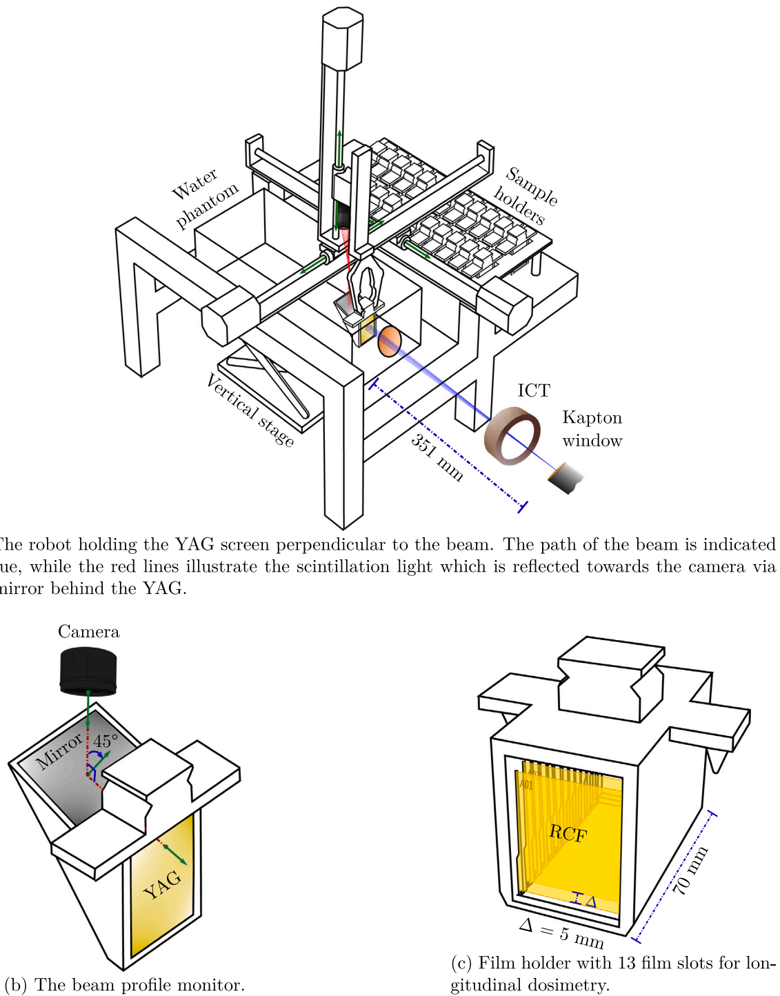
Fig. 3. Drawings of the robotic sample handling system and the 3D printed sample holders.
