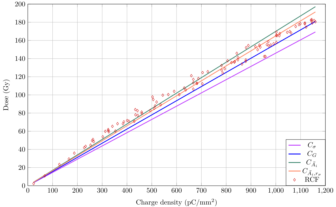
Fig. 7. Predicted doses using the calibration factors C_G , C_{A_i} , C_{A_i, r_σ} and C_σ on the circles A_i in Fig. 6(a). The corresponding measured doses from Fig. 6(b) are shown in red.
