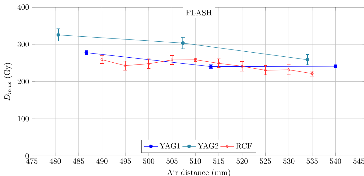
Fig. 13. The longitudinal evolution of the predicted and measured peak doses in FLASH conditions.
