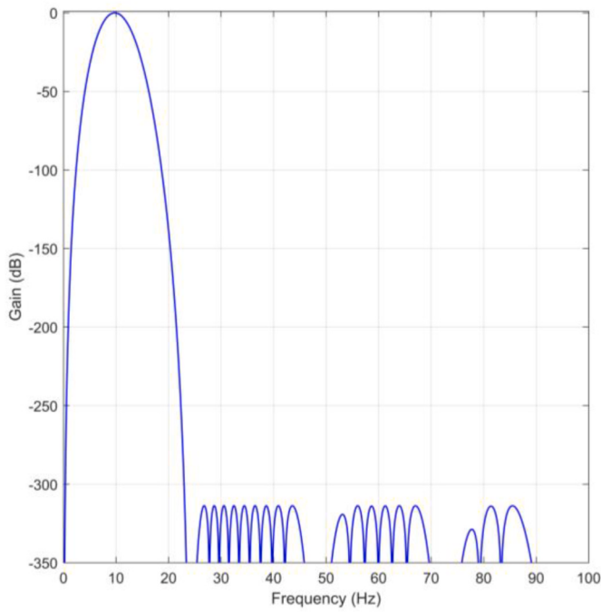
Fig. 4. Prism low pass filter.
