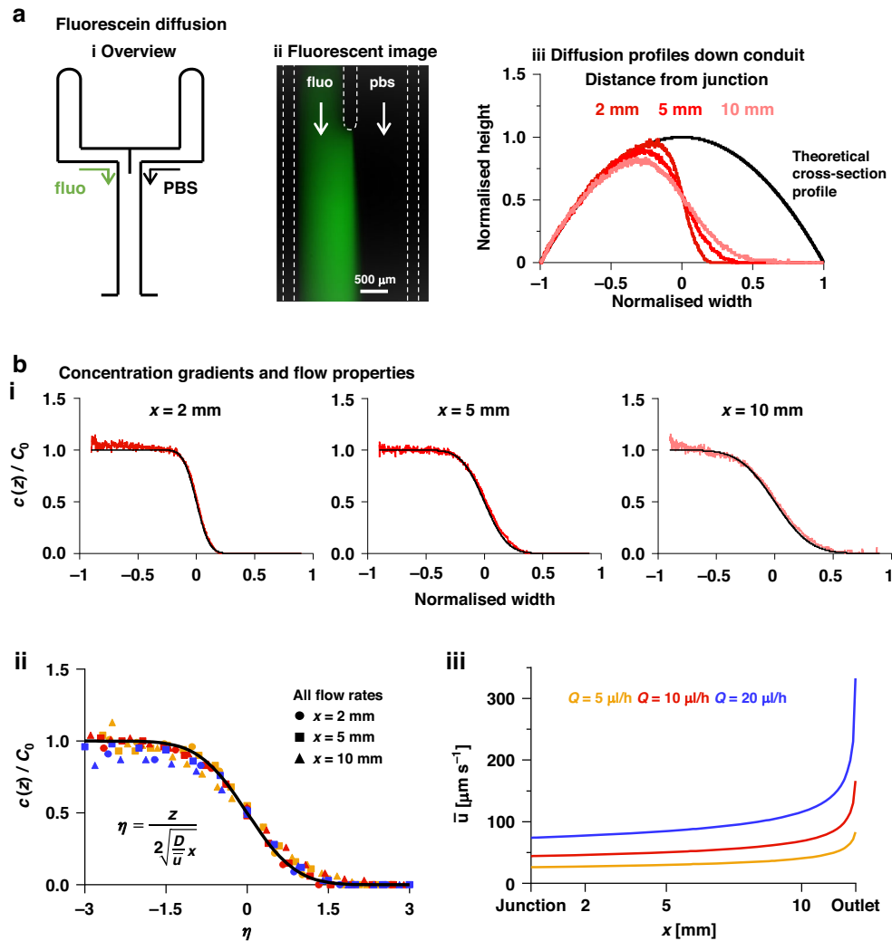
Fig. 4 Diffusion of fluorescein from one laminar stream into a fluorescein-free stream flowing at the same rate. a Overview. (i) Schematic. PBS-fluorescein (fluo) is inputted into the left-hand arm, and PBS into the right-hand one ( Q = 10 \mu\text{l/h} ; q_A = q_B ). (ii) Representative fluorescent image of the junction. Dashed lines mark fluid walls pinned to the dish. (iii) Diffusion profiles across the central conduit at positions 2, 5, and 10 mm from the junction. For each distance from the junction, there is one black curve (derived using Eq. 1) plus an associated red curve (derived from intensities measured in images like that in (A)ii, and then converted to equivalent heights using the calibration factor). Pairs of curves are overlaid by normalising widths and heights with respect to h_0 on each black curve. b Concentration gradients and flow properties. (i) Concentration profiles (red) measured 2, 5, and 10 mm from the junction compared to predictions from Eq. (7) (black line). Experimental gradients are computed as the ratio of a diffusion profile (shown in Aiii) and the corresponding cross-section profile at each point across the width. (ii) Collapsed experimental data for all flow rates tested (for \eta see Eq. (7); colours refer to flow rates and shapes of data points indicate distances from the junction) and predicted curve from Eq. (7) (black line). (iii) Mean velocities in the centre of the conduit for different flow rates (from Eq. (3))
