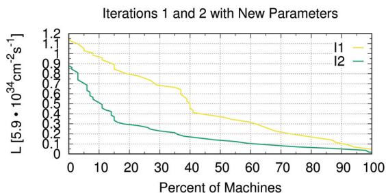
Figure 5: Comparison of iterations 1 and 2 using the new weighting parameters.
