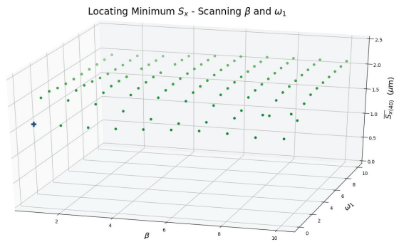
Figure 2: \beta vs. \omega_1 vs. horizontal beam size averaged over 40 seeds. Minimum indicated by blue cross.
