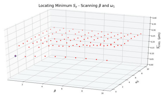
Figure 3: \beta vs. \omega_1 vs. vertical beam size averaged over 40 seeds. Minimum indicated by blue cross.
