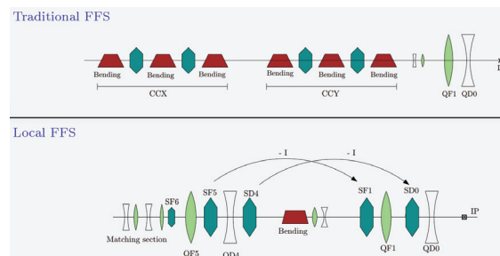
Figure 1: General layouts of two FFS systems [3].
