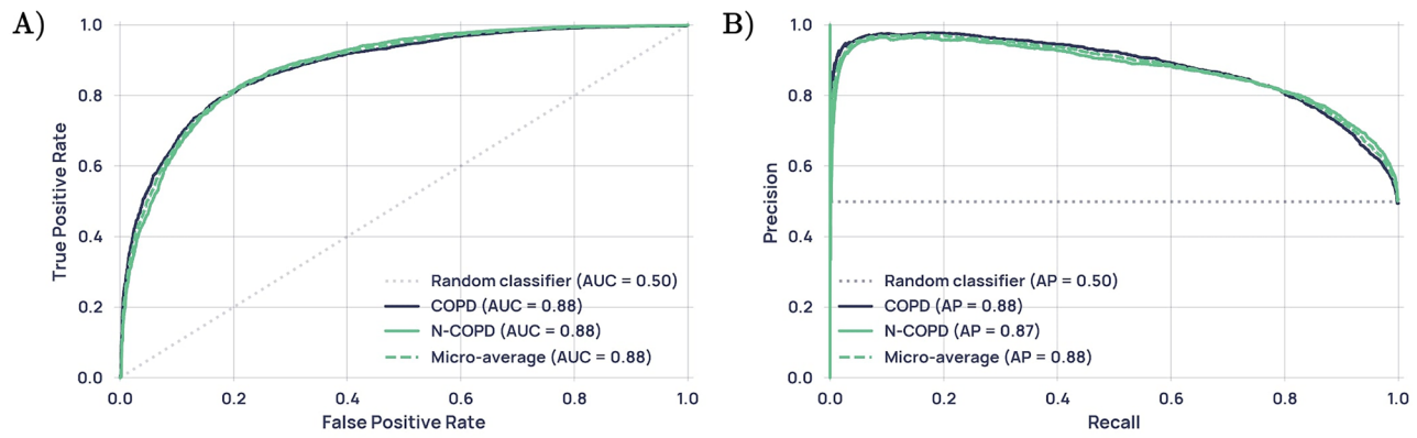
Figure 3. (A) Receiver operating characteristic (ROC) curve for the LR model, reported with results of a theoretical ‘random’ classifier with no predictive power. (B) Precision-Recall Curve for the LR model, reported with the results of a theoretical ‘random classifier’ and the average precision (AP).
