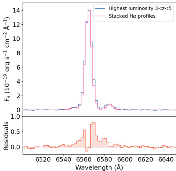
Figure B2. The true stack (blue) of the highest luminosity sources in our sample at z = 3\text{--}5 compared to the stack of the observed H\alpha profiles (pink). The bottom panel shows the residuals between the true stack and the stacked H\alpha profiles.
