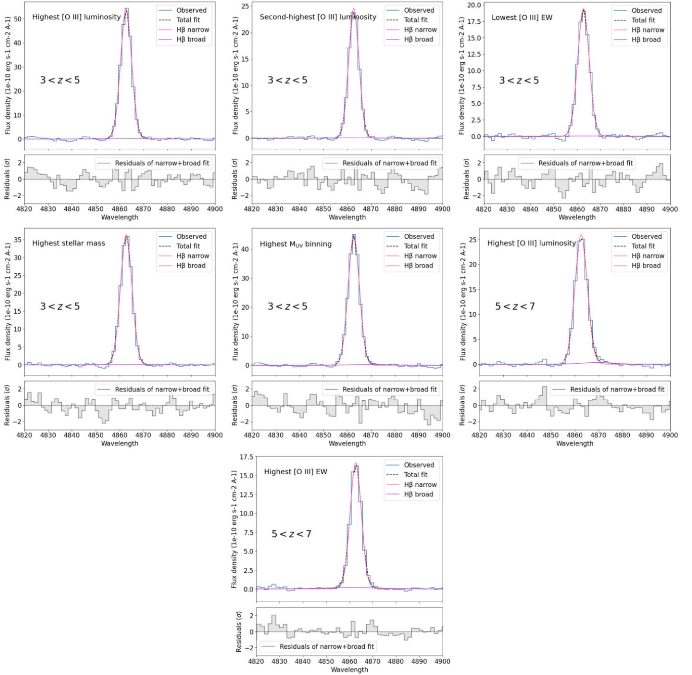
Figure F1. The results of fitting a broad component to H\beta in the stacks where we have detected AGN activity. Left to right and top to bottom: highest luminosity 3 < z < 5 ( \Delta BIC = -14.15 ), second-highest luminosity 3 < z < 5 ( \Delta BIC = -15.26 ), lowest EW 3 < z < 5 ( \Delta BIC = -15.28 ), highest stellar mass 3 < z < 5 ( \Delta BIC = -15.77 ), highest M_{UV} 3 < z < 5 ( \Delta BIC = -12 ), highest luminosity 5 < z < 7 ( \Delta BIC = -6.57 ), highest EW 5 < z < 7 ( \Delta BIC = -12.16 ). All values of \Delta BIC are in favour of a narrow only model.
