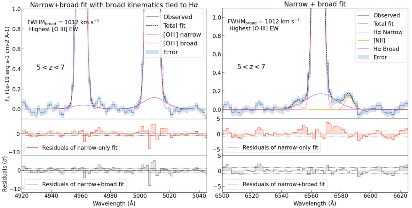
Figure 6. Same as Fig. 5, but for the stack in the redshift range 5 < z < 7 and highest EW([O III]) bin. Also in this case the FWHM of the H \alpha broad component that provides a good fit is \gtrsim 1000 \text{ km s}^{-1} , supporting the BLR hypothesis. The same broad component is not required by the [O III] as indicated by the residuals and, most importantly, as indicated by the \Delta BIC , which favours a much narrower broad component for [O III] (see Table 2).
