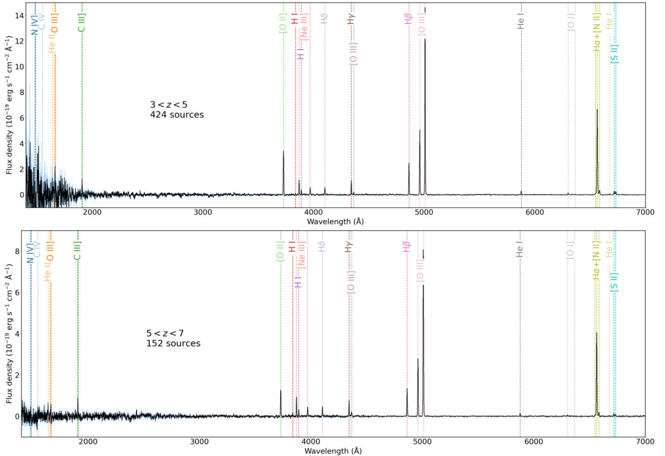
Figure 1. Stacked spectra of our sample of medium-resolution JADES galaxies that have not been previously identified as AGNs at 3 < z < 5 (top) and 5 < z < 7 (bottom). These are mean stacks with no weighting or normalization. The 3 < z < 5 stack contains 424 sources and the 5 < z < 7 stack contains 152 sources. The shaded region indicates the errors of the stack.
