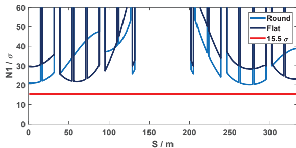
Figure 6: BSC in triplet for flat and round collision optics.
