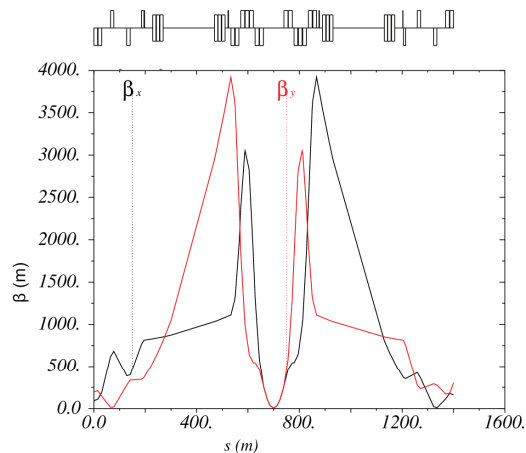
Figure 7: Optics for 6 \text{ m } \beta^* injection optics with 40 \text{ m } L^* .
