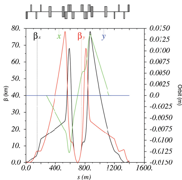
Figure 1: \beta functions and orbit for 0.3 m \beta^* collision optics with alternative triplet and 45 m L^* .
