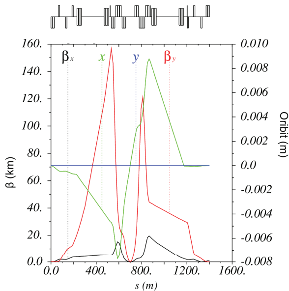
Figure 5: \beta functions and orbit for 1.2 \times 0.15 m flat collision optics with alternative triplet and 40 \text{ m } L^* .
