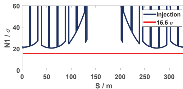
Figure 8: BSC in triplet for 6 \text{ m } \beta^* at an injection energy of 1.3 \text{ TeV} .
