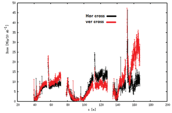
Figure 3: Triplet radiation studies for round collision optics with 40 m L^* .
