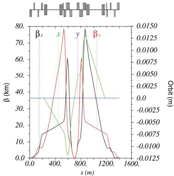
Figure 2: \beta functions and orbit for 0.3 m \beta^* collision optics with alternative triplet and 40 m L^* .
