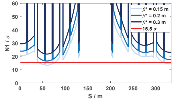
Figure 4: BSC in triplet for various \beta^* optics options.
