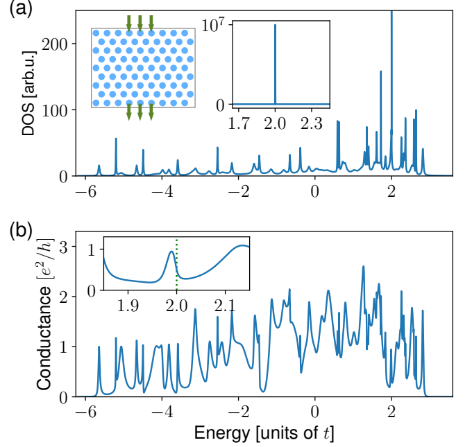
FIG. 3. (a) DOS of a 9 \times 9 square with connections to fibers on three sites at the top and bottom boundaries as shown in the left inset. The right inset shows the DOS divergence close to E_{\text{VH}} = 2t . (b) Transmittance of the same system, normalized to the input flux on a single fiber. The inset highlights the absence of resonant transmission features at E_{\text{VH}} .
