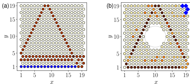
FIG. 4. Examples of VH lattice scars. The intensity of red color is proportional to the probability density at each lattice site (circles) after a long time evolution of a Gaussian wavepacket, subject to localized losses at the sites marked by blue diamonds. (a) 19 \times 19 square triangular lattice with losses in the 17 bottom-left sites. (b) 19 \times 19 Sinai triangular lattice with losses in 4 sites in the upper right corner. The dimensions of the VHD for each closed system are (a) n_{\text{VH}} = 18 and (b) 5; only one BIC remains in each system after coupling to the environment.
