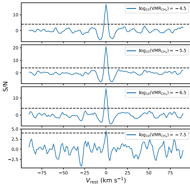
Figure 5. Injected CCFs (CCF injection ) of pure CH 4 models at the atmospheric adiabatic limit, at varying abundances, into the L -band data. The CCFs have been sliced at the injected velocity of K_p = 146 \text{ km s}^{-1} . The black dashed lines indicate a detection level of S/N = 4 .
