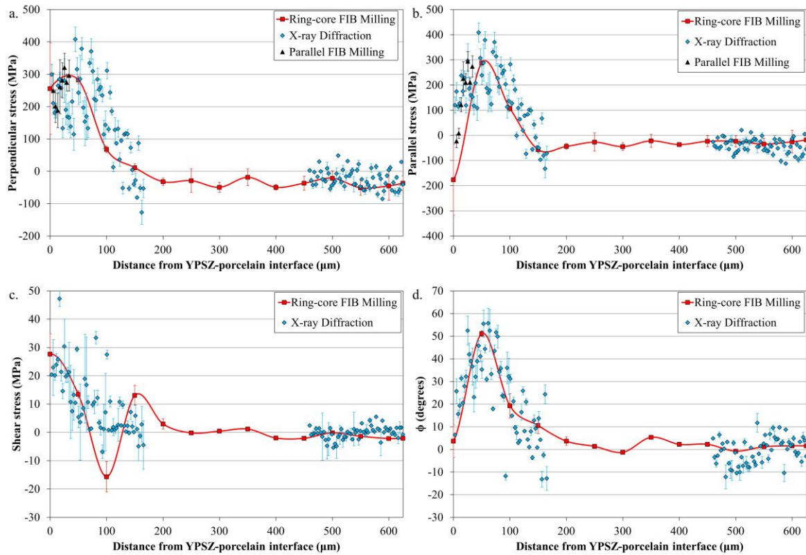
Figure 6.10. Residual stress in YPSZ as a function of distance from the YPSZ-porcelain interface.
