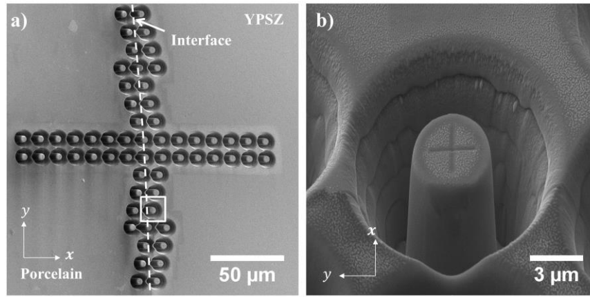
Figure 7.14. a) Positions of FIB milled micropillars across the YPSZ-Porcelain interface. b) A high magnification image of one pillar. Both images were captured at tilt of 55° in the x direction.
