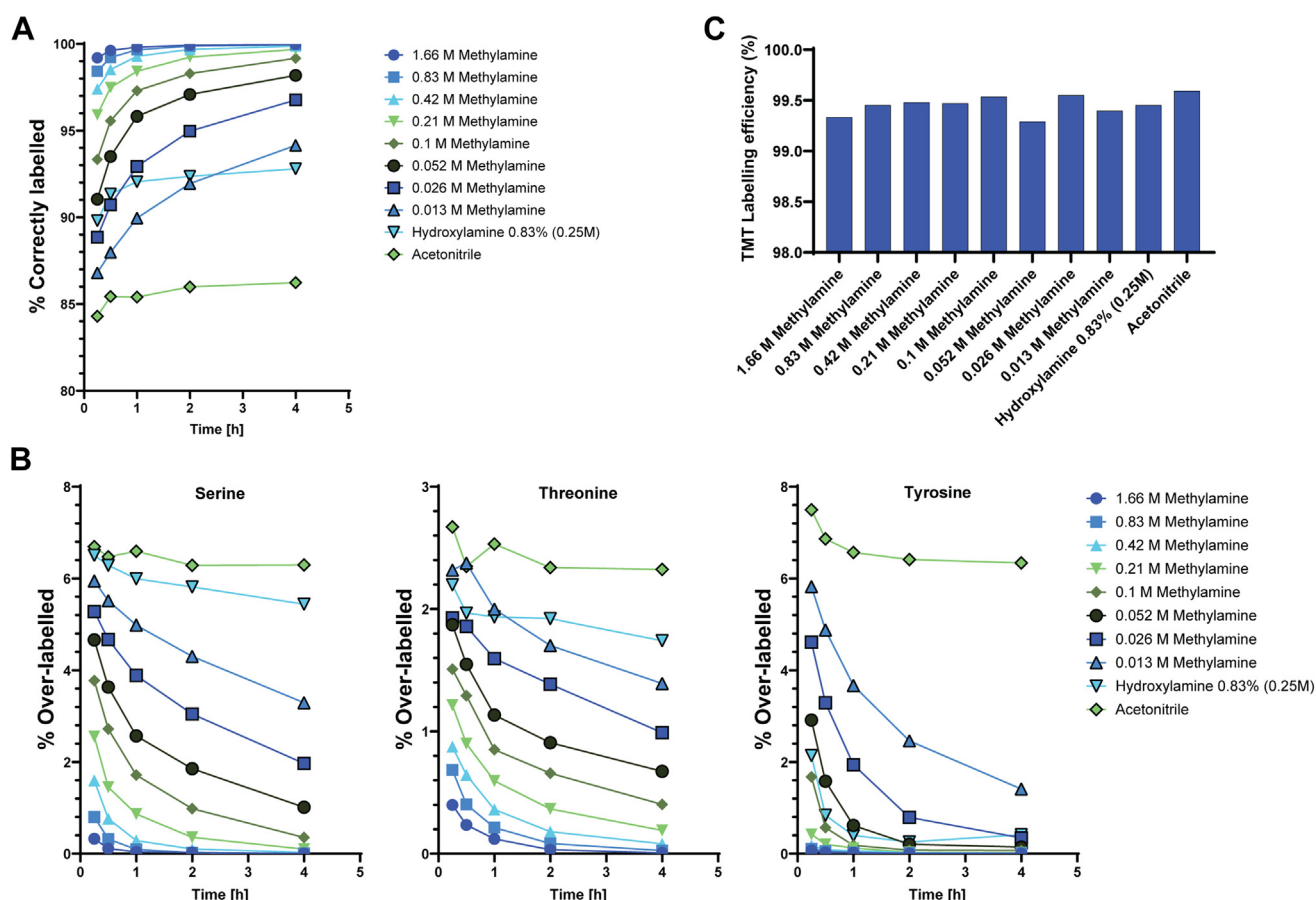
FIG. 4. Optimization of methylamine concentration and reaction time to minimize the proportion of overlabeled peptides. A, a line graph showing the proportion of peptides (by intensity) correctly labeled only at lysines and N termini after 15 min to 4 h of quenching with increasing concentrations of methylamine compared with standard treatment with hydroxylamine and no quenching controls. B, a line graph showing the proportion of peptides (by intensity) containing O -acyl esters of serines, threonines, and tyrosines for each treatment and timepoint. C, a bar chart showing the proportion of labeled lysines and N termini (labeling efficiency) after 2 h of treatment.
