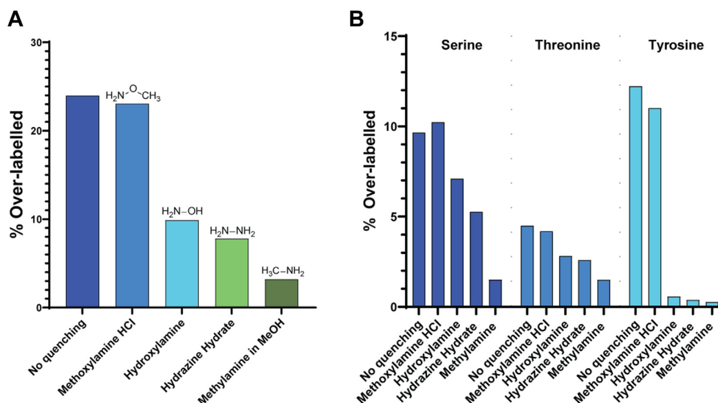
FIG. 3. Screening of aminolysis reagents. A, bar chart showing the percentage of the intensity attributable to peptides containing at least one overlabelled residue after treatment with 50% acetonitrile (control) or 0.3 M of each: methoxylamine, hydroxylamine, hydrazine hydrate, and methylamine. B, a bar chart showing the percentage of overlabelled peptide intensity by ester type after each treatment.
