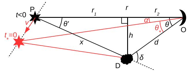
Figure A1. Schematic representation of the geometry causing an echo in the pulse profile (not to scale). A density variation in the IISM (D) deflects radio waves emitted from a pulsar (P) back to the observer (O). The pulsar is moving with a velocity v with respect to the IISM structure and thus the angles \alpha , \theta and \theta' evolve with time. Two different epochs are represented: red symbols indicate the system configuration at the closest approach, i.e. when \theta and \theta' are smallest, whereas black symbols refer to an arbitrary time t ( t < 0 in this example). The distance h of the LoS to the IISM structure divides the distance r from Earth to the pulsar in two segments r_1 and r_2 . x is the distance between the pulsar and the IISM structure D.
