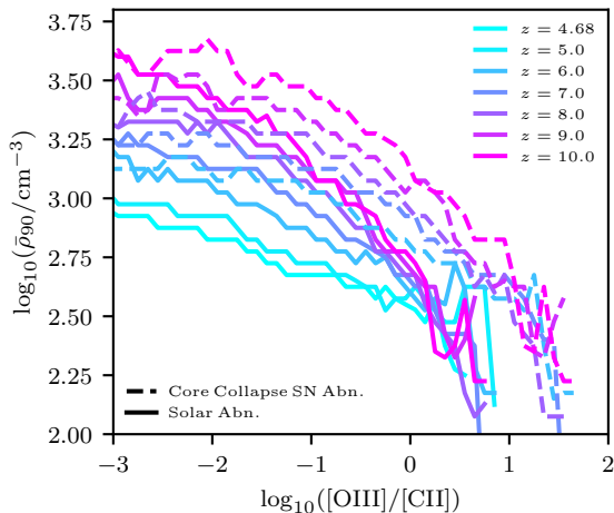
Figure 10. [\text{OIII}]/[\text{CII}] versus \log_{10}(\bar{\rho}_{90}/\text{cm}^{-3}) for galaxies in our simulation versus observations. \rho is defined to be the 90th percentile value from the [\text{CII}] and [\text{OIII}] emitting gas in the galaxies. The coloured lines indicate the median relation for different redshift bins. Solid and dashed lines represent the results when we assume Solar abundances and core collapse SN abundances, respectively. We only include galaxies in this plot that have an \text{SFR} > 10^{-2} M_{\odot} \text{yr}^{-1} .
