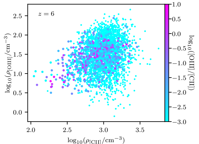
Figure 11. Luminosity-weighted gas density of [\text{CII}] regions versus [\text{OIII}] regions for galaxies at z = 6 coloured by the ratio of [\text{OIII}]/[\text{CII}] . We only include galaxies that have \text{SFR} > 10^{-2} M_{\odot} \text{yr}^{-1} as well as [\text{CII}] and [\text{OIII}] luminosities > 10^3 L_{\odot} . [\text{OIII}]/[\text{CII}] ratios are shown for the Solar abundance model although the results are not fundamentally different for the core collapse SN abundance model.
