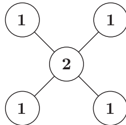
Figure 6.1: The \tilde{D}_4 Dynkin diagram represents a configuration of five spheres with edges indicating a single point of transverse intersection and the number is the algebraic multiplicity of the sphere.
