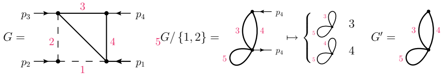
Fig. 7 A graph G with a massive loop (edges 3, 4 and 5), two massless propagators {1, 2} and four external legs ( p_1^2 \neq 0 massive and p_2^2 = p_3^2 = p_4^2 = 0 massless). Since the only momentum p_4 running through the graph after contracting 1 and 2 is null ( p_4^2 = 0 ), the associated integral is the same as for G'
