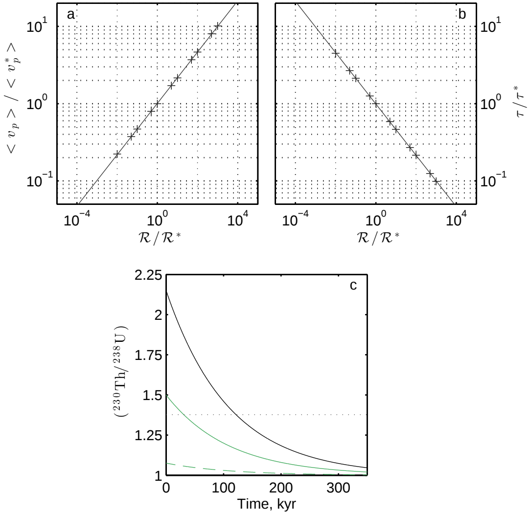
Figure 6.10: The effect of \mathcal{R} = k_0 \Delta \rho g / \mu on melt migration computed using the upwelling column model outlined in chapter 4. The upwelling rate is 6 cm/yr and the grid spacing is 1 km in each direction. Other parameter values are given in table 5.2. (a) Effect of \mathcal{R} on the mean particle speed \langle v_p \rangle . \mathcal{R}^* and \langle v_p \rangle^* indicate normalizing values computed from an experiment that shares the same \mathcal{R} value as other experiments presented in this chapter. (b) Effect of \mathcal{R} on the duration of melt migration \tau , where \tau^* is the duration associated with the \mathcal{R}^* parameter regime. (c) Figure shows how the range of excesses computed by the numerical experiments run with mantle heterogeneity changes with time. Green dashed curve corresponds to the minimum initial excess predicted by the random blob and smoothed noise cases, solid green curve corresponds to the maximum initial excess generated in the spinel zone, black curve corresponds to the maximum initial excess generated in the garnet zone. Black dotted line shows the maximum observed ^{230}\text{Th} excess from the dataset presented in figure 6.1.
