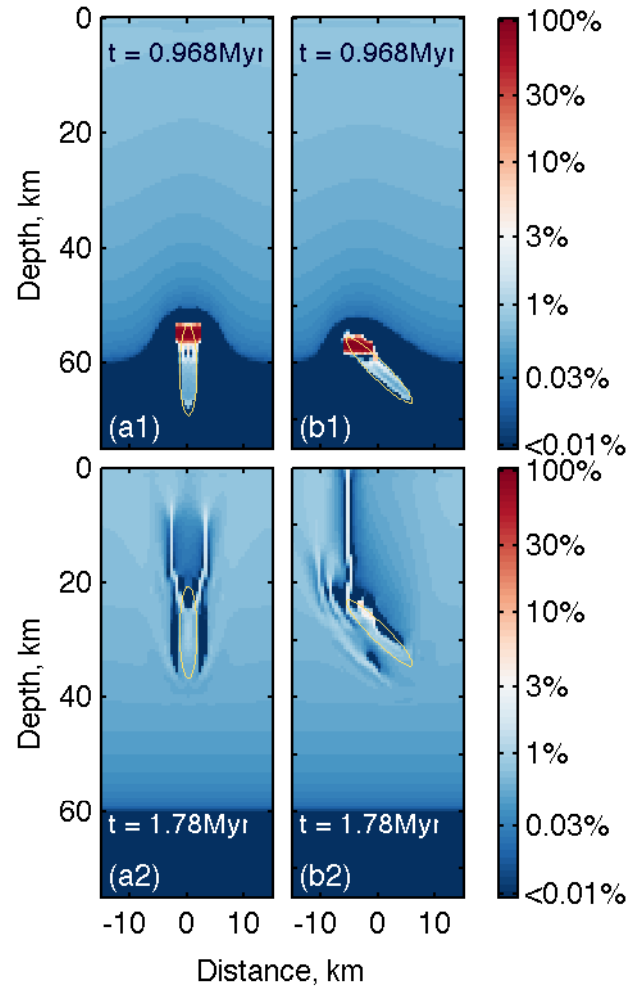
Figure 4.11: Solutions to two different experiments shown in terms of porosity. The original shape of the enclave for both experiments is an ellipse. The ellipse shown in panels b1 and b2 has been rotated by 45^\circ . The long and short axes of the ellipse are 16 km and 4 km respectively. All other parameters take the default values given in table 4.2. Snapshots referenced by the same letter are taken from the same experiment. Yellow ellipses show what would be the perimeter of the unmolten enclaves.
