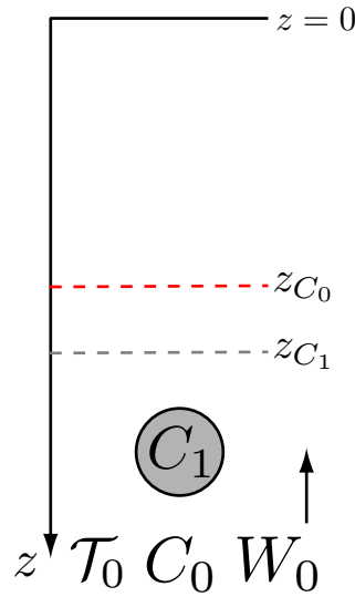
Figure 4.1: Schematic showing the general setup of our experiments. Solid rock flows into the base of the column at a rate W_0 . It has a known potential temperature \mathcal{T}_0 , and known composition C_0 . The initial composition field contains a lithological heterogeneity (grey circle) of composition C_1 < C_0 that is enriched in the more fusible chemical component. The ambient mantle begins to melt at a depth z_{C_0} . Since the lithological heterogeneity is more fusible, it begins to melt at the deeper depth of z_{C_1} .
