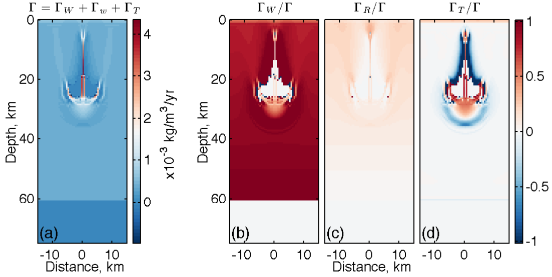
Figure 4.12: Panel a shows the melting rate from an experiment run with the default parameter values (table 4.2) after a model time of 1.81 Myr. The melting rate is the sum of contributions from the upwelling rate of the matrix \Gamma_W , the upwelling rate of the magma \Gamma_R , and thermal diffusion \Gamma_T . Panels b–d show each of these contributions as a fraction of the total melting rate.
