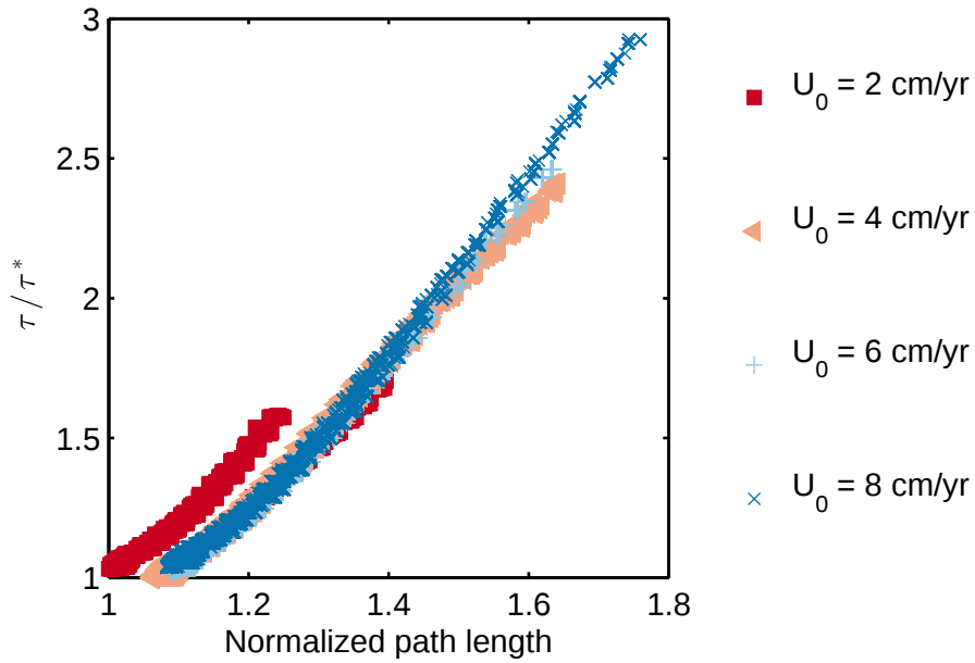
Figure 6.6: Scaled travel time versus nondimensional distance for the experiments conducted with no mantle heterogeneity. Travel time \tau is scaled by \tau^* = (3/2U_0)^{1-1/n}/l , where l is a characteristic length scale.
