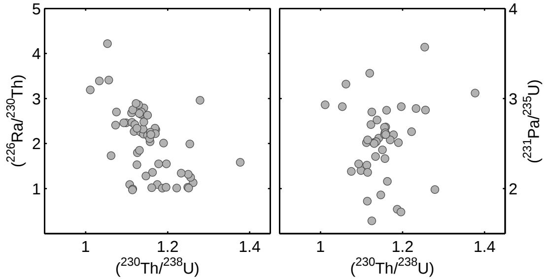
Figure 6.1: (a) Variation of ^{226}\text{Ra}/^{230}\text{Th} with ^{230}\text{Th}/^{238}\text{U} . Measurements from the Juan de Fuca ( U_0 = 3 cm/yr) and Gorda ( U_0 = 2.75 cm/yr) ridges (Goldstein et al., 1991; Volpe and Goldstein, 1993; Lundstrom et al., 1995; Cooper et al., 2003), East Pacific Rise 9–10°N ( U_0 = 5.5 cm/yr) (Volpe and Goldstein, 1993; Lundstrom et al., 1999; Sims et al., 2002), Mid-Atlantic Ridge 33°S ( U_0 = 1.8 cm/yr) (Lundstrom et al., 1998). (b) Variation of ^{231}\text{Pa}/^{235}\text{U} with ^{230}\text{Th}/^{238}\text{U} . Locations and references as above with additional data from (Goldstein et al., 1993). All measurements are made using mass spectrometry. Data compiled by Elliott and Spiegelman (2003).
