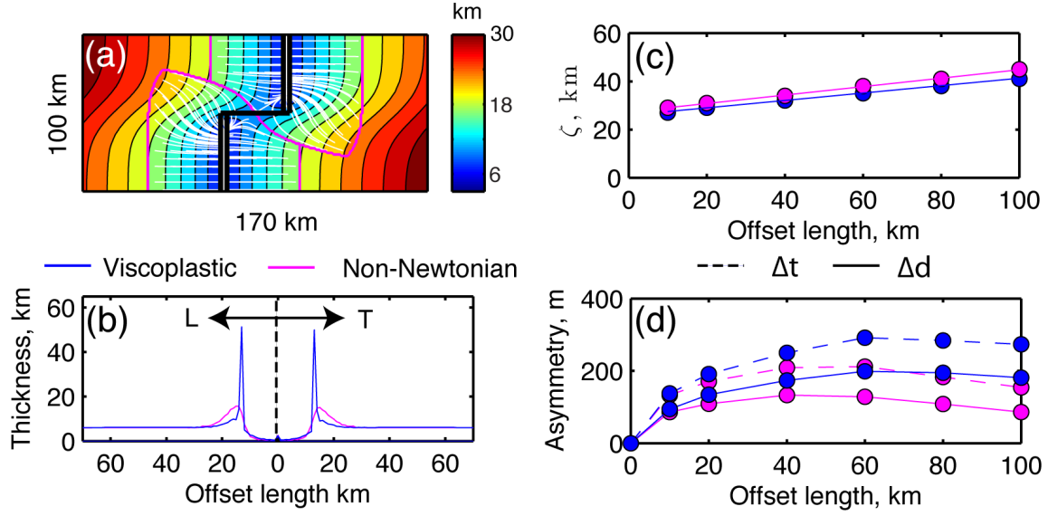
Figure 3.8: Comparison of results from a two suites of simulations, one having a non-Newtonian rheology (magenta lines) and the other using a viscoplastic rheology (blue lines). All simulations have U_r = 2\text{cm/yr} and a domain depth of 300 km. (a) Map showing the relationship between solidus depth, focusing region shape and melt focusing trajectories. White streamlines show melt focusing trajectories. Black lines outline the geometry of the ridge system. Magenta lines mark the perimeters of the focusing regions. Coloured contours show depth to the top of the melting region. The transform fault length is 40 km. Ridge is migrating to the left. This figure can be compared directly with its non-Newtonian analogue in figure 3.3a. (b) Profiles showing the along-axis crustal thickness prior to redistribution of the melt. The offset length for these simulations is 40 km. L and T denote the leading and trailing ridge segments respectively. (c) Variation in the redistribution length \zeta as a function of transform fault length. (d) Comparison of the difference in crustal thickness ( \Delta t , dashed) and axial depth ( \Delta d , solid) for the two suites of simulations as a function of offset length.
