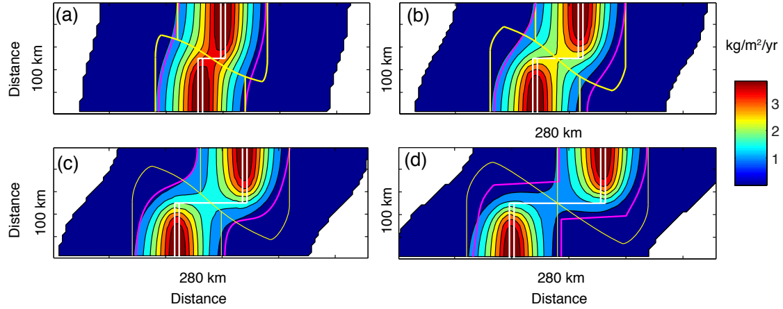
Figure 3.7: Maps contoured for the melting rate integrated over the depth of the domain. White lines show the trace of the ridge system, yellow lines show the outlines of the focusing regions, and magenta lines show the trace of the extremal surfaces on the base of the melting region. Results taken from simulations with U_r = 1\text{cm/yr} and offsets of (a) 20 km, (b) 40 km, (c) 60 km, (d) 80 km.
