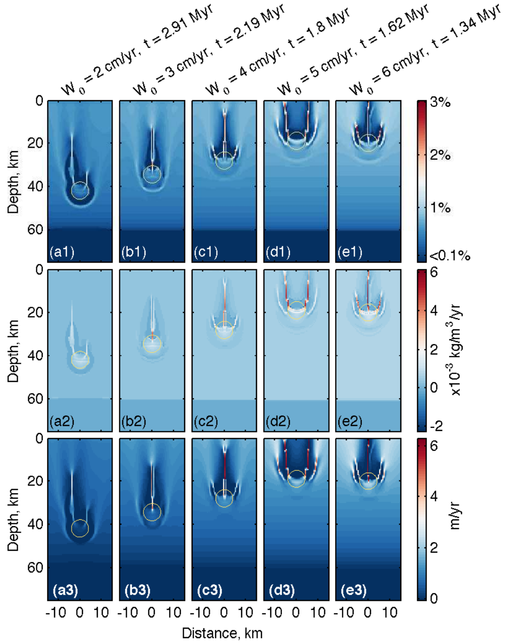
Figure 4.10: Solutions to a suite of five different experiments for which the upwelling rate is varied. All other parameters take the values given in table 4.2. Figures show snapshots from the experiment at 0.5 Myr after the onset of channelization. Snapshots referenced by the same letter are taken from the same experiment. Panels a1–e1 show the solutions in terms of porosity, and panels a2–e2 show them in terms of the melting rate, and panels a3–e3 show the solutions in terms of the magma speed. Yellow circles show what would be the perimeter of the unmolten enclave.
