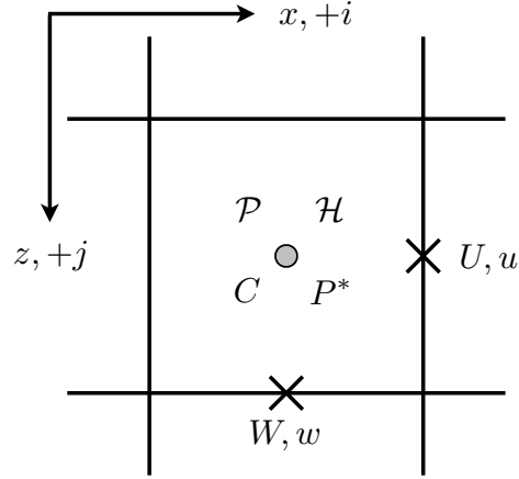
Figure 4.3: Schematic showing where the variables are located in each grid cell. \mathcal{H} , \mathcal{P} , \mathcal{U} , C , in addition to C_m and C_f (not shown) are located at the centre. The horizontal and vertical components of velocity for the matrix ( U = \mathbf{v}_m \cdot \mathbf{x} , W = \mathbf{v}_m \cdot \mathbf{k} ) and magma ( u = \mathbf{v}_f \cdot \mathbf{x} , w = \mathbf{v}_f \cdot \mathbf{k} ) are placed on the +i and +j faces respectively.
