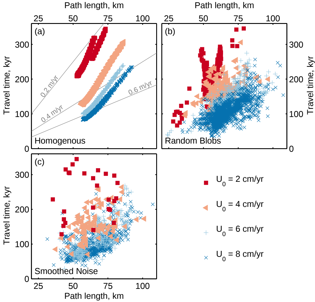
Figure 6.2: Travel time for individual particles plotted as a function of path length for half-spreading rates of 2, 4, 6, and 8 cm/yr. Figure (a) shows data from experiments run in a homogenous mantle. Grey lines correspond to the magma flow speeds indicated. (b) shows data from simulations where the heterogeneity is manifested as random blobs, and (c) plots data from simulations run with smoothed noise heterogeneity.
