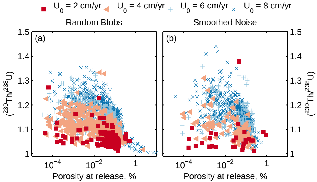
Figure 6.9: Variation of the decayed excesses for the erupted tracers with the porosity at the points from which the tracers are released. (a) Results from experiments run with the random blob heterogeneity. (b) Results from experiments run with the smoothed noise heterogeneity.
