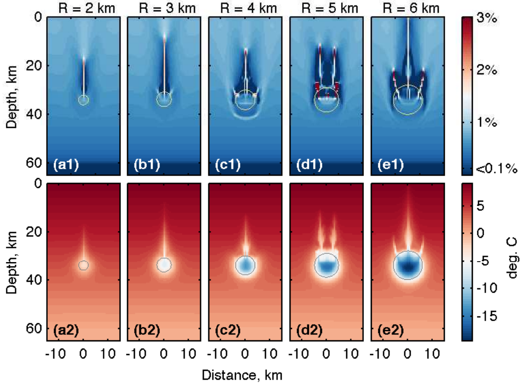
Figure 4.8: Solutions from a suite of five different experiments at t = 1.65 Myr for which the radius R is varied. All other parameters use the default values given in table 4.2. Snapshots referenced by the same letter are taken from the same experiment. Panels a1–e1 show the solutions in terms of porosity, whilst panels a2–e2 show \Delta T_C . Circles show the perimeter of what would be the unmolten enclave.
