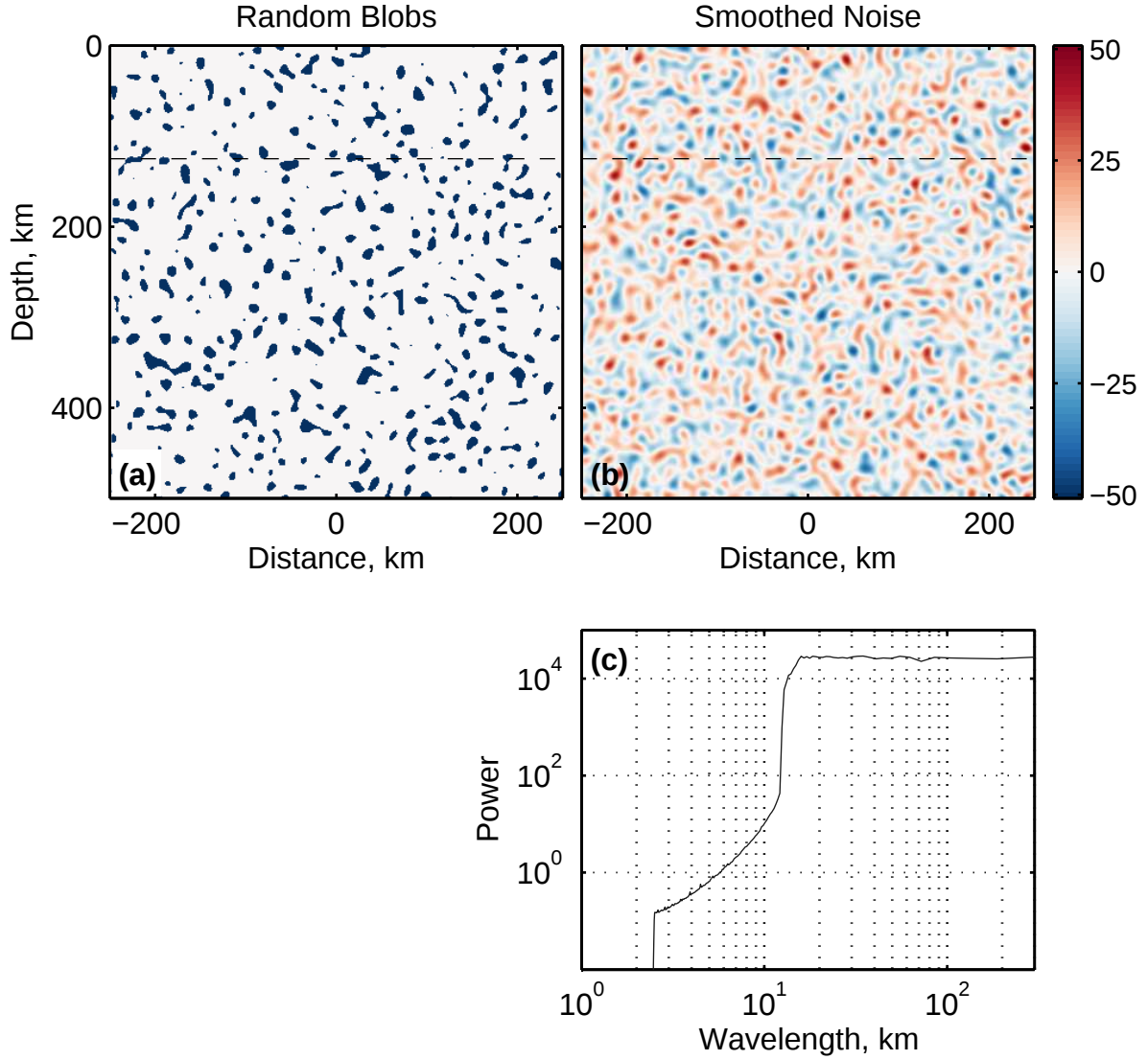
Figure 5.2: Results from the algorithms used to generate mantle heterogeneity, shown as a perturbation to the solidus temperature given by \Delta T_C = M_S(C_m - C_0) . The background composition C_0 is set to 0.5. Dashed lines in panels a and b indicate the size of the computational domain relative to the fields of heterogeneity; the heterogeneity fields are larger in the z -direction in order to satisfy the bottom boundary on C as material is advected into the domain. (a) Result from the random blob algorithm. 10% of the area is occupied by fertile heterogeneities. (b) Result from the smoothed noise algorithm. (c) Directionally averaged power spectrum for the heterogeneity field in panel b. It shows approximately uniform power above a wavelengths > 11 km and greatly reduced power for shorter wavelengths.
