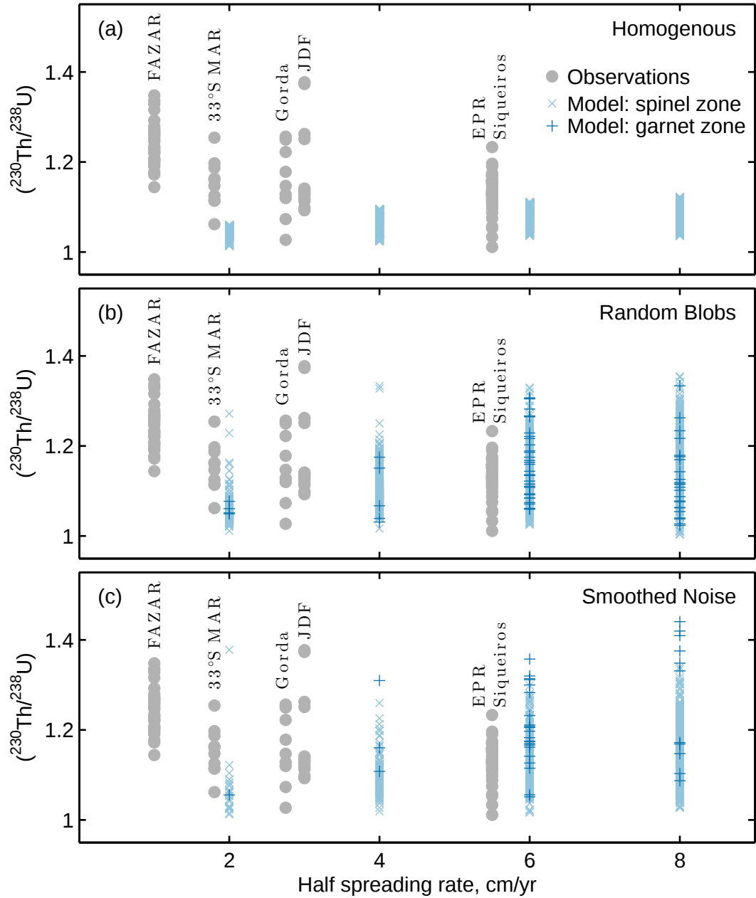
Figure 6.8: Variation in predicted and observed ^{230}\text{Th} excesses with spreading rate. (a) Results from experiments run with no mantle heterogeneity. (b) Results from experiments run with the random blob heterogeneity. (c) Results from experiments conducted with the smoothed noise heterogeneity. Grey circles show observations, light blue crosses show modelled excesses for tracers that originate in the spinel zone, dark blue plus signs show modelled excesses for tracers that originate in the garnet zone. Observed excesses are taken from the dataset plotted and referenced in figure 6.1. Abbreviations are as follows: FAZAR, Azores Platform; MAR, Mid-Atlantic Ridge; JDF, Juan de Fuca Ridge; EPR, East Pacific Rise 9 – 11°N.
