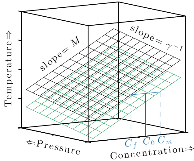
Figure 4.2: Linearized surfaces for the solidus (lower surface) and liquidus (upper surface). C_0 marks the bulk magma composition at zero pressure. C_f and C_m show the compositions of coexisting magma and solid rock. The mass fraction of the liquid is given by (C_0 - C_f)/(C_m - C_f) .
