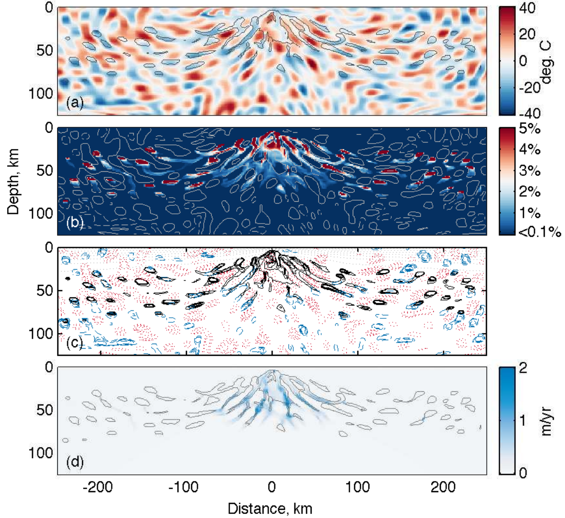
Figure 6.7: Covariation of porosity and composition from a representative experiment initialized with the smoothed noise heterogeneity model and U_0 = 6 cm/yr. (a) Colours show composition in terms of a perturbation to the solidus temperature, black lines contour \phi = 1\% . (b) Colour shows porosity, grey dashed lines contour \Delta T_C = -15^\circ\text{C} , grey solid lines contour \Delta T_C = +10^\circ\text{C} . (c) Covariation of large porosities and regions of enriched and depleted mantle. Black lines contour \phi = 1\% , blue solid lines contour \Delta T_C \leq -15^\circ\text{C} in 5^\circ\text{C} intervals, and red dashed lines contour \Delta T_C \geq +10^\circ\text{C} in 5^\circ\text{C} intervals. (d) Magma speed |\mathbf{v}_f| with grey lines showing the 1% porosity contour.
