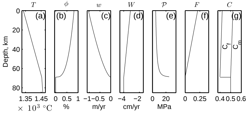
Figure 2.2: Steady one dimensional solutions to the equations provided in Appendix A for (a) temperature, (b) porosity, (c) magma speed (d) upwelling rate of the mantle (e) compaction pressure, (f) degree of melting (g) liquid ( C_f ) and solid ( C_m ) compositions, subject to the parameter values given in table 2.1.
