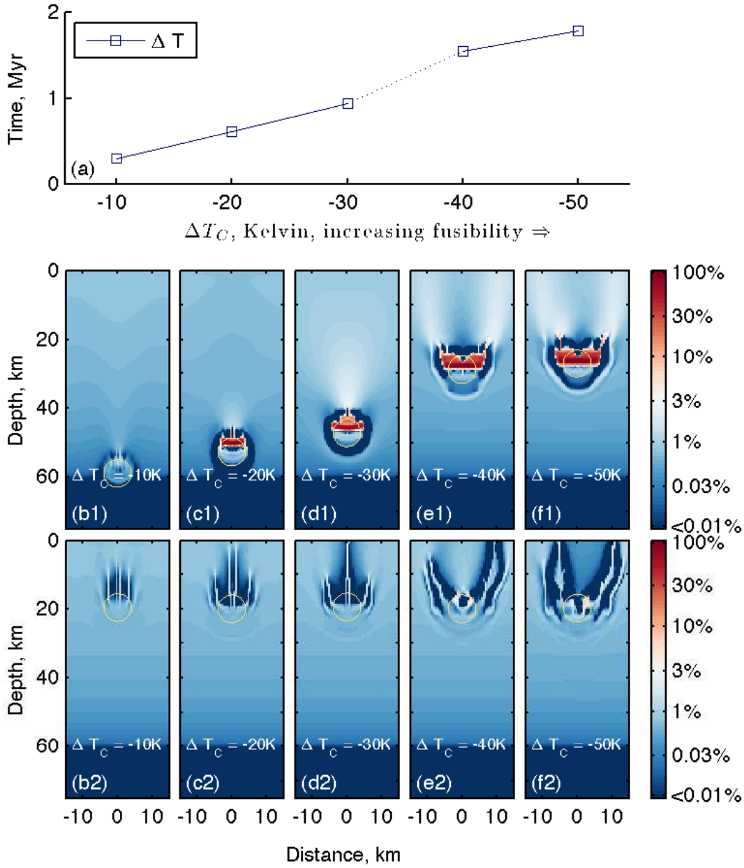
Figure 4.9: Solutions to a suite of five different experiments for which the enrichment of the heterogeneity \Delta T_C is varied. All other parameters use the default values given in table 4.2. Panel a shows how the time \Delta t between the onset of channelization and the onset of melting within the enclave varies with \Delta T_C . The dotted line indicates where the relationship between \Delta t and \Delta T_C is uncertain. Panels b1–f1 show solutions from each experiment, in terms of porosity at the instant preceding channelization. Panels b2–f2 show the solutions in terms of porosity at t = 2.01 Myr. Snapshots referenced by the same letter are taken from the same experiment. Yellow circles show what would be the perimeter of the unmolten enclave.
