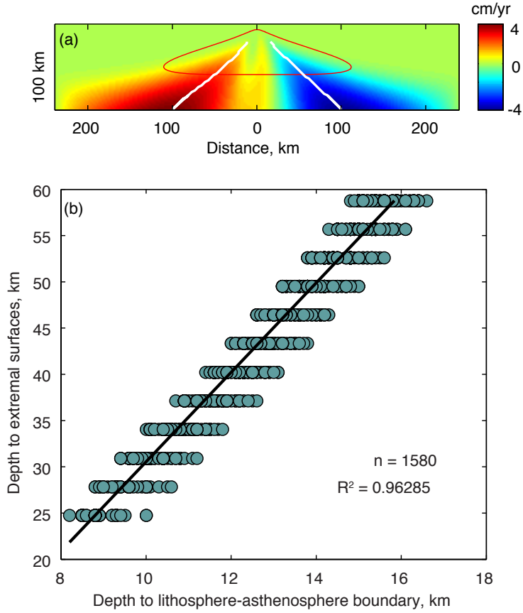
Figure 3.6: Results from analogous 2D and 3D calculations with U_r = 1\text{cm/yr} and an asthenospheric depth of 100 km. (a) Figure shows, for a 2D simulation, the locations of extremal values of W' and the shape of the melting region. Coloured field is the component of upwelling induced by ridge migration, W' . White bold lines mark the extremal values of W' as a function of depth. The red contour outlines the melting region. (b) This figure shows, for the analogous 3D simulation, the relationship between the depth to the extremal surfaces of W' and the depth to the lithosphere–asthenosphere boundary (LAB). The black line is least squares best fit line taken through all data points.
