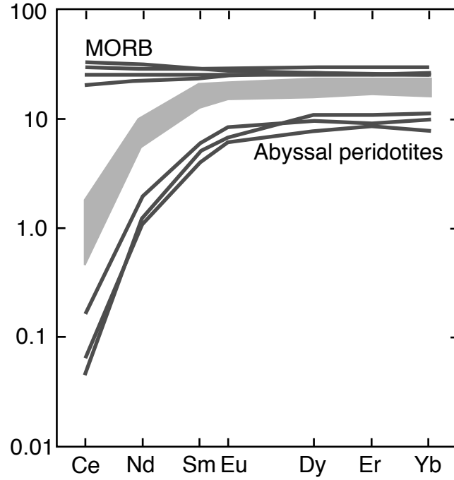
Figure 1.4: Chondrite normalized rare earth element patterns from clinopyroxene crystals hosted in abyssal peridotites and spatially associated basalts from the Atlantis II Fracture Zone, Southwest Indian Ridge. Grey region shows compositions of hypothetical melts in equilibrium with the abyssal peridotites. Modified from Johnson et al. (1990) by permission of American Geophysical Union.
