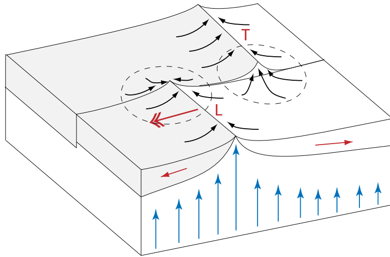
Figure 3.1: Schematic showing a ridge system consisting of a leading and trailing ridge segment separated by a discontinuity. (The leading and trailing ridge segments are marked L and T respectively.) Single headed red arrows show spreading component of plate motion whilst the double headed red arrow indicates the direction of ridge migration. The leading plate is shaded grey. Blue vertical arrows depict upwelling in the underlying mantle and black arrows show hypothetical melt focusing trajectories. The dashed circles represent idealized regions of melt focusing, which extend into the mantle beneath the adjacent plates. Melt tapped from these regions contributes to the morphological asymmetry of ridge segments separated by an offset.
