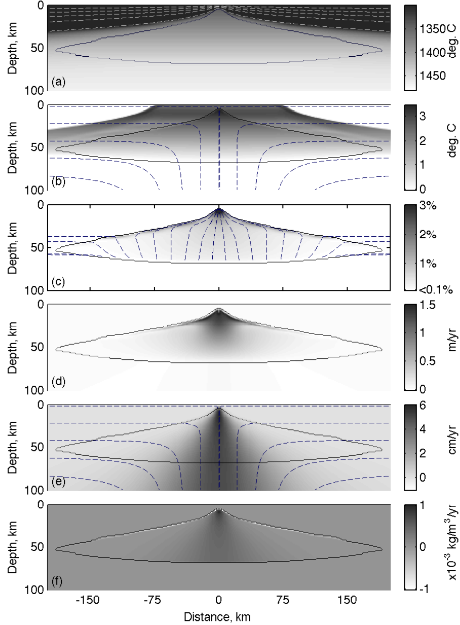
Figure 5.3: A snapshot from a simulation with no initial mantle heterogeneity and U_0 = 4 cm/yr after a model time of 2 Ma. Black solid lines in all panels contour the solidus. (a) Temperature with dashed grey lines contouring temperature in the lithosphere in intervals of approximately 200 K. (b) Composition of the solid mantle, expressed as a perturbation to the solidus temperature. Dashed blue lines show flow lines for the convecting mantle. (c) Porosity, with dashed blue lines representing flow lines for the magma. (d) Magma speed |\mathbf{v}_f| , (e) upwelling rate of the solid mantle |\mathbf{v}_f \cdot \hat{\mathbf{k}}| , (f) melting rate. Parameter values for this experiment are given in table 5.2.
