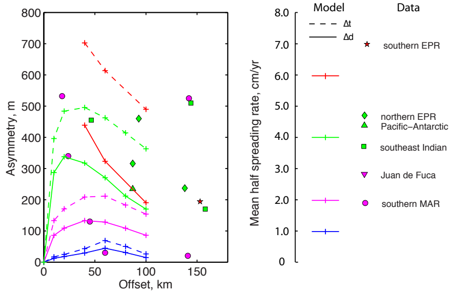
Figure 3.5: Left panel: Model results and global data showing the difference in axial depth of two ridge segments separated by an offset, as a function of offset length. Right panel shows legend. All simulations have a grid resolution of 3 km in each direction, an asthenospheric depth of 300 km. Data for transform faults on intermediate and fast spreading ridges (Juan de Fuca, JDF, south east Indian Rise, SEIR, Pacific Antarctic Rise, PACANT, north east Pacific Rise, NEPR, south east Pacific Rise, SEPR) are from Carbotte et al. (2004) , and for the southern Mid-Atlantic Ridge (SMAR) from Katz et al. (2004) . The data set covers some 11,000 km of MOR along which 76% of the leading ridge segments have a shallower bathymetry than the trailing ridge segment for all offsets in excess of 5 km. Any data not fitting this trend is excluded from the figure. Simulations for U_r = 6\text{cm/yr} with offsets of 10 km, 20 km, and 80 km did not converge to a solution.
