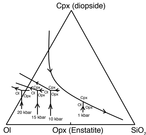
Figure 1.3: Projection of the basalt tetrahedron from plagioclase onto the plane olivine–diopside–silica. Black lines show experimentally determined cotectics for olivine (ol), clinopyroxene (cpx) and orthopyroxene (opx) taken from Stolper (1980) .
