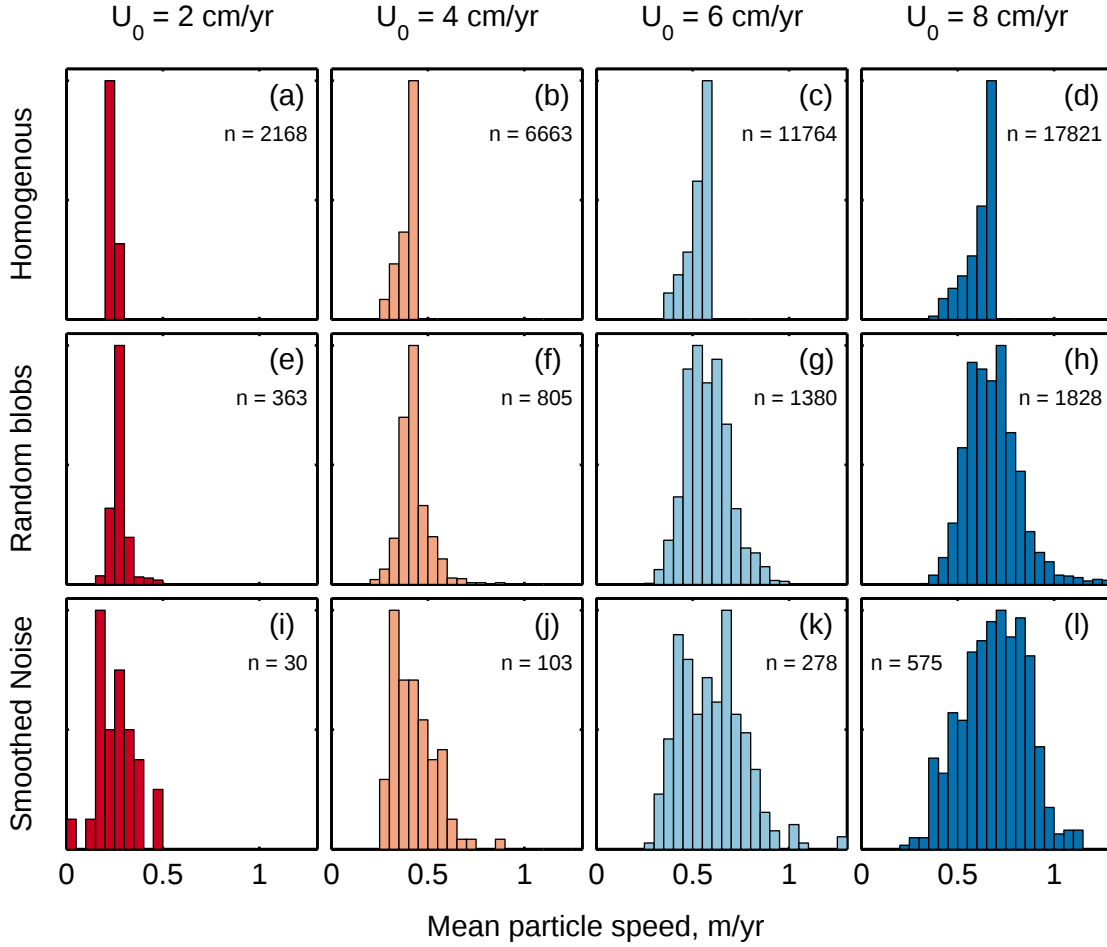
Figure 6.3: Normalized histograms showing the local mean speeds of particles. Each column shows results from simulations with the same half-spreading rate and each row presents data from simulations with different styles of heterogeneity as the initial condition. Bin widths are 5 cm/yr.
