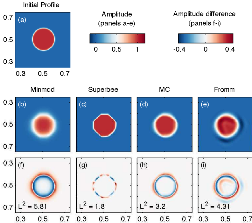
Figure B.1: Results from tests in which an initial profile is advected diagonally across the grid in a top left-to-bottom right direction using different advection schemes. (a) Initial profile. (b–e) Final solution after the initial profile has made one pass around the grid. (f–i) Plots of the difference between each final solution and the initial profile. The L^2 norm of the result is indicated on each panel.
