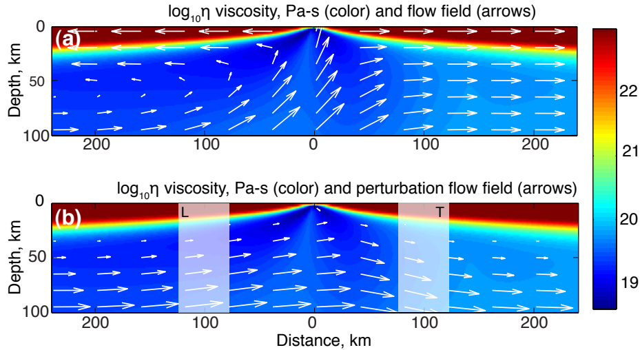
Figure 3.2: Example output from the 2D simulations by Katz et al. (2004). These figures compare the mantle flow pattern beneath a migrating ridge (a) and the component of mantle flow induced by ridge migration (b). (a) Solid mantle flow pattern (white arrows) from 2D simulation with half spreading rate U_o = 4\text{cm/yr} and ridge migration rate U_r = 4\text{cm/yr} . The ridge is migrating to the left. Coloured background shows viscosity in Pa s. (b) Component of mantle flow caused by ridge migration. White boxes show the regions within the leading (L) and trailing (T) minor focusing regions.
