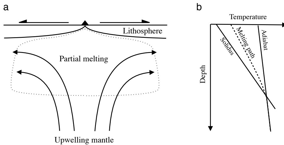
Figure 1.2: (a) The dynamical situation at mid-ocean ridges. Grey dotted line represents region of partial melting. (b) A schematic representation of the solidus, adiabatic temperature profile and temperature profile in the partially molten region directly beneath the ridge axis.
