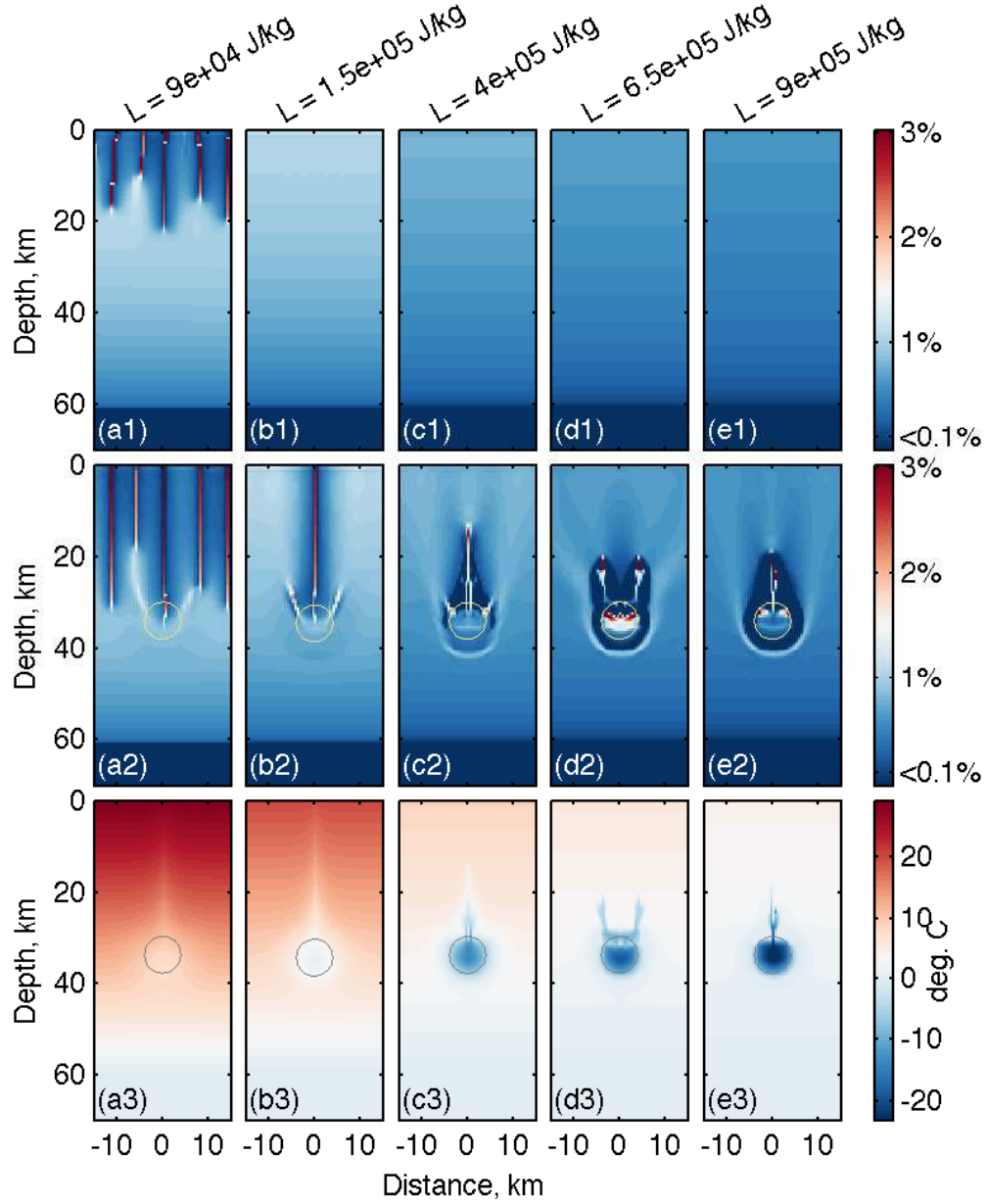
Figure 4.6: Solutions to a suite of experiments for which the latent heat of fusion L is varied. All other parameters are assigned the values listed in table 4.2. Panels a1–e1 show solutions, in terms of porosity for experiments that are not initialized with an enriched heterogeneity. Panels a2–e2 and a3–e3 show solutions from the similar experiments that were initialized with an enriched heterogeneity. Snapshots a2–e2 and a3–e3 show the solutions after a model time of 1.65 Myr in terms of porosity and \Delta T_C respectively. Circles show what would be the perimeter of the unmolten heterogeneity.
