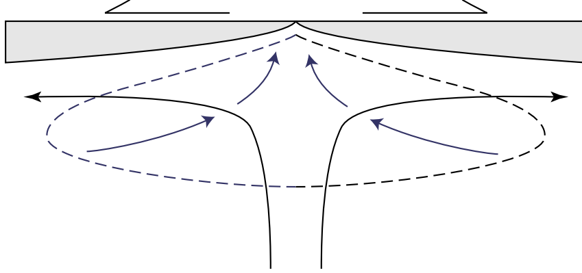
Figure 5.1: Schematic illustrating the model setup. Lithospheric plate (grey regions) diverge at a known rate, driving large scale convection in the solid mantle (black arrows). Decompression causes the mantle to melt within an unknown region indicated by the dashed line. Within this region solid rock and magma coexist and the melt is able to move by porous flow (blue arrows).
