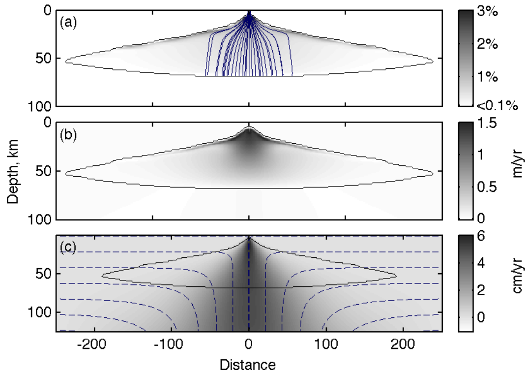
Figure 6.5: Snapshots from an experiment conducted with no mantle heterogeneity and U_0 = 4 cm/yr after a model time of 2 Ma. Black solid lines in all panels contour the solidus. (a) Color shows porosity, blue lines show trajectories of randomly selected tracers that migrate from the base of the melting region to the ridge axis. (b) Magma speed |\mathbf{v}_f| . (c) Upwelling rate of the matrix -\mathbf{v}_m \cdot \hat{\mathbf{k}} . Dashed lines show the flow pattern of the matrix.
