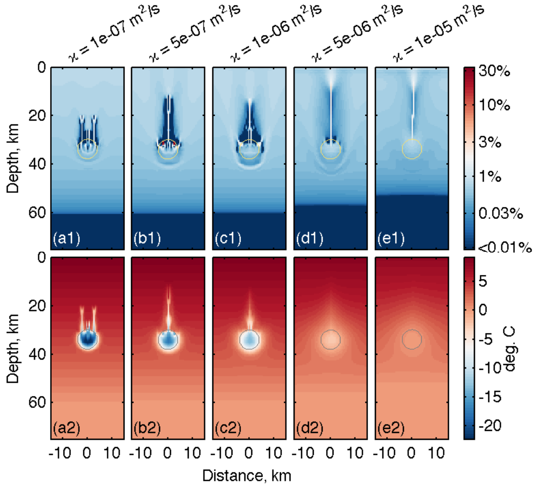
Figure 4.7: Solutions to a suite of five different experiment for which the thermal diffusivity is varied. All other parameters are assigned the default values given in table 4.2. The figures show results from the experiments in terms of porosity (panels a1–e1) and \Delta T_C (panels a2–e2) after a model time of 0.91 Myr. Panels referenced by the same letter are taken from the same experiment. Circles show what would be the perimeter of the unmolten enclave.
