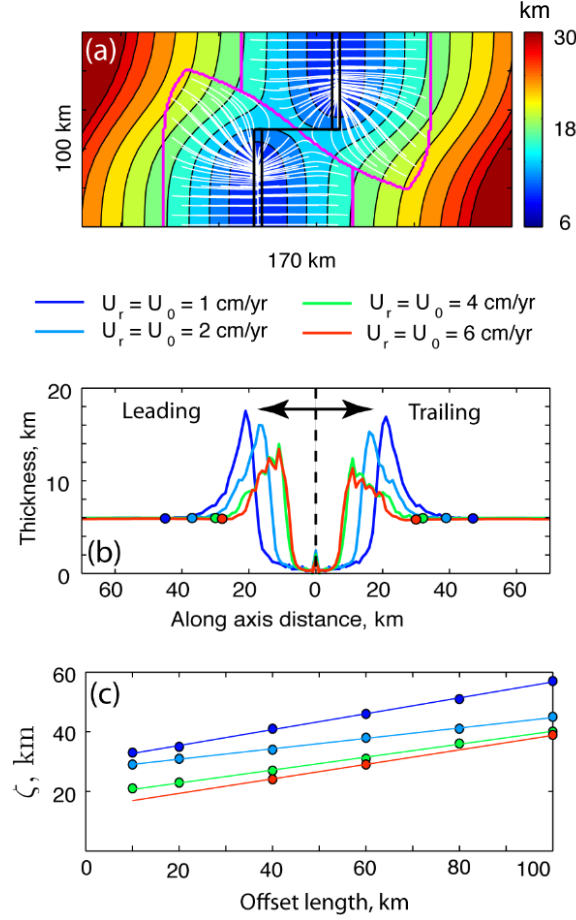
Figure 3.3: Summary of steps needed to focus melt to the ridge and redistribute it along the ridge axis. (a) Map showing the relationship between solidus depth, focusing region shape and melt focusing trajectories. White streamlines show melt focusing trajectories. Black lines outline the geometry of the ridge system. Magenta lines mark the perimeters of the focusing regions. Coloured contours show depth to the top of the melting region. Simulation has U_r = 2\text{cm/yr} and an offset of 40 km. The ridge is migrating to the left. (b) Profiles showing along-axis variation in crustal thickness for simulations with U_r = 1, 2, 4, 6\text{cm/yr} and an offset of 40 km. Solid dots show the positions at which the gradient of the crustal thickness profiles first departs significantly from zero. The distance between these points and the offset for each simulation is the redistribution distance \zeta . (c) Variation in \zeta as a function of transform fault length.
