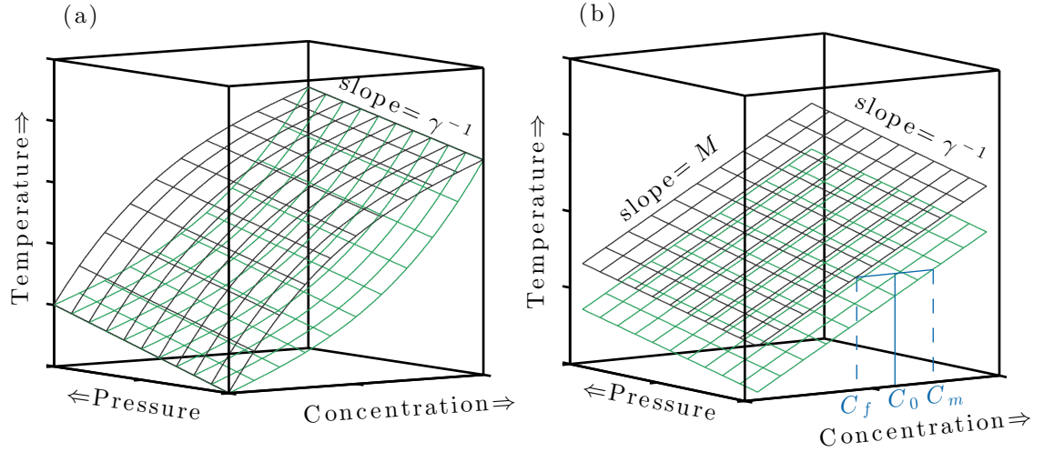
Figure 2.1: (a) Example binary phase loop relating the solidus (lower surface) and liquidus (upper surface) compositions to temperature and pressure. (b) Linearized version of a binary phase loop. C_f and C_m indicate the liquid and solid compositions in equilibrium with bulk composition C_0 .
