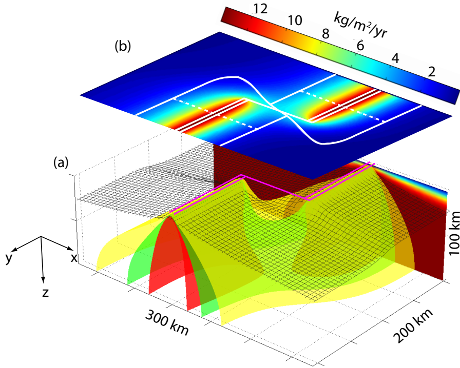
Figure 3.4: Example output from a 3D simulation with U_r = 4\text{cm/yr} and an offset of 80 km. The ridge is migrating to the left. (a) 3D image of the upwelling geometry beneath the ridge system. Magenta lines indicate the position of the transform fault and ridge segments. Red, green and yellow surfaces show constant upwelling rates of 1, 2 and 2.75 cm/yr respectively. Upwelling is asymmetric about the ridge axis. Wire mesh marks the base of the lithosphere, defined by the locus of the maximum rate of change in viscosity in the z -direction. The back wall shows a 2D slice through the potential temperature field. Dark red represents the mantle potential temperature ( 1300^\circ\text{C} ) and dark blue indicates 0^\circ\text{C} . (b) Map of the vertically integrated melting rate, \int_0^Z \Gamma dz . White lines show the location of the ridge segments, transform fault, and the focusing regions. The focusing regions are divided by a white, dashed line into major and minor sub-regions that are distal and proximal to the transform fault respectively. The vertically integrated melting rate is the melt production rate beneath any point on the surface of the solidus that can be focused to a ridge segment.
