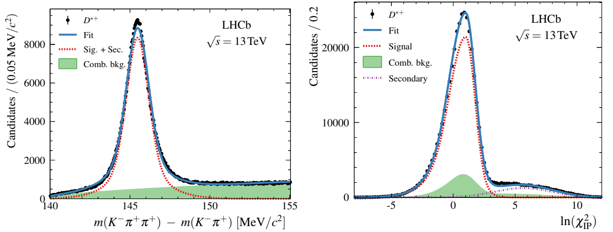
Figure 4: Distributions for selected D^{*+} \rightarrow D^0 \pi^+ candidates, with D^0 \rightarrow K^- \pi^+ : (left) \Delta m = m(D^{*+}) - m(D^0) for a mass window of \pm 20 \text{ MeV}/c^2 around the nominal D^0 mass and (right) \ln \chi_{\text{IP}}^2 with an additional mass window of \pm 3 \text{ MeV}/c^2 around the nominal D^{*+} - D^0 mass difference. The sum of the simultaneous likelihood fits in each (p_T, y) bin is shown, with components as indicated in the legends.
