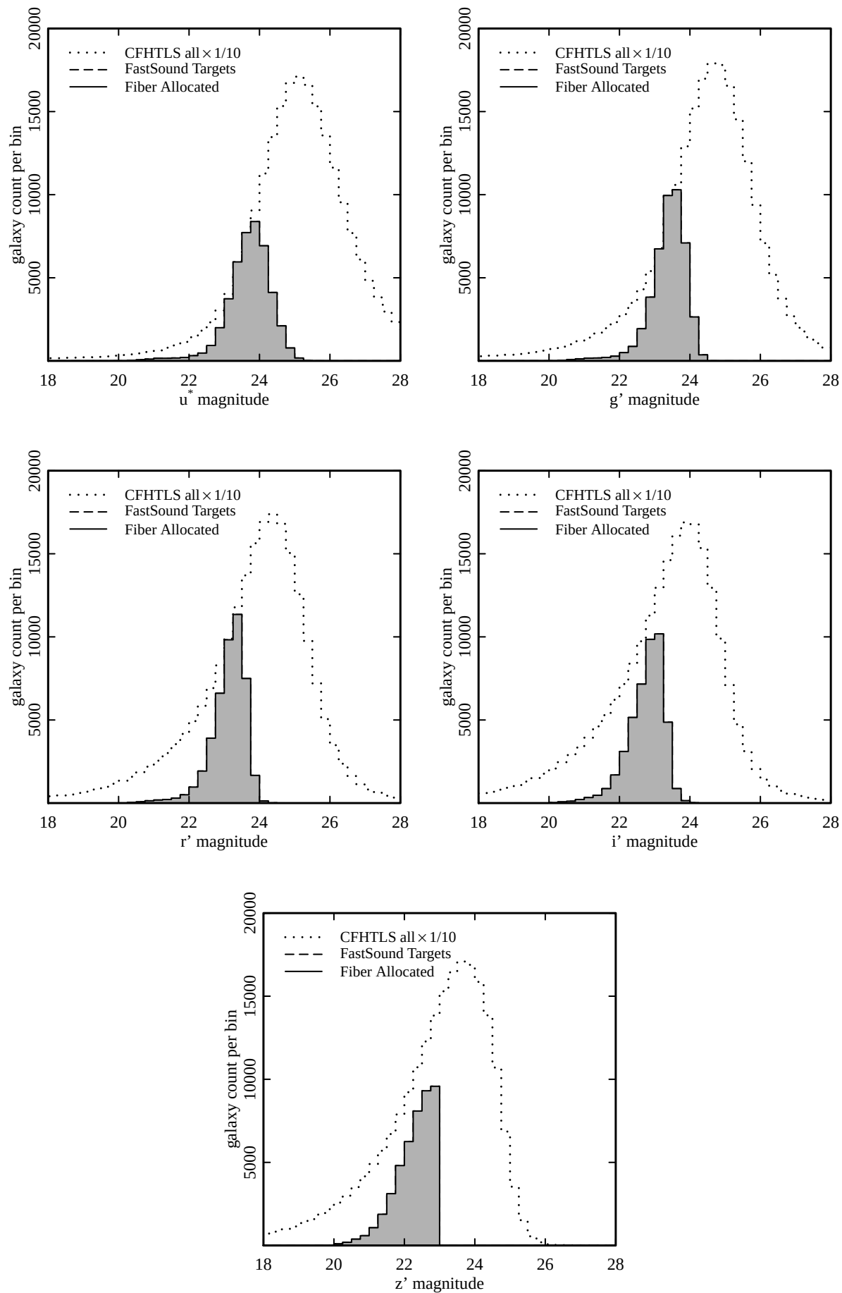
Fig. 3. The histogram of u^*g'r'i'z magnitudes of all CFHTLS Wide galaxies in the FastSound footprints (dotted), FastSound target galaxies (dashed), and galaxies that the fibers were actually allocated to (solid). The cutoff of z' -magnitude at 23.0 is due to our selection condition.
