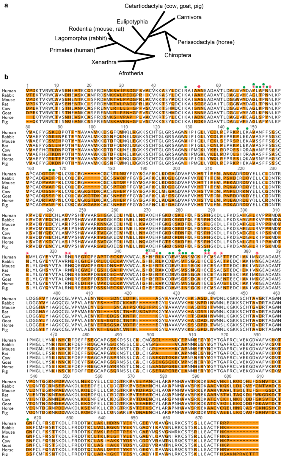
Extended Data Figure 4: Sequence alignment of mammalian transferrin variants analysed in this study
