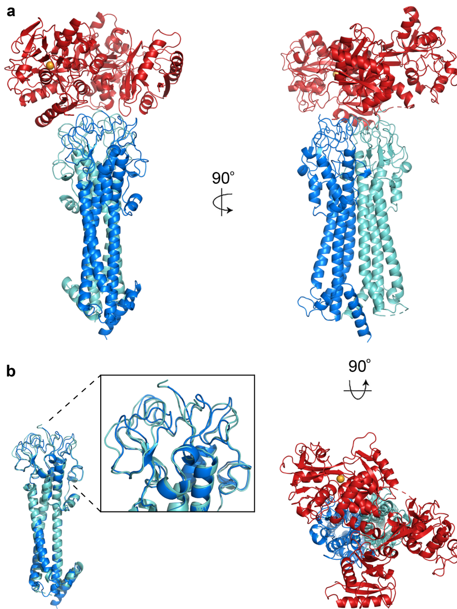
Figure 1: The structure of the trypanosome transferrin receptor
