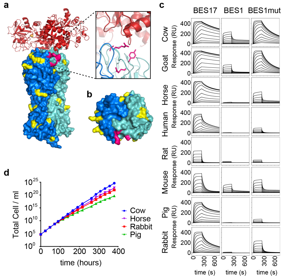
Figure 3: Binding of the transferrin receptor to transferrin from different mammalian species
