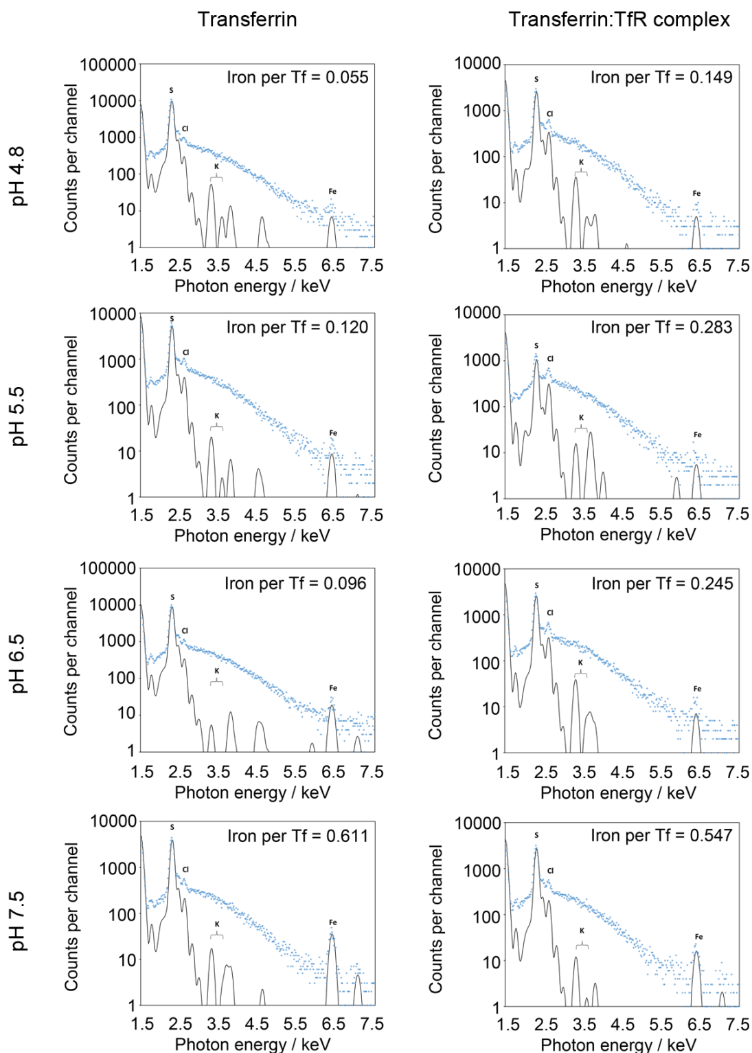
Extended Data Figure 7: elemental analysis by IPIX to determine the number of Fe ions per transferrin or transferrin:TfR complex at different pH values.
