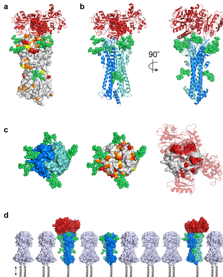
Figure 4: Glycans and sequence diversity concentrate around the membrane distal head of the transferrin receptor.
