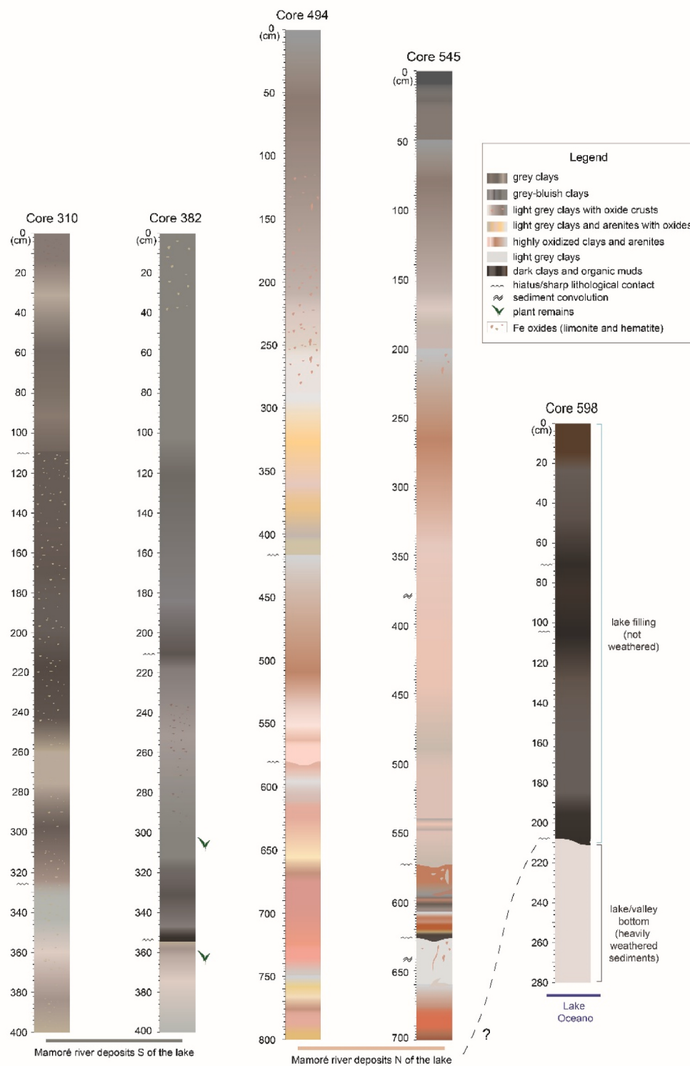
Fig. 2. Lithological columns for cores 310, 382, 494, 545, and 598, and core correlation. The lithologies indicate different sources for the sediments in and around the lake.
