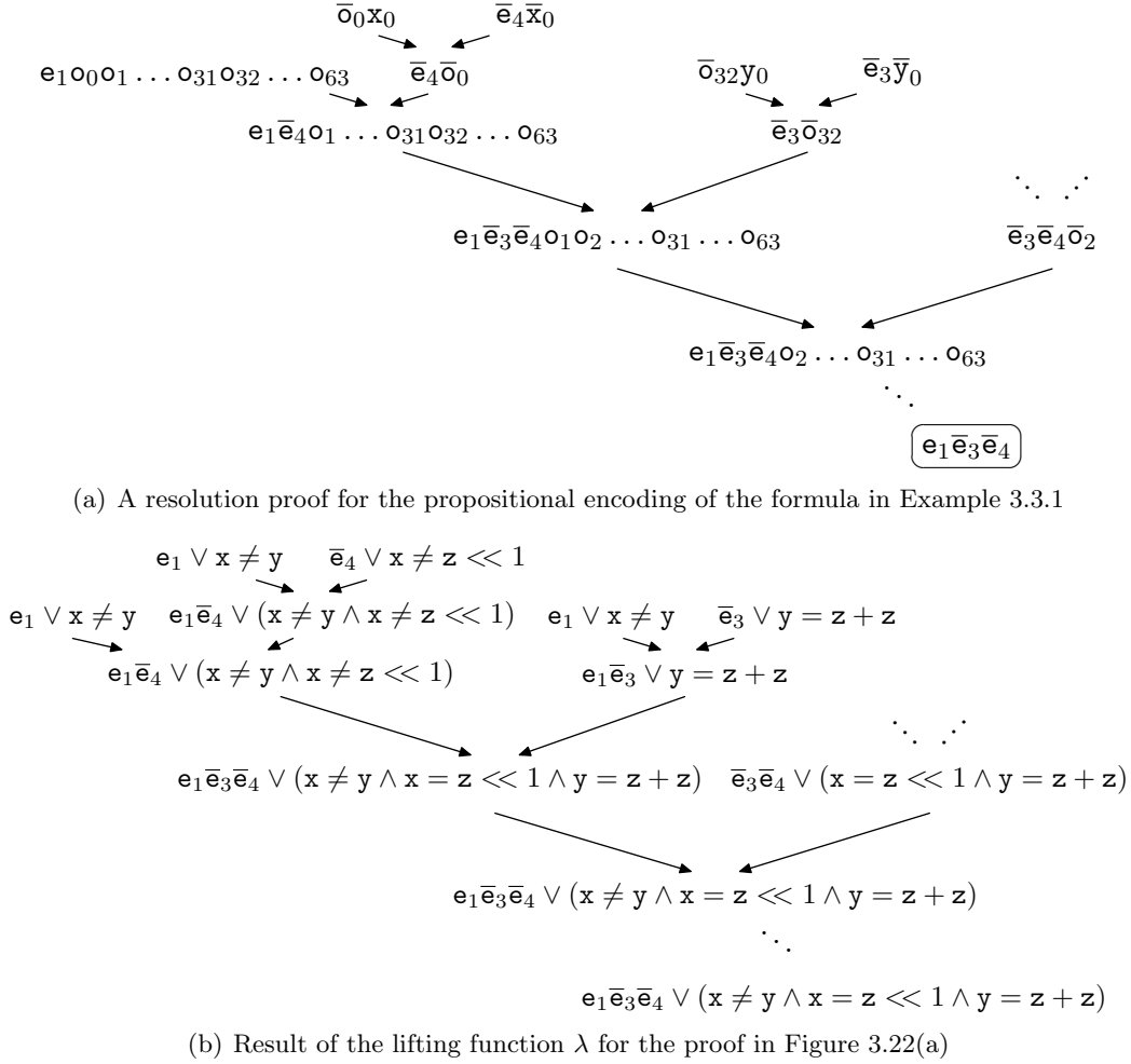
Figure 3.22: Deriving blocking clauses from propositional resolution proofs
