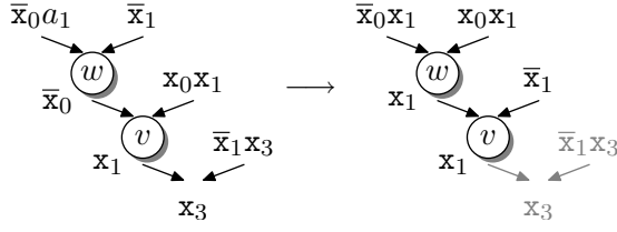
Figure 3.16: The graph R[w \rightleftharpoons v] is not a proof because x_1 is merged.
