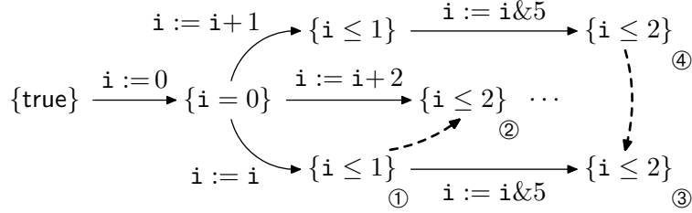
(b) An attempt to construct a safety proof using a non-monotonic predicate transformer
