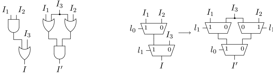
Figure B.3: Circuits representing the annotations I and I' in Figure B.2(a) and Figure B.2(b) for the cases \langle c, d \rangle = \langle b, a \rangle and \langle c, d \rangle = \langle ab, ab \rangle .
