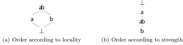
Figure 3.10: Different orders for \{\perp, \mathbf{a}, \mathbf{b}, \mathbf{ab}\}
