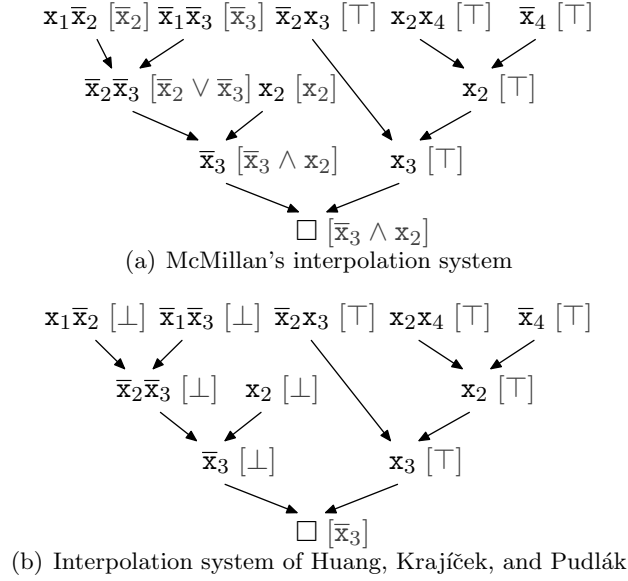
Figure 3.8: Refutation yielding different interpolants for different systems
