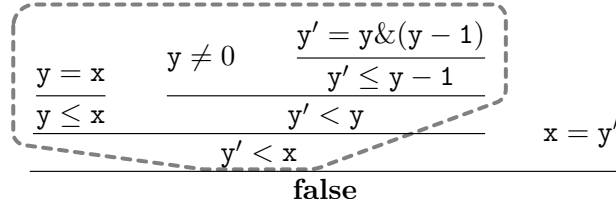
Figure 3.2: A proof consisting of local derivations
