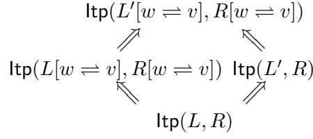
Figure 3.19: Combining labelling functions and proof transformations (Corollary 3.3.1)
