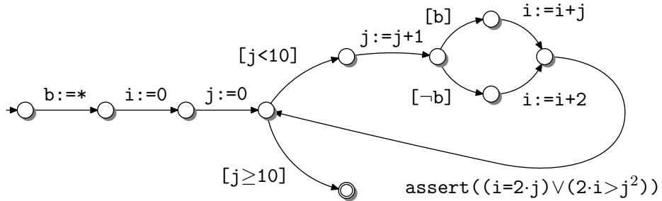
(c) A loop with a disjunctive invariant
