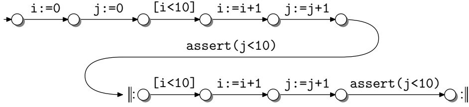
Figure 4.4: The path from Figure 4.2 annotated with loop information
