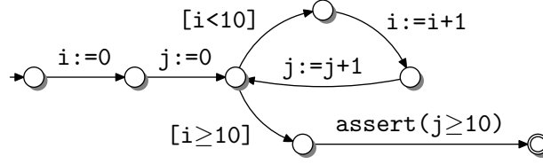
Figure 4.10: A safe program
