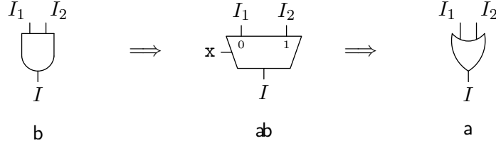
Figure 3.12: Combining partial interpolants: (I_1 \wedge I_2) \Rightarrow (\mathbf{x} \vee I_1) \wedge (I_2 \vee \neg \mathbf{x}) \Rightarrow (I_1 \vee I_2)
