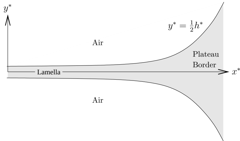
FIGURE 1. Schematic of the edge of a lamella.
