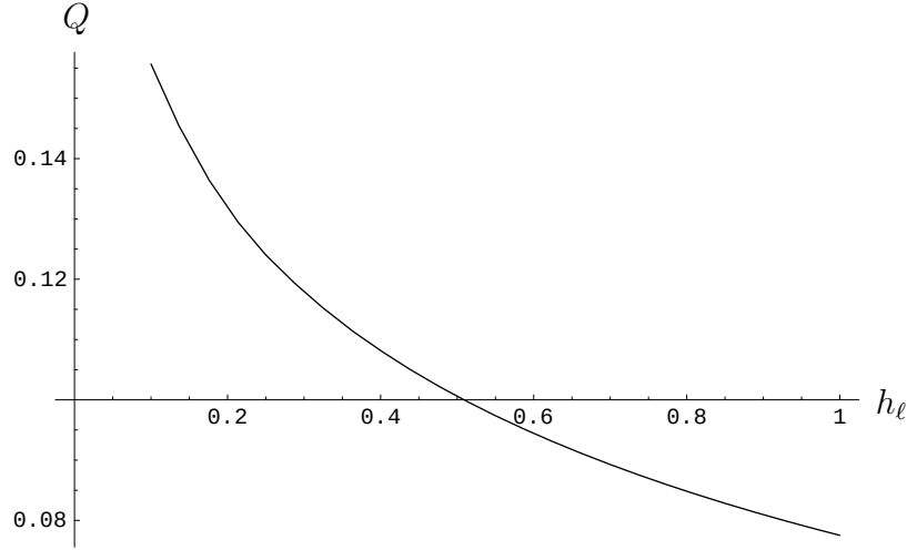
FIGURE 10. Graph showing Q as a function of h_\ell for \mathcal{P} = 0.5 , \mathcal{T} = 0.5 , C_I = 0.1 .
