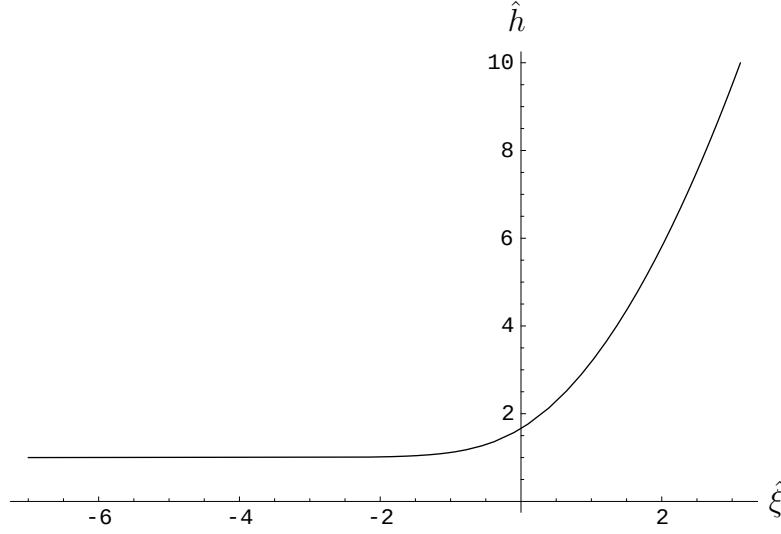
FIGURE 4. Transition region shape.
