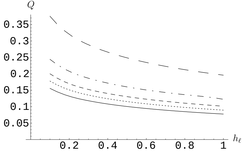
FIGURE 16. Graph showing how the flux varies with h_\ell , for \beta = 0 (solid line), 0.5 (dotted line), 1 (small-dashed line), 2 (dot-dashed line) and 5 (large-dashed line). The other parameters are taken to be \mathcal{P} = 0.5 , \mathcal{T} = 0.5 , and C_I = 0.1 .
