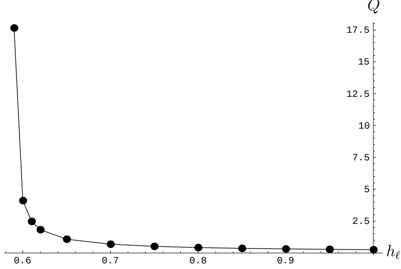
FIGURE 20. Graph showing Q against h_\ell for C_I = 0.5 , \mathcal{P} = 5 and \mathcal{T} = 5 .
