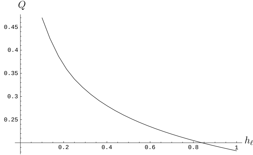
FIGURE 19. Graph showing Q against h_\ell for \mathcal{P}^* = 0.1 and \mathcal{T} = 1 and C_I = 0.1 .
