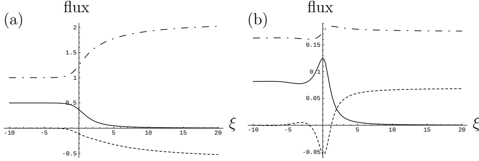
FIGURE 8. Surface convection (solid line), bulk convection (dot-dashed line) and bulk diffusion (dashed line), for (a) a monotonic and (b) a nonmonotonic solution.
