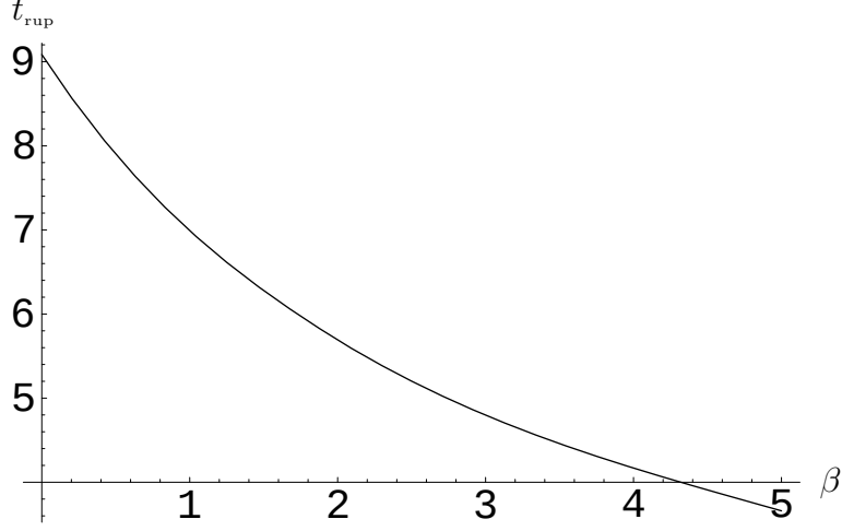
FIGURE 18. Graph showing how the rupture time varies with \beta . The other parameters are taken to be \mathcal{P} = 0.5 , \mathcal{T} = 0.5 , and C_I = 0.1 .
