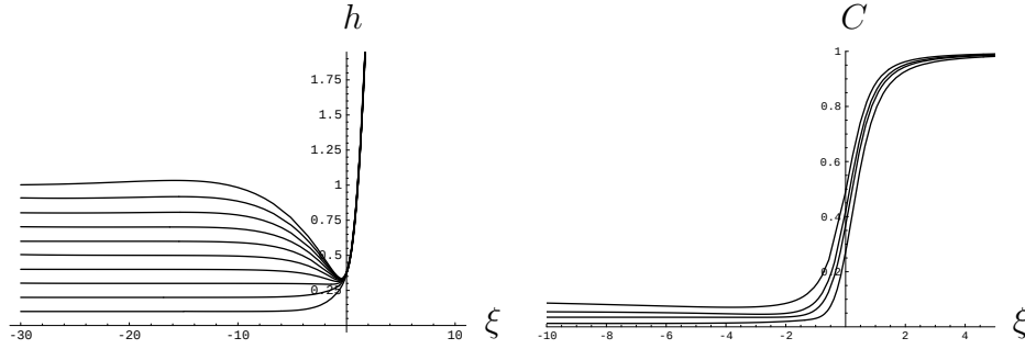
FIGURE 11. Transition region thickness and concentration for various values of h_\ell , with \mathcal{P} = 0.5 , \mathcal{T} = 0.5 , C_I = 0.1 .
