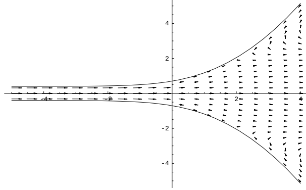
FIGURE 13. Velocity field for a solution where \mathcal{K} > 1 .
