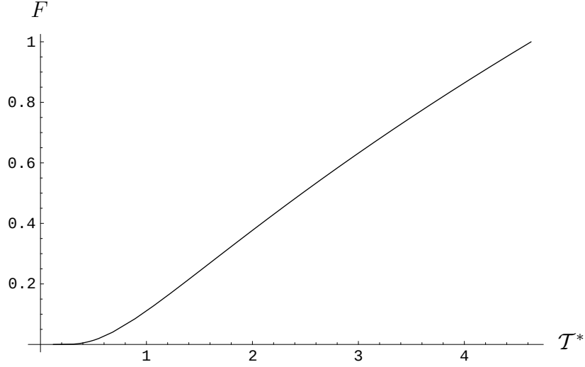
FIGURE 21. Graph showing the function F(T^*) defined in (6.11).
