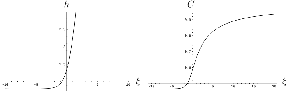
FIGURE 6. Results for thickness and concentration in a monotonic solution.
