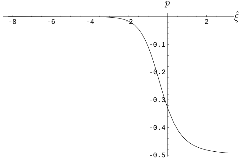
FIGURE 5. Transition region pressure profile.
