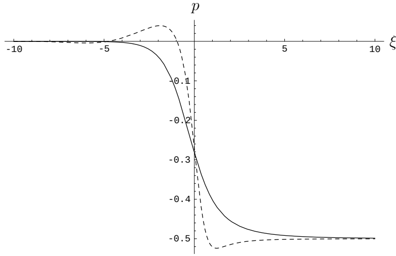
FIGURE 9. Pressure in a monotonic solution (solid) and a dimpled solution (dashed).
