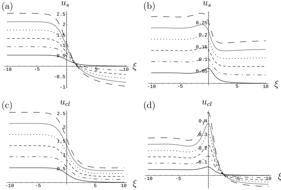
FIGURE 15. Graphs showing surface velocity u_s and centre-line velocity u_{cl} for the cases \mathcal{K} > 1 (figures (a) and (c)) and \mathcal{K} < 1 (figures (b) and (d)), with \beta = 0 (solid line), 0.2 (dot-dashed line), 0.4 (small-dashed line), 0.6 (wide-spaced dotted line), 0.8 (close-spaced dotted line) and 1.0 (large-dashed line).
