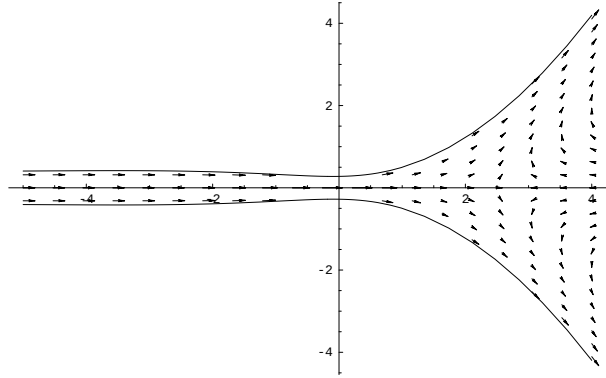
FIGURE 14. Velocity field for a solution where \mathcal{K} < 1 .
