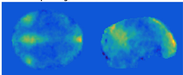
(c) Oulu Event2 ICA FIX retrained thr 20, PCA component 1, explaining 8.4867 % of the variance
