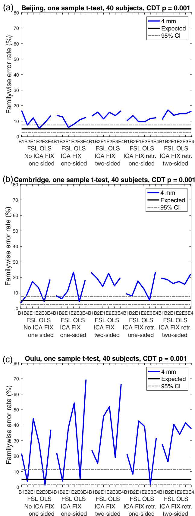
FIGURE 5 Results for FSL OLS one-sample t tests for cluster-wise inference using a CDT of p = .001 , for no ICA FIX, pretrained ICA FIX and retrained ICA FIX. (a) Results for Beijing data (b) results for Cambridge data (c) results for Oulu data. Results are only shown for 4 mm smoothing, as other smoothing levels would require retraining the ICA FIX classifier. The two-sided tests show a higher degree of false positives compared to the one-sided tests. This is explained by the fact that a two-sided test involves two tests at p = .025 , instead of one test at p = .05 , and parametric methods are relatively more inflated at more stringent significance thresholds (as the statistical assumptions are more critical for the tail of the null distribution) [Color figure can be viewed at wileyonlinelibrary.com ]
