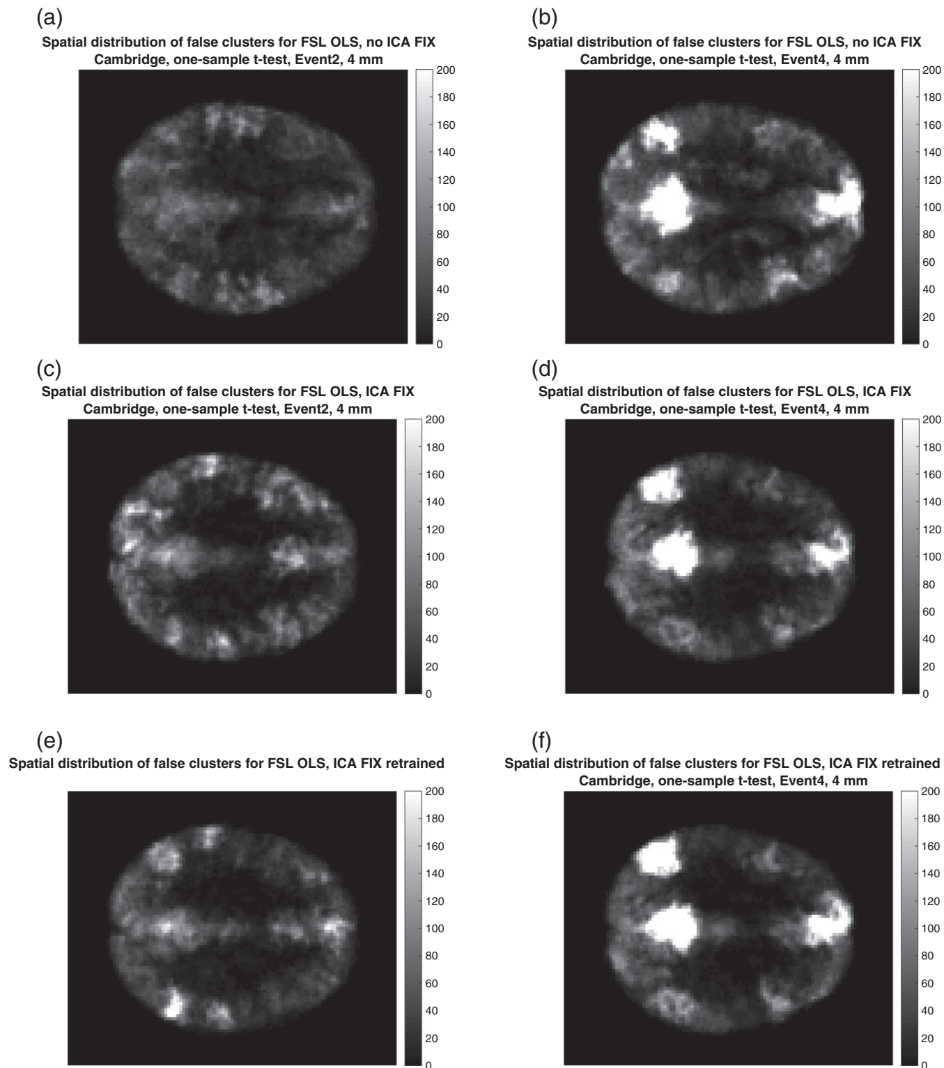
FIGURE 7 The maps show voxel-wise incidence of false clusters for the Cambridge data, for two of the six different first level designs (a,b) no ICA FIX (c,d) ICA FIX pretrained (e,f) ICA FIX retrained for Cambridge. Left: results for design E2, right: results for design E4. Image intensity is the number of times, out of 10,000 random analyses, a significant cluster occurred at a given voxel (CDT p = .01 ) for FSL OLS. Each analysis is a one-sample t test using 20 subjects. The maps represent axial slice 50 (MNI z coordinate = 26) for the MNI152 2 mm brain template used in FSL
