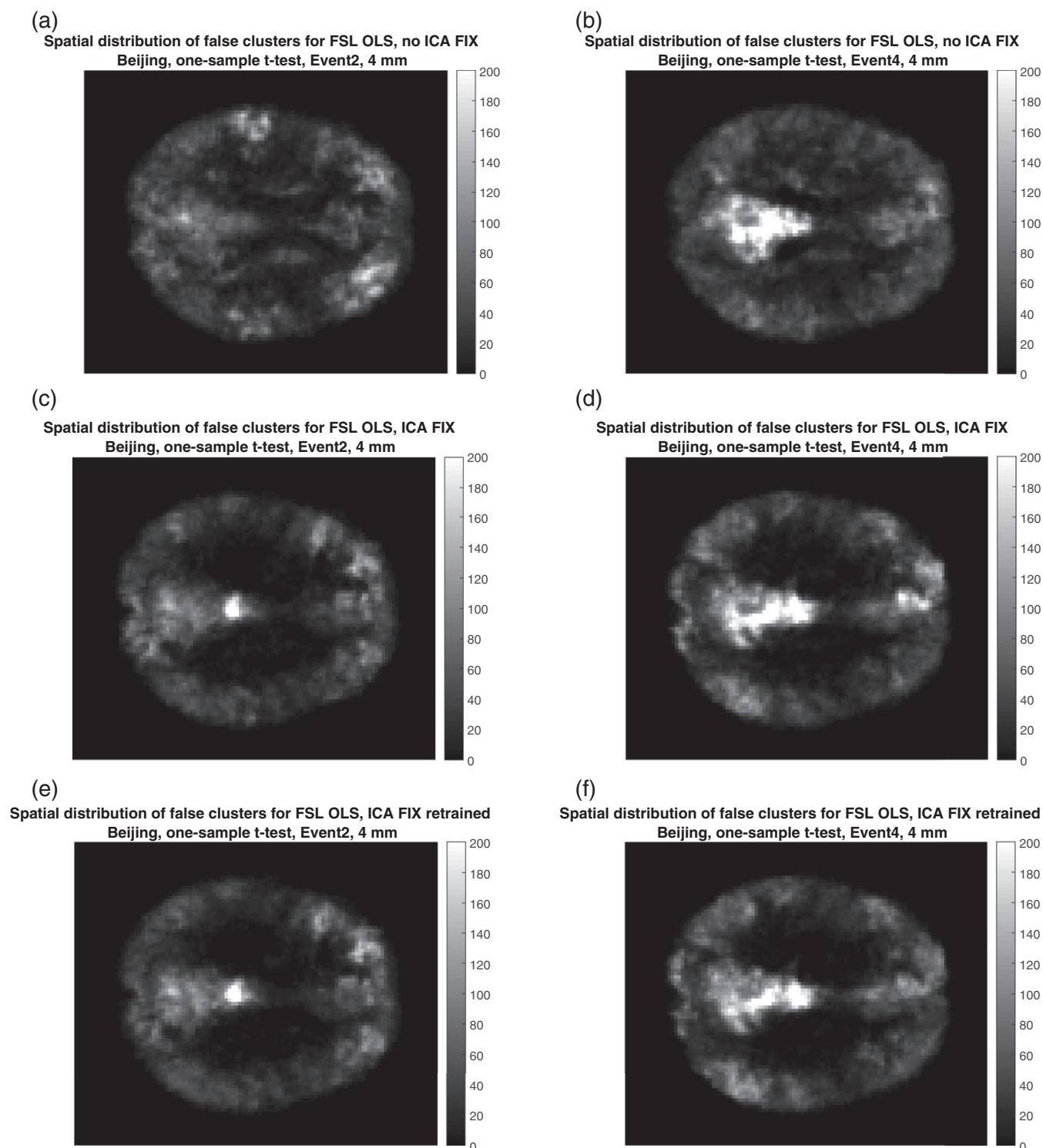
FIGURE 6 The maps show voxel-wise incidence of false clusters for the Beijing data, for two of the six different first level designs (a,b) no ICA FIX (c,d) ICA FIX pretrained (e,f) ICA FIX retrained for Beijing. Left: results for design E2, right: results for design E4. Image intensity is the number of times, out of 10,000 random analyses, a significant cluster occurred at a given voxel (CDT p = .01 ) for FSL OLS. Each analysis is a one-sample t test using 20 subjects. The maps represent axial slice 50 (MNI z coordinate = 26) for the MNI152 2 mm brain template used in FSL
